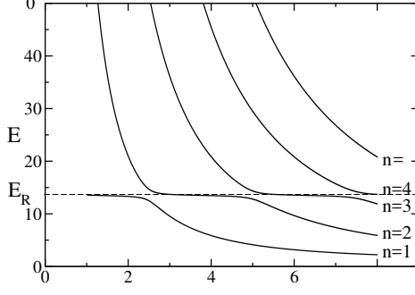
FIG. 18 Energy levels of an interacting two-particle system. In case of a resonance in this system, the energy levels exhibit the avoided level crossing (plateau) that allows to read off the resonance energy E_R directly.
