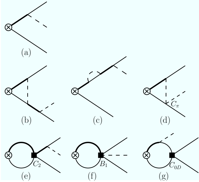
FIG. 14 LO (a) and NLO (b, ..., g) diagrams for the calculation of the X(3872) \rightarrow D^0 \bar{D}^0 \pi^0 decay width. The circled cross denotes an insertion of the X(3872) , the thin and thick solid lines represent the pseudoscalar and vector charm mesons, respectively, and the dashed lines denote the pions.
