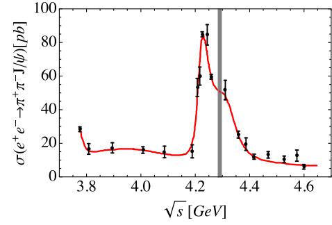
FIG. 5. The cross section of e^+e^- \rightarrow \pi^+\pi^- J/\psi for center-of-mass energies from 3.77 to 4.6 GeV (Ablikim et al. , 2017c). It shows a clear shoulder around the D_1\bar{D} threshold (marked by the vertical gray band) as predicted by Cleven, Wang et al. (2014). The solid red curve is from the analysis of BESIII (Ablikim et al. , 2017c). A comparison of these data with the BESIII scan data can be found in Gao, Shen, and Yuan (2017).
