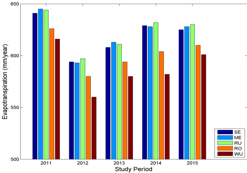
Figure 3.12. Annual sum of evapotranspiration (mmyear -1 ) for Eddy Covariance sites, namely, Selhausen (SE), Merzenhausen (ME), Selhausen-Ruraue (RU), Rollesbroich (RO) and Wuestebach (WU) for a period of 2011 through 2015, in the Rur catchment, Germany.
