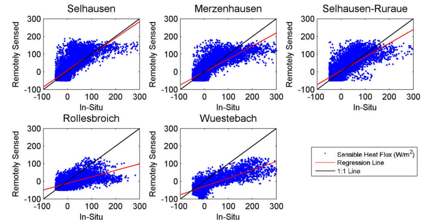
Figure 3.5. Scatter plots of hourly H_{EC} ( in situ ) and H_{EBM} (energy balance model) for the Eddy Covariance sites in the Rur catchment, Germany, for the years 2011-2015.
