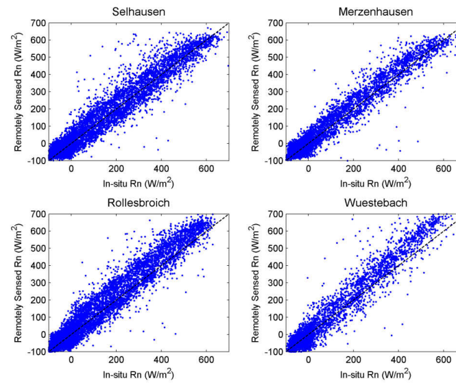
Figure 3.3. Scatter plots of hourly in situ and remotely sensed net radiation ( R_n ) for Eddy Covariance sites in the Rur catchment, Germany, for five years (2011-2015).
