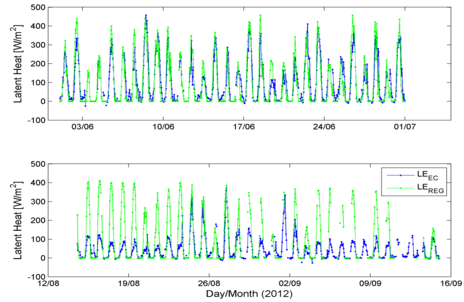
Figure 3.10. Temporal sequence of LE_{REG} and LE_{EC} during June 2012 (upper) and mid-August to mid-September 2012 (lower) at Merzenhausen.
