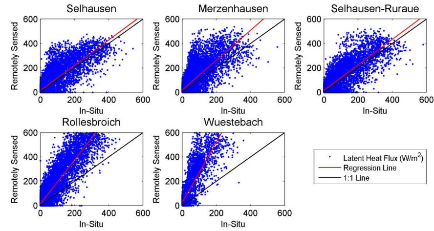
Figure 3.4. Scatter plots of hourly L_{EC} ( in situ ) and L_{EBM} (energy balance model) for the Eddy Covariance sites in the Rur catchment, Germany, for the years 2011-2015.
