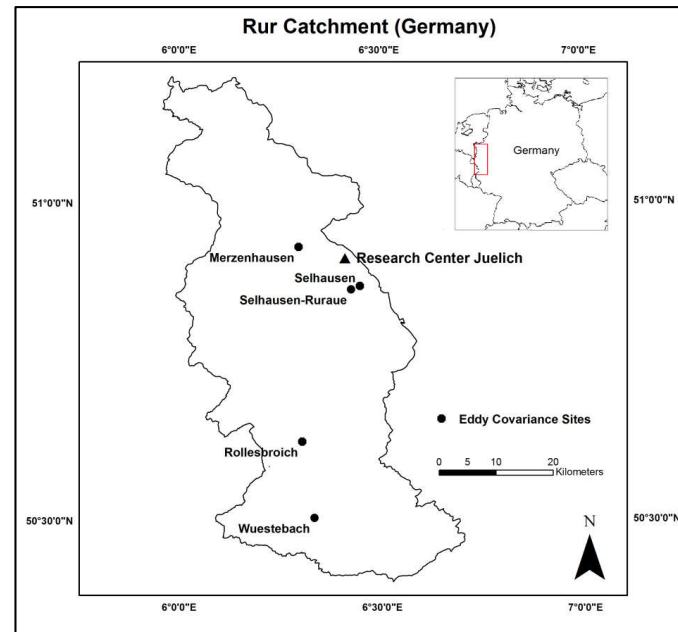
Figure 3.1. Rur Catchment, Germany, with Eddy Covariance sites.
