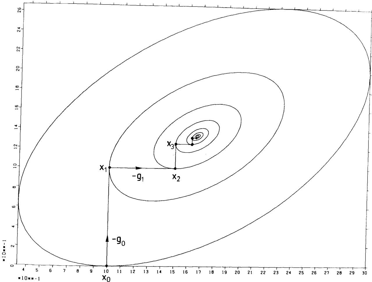
Fig. 5.1: Optimum gradient method for n=2 .
