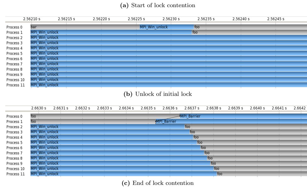
Figure 5.8.: Timeline view of the start and the end of a lock contention scenario. The execution time of the initial call to function foo() is skewed across the processes to ensure that process 0 acquires the lock first and the accesses of the remaining processes are queued. When process 0 releases the lock after the call to function bar() , process 1 completes its access and releases the lock again, yet process 0 does not provide further progress for the completion on the other processes. Starting the enclosing barrier synchronization, process 0 provides progress again, enabling completion of the pending lock epochs on the remaining processes.
