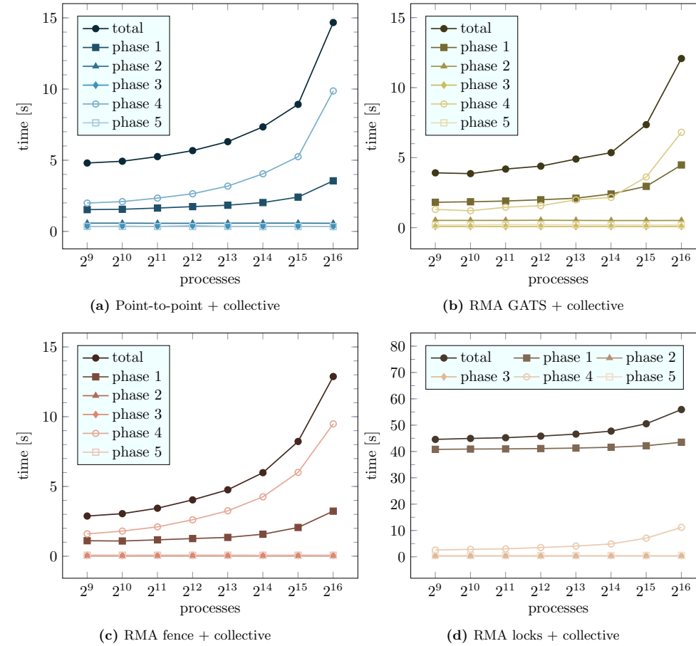
Figure 5.1.: Timings of the five analysis phases for measurements of the original SOR implementation using MPI point-to-point and collective communication, as well as modified implementations using various RMA synchronization schemes as replacements for the point-to-point communication. For the point-to-point and active-target synchronization scenarios the overall trend is similar with runtime mostly dominated by the cost accounting in the fourth phase. For the passive-target synchronization scenario the first phase with the detection of lock contention clearly dominates the overall runtime, however, its costs appear mostly scale-independent.
