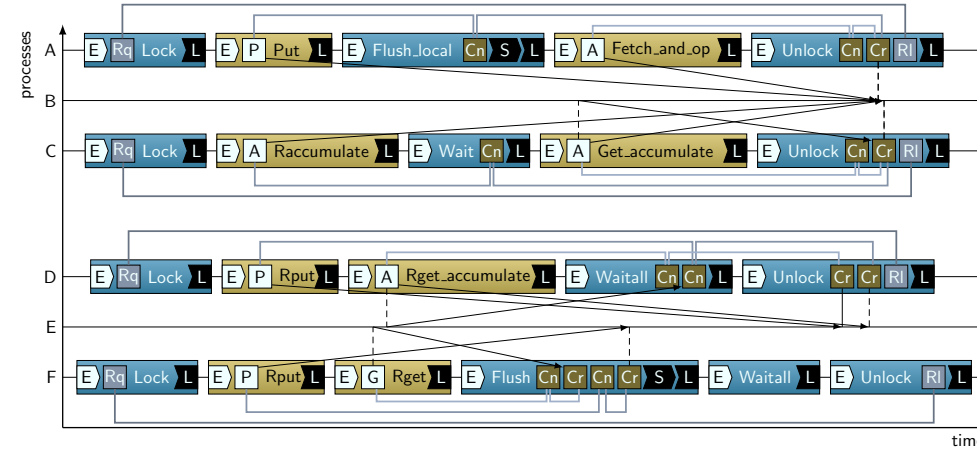
Figure 3.4: OTF2 event model for MPI passive-target synchronization. Locks model simultaneous access and exposure epochs. The release-lock event also marks remote completion of any operation. Flush calls, as introduced in MPI 3.0, enforce local completion of any operation. As always, get operations complete remotely when they complete locally and all other operations complete remotely at the release of the lock.
