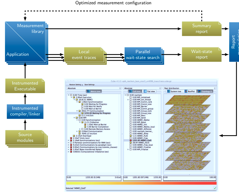
Figure 2.1.: The Scalasca workflow.
