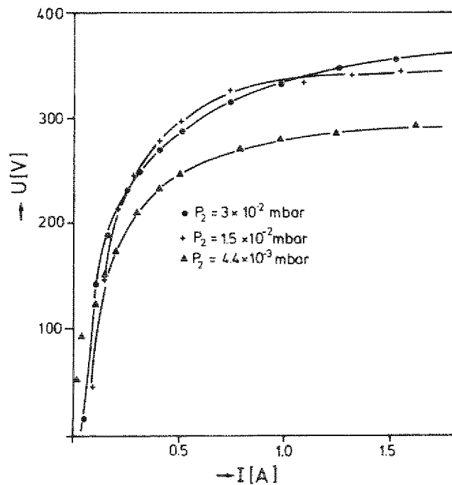
Fig. 12 Voltage ( U )- current ( I ) characteristics of RG discharges with a coil antenna in a NW 100 porthole at different pressures. With the exception of the steep increase at low current, the curves are almost independent on the rf power.
