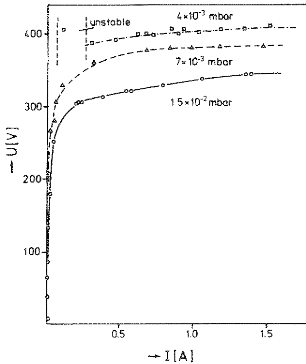
Fig. 11 Voltage ( U )- current ( I ) characteristics of RG discharges with the Lecher antenna at various pressures. With the exception of the steep increase at low current, the curves are almost independent on the rf power.
