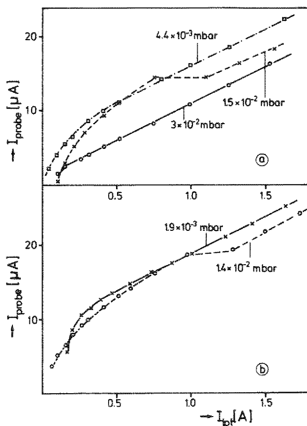
Fig. 15 Current to the auxiliary electrode ( I_{probe} ) versus total current of the discharge ( I_{tot} ) for a) coil anode in a NW 100 porthole b) coil anode in the center of the vessel
