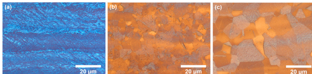
Figure 7. Microstructure of X60Mn18 steel (a) cold rolled; (b) recrystallization annealed at 800 °C for 2 min; (c) recrystallization annealed at 800 °C for 30 min.
