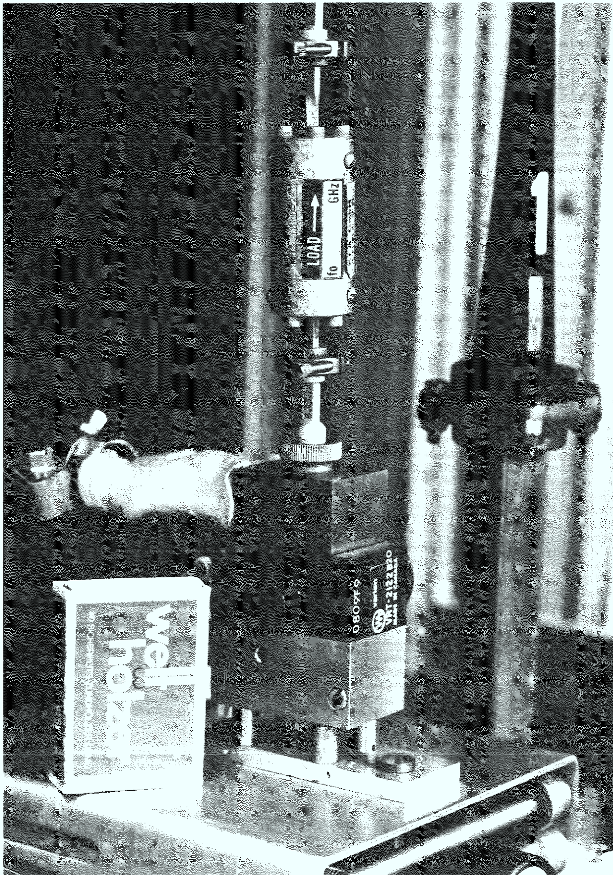
Fig. 7: Reflex klystron with water cooling unit used here as carrier wave generator.
