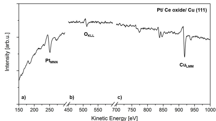
Fig. 6.3: First derivative of Auger electron spectrum for the Cu (111) crystal with the prepared platinum - cerium oxide combination on top: The energy ranges are selected for the identification of features belonging to a) platinum, b) oxygen and c) copper.
