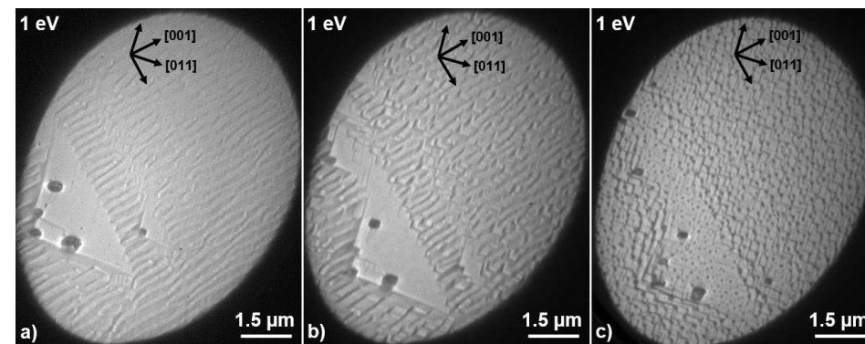
Fig. 3.17: Ceria growth at 530 °C on Cu (100) observed with LEEM: a) start, b) after 5 min, c) after 15 min.
