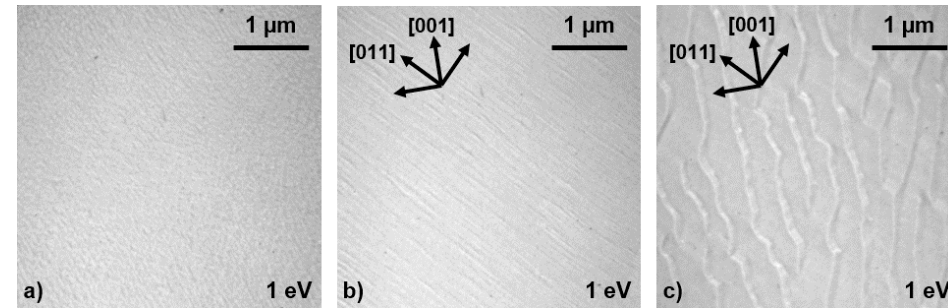
Fig. 3.16: LEEM images of Cu (100) substrate preparation: a) after \text{Ar}^+ -sputtering, b) heated to 600 °C, c) at 600 °C and in 5 \times 10^{-7} mbar \text{O}_2 .
