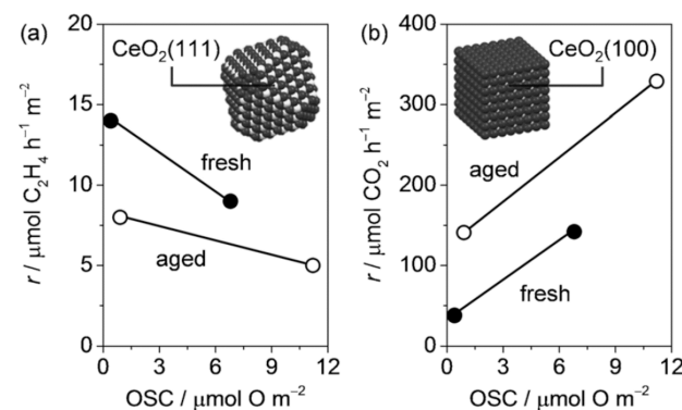
Fig. 1.5: \text{CeO}_2 reaction rates as a function of OSC: a) \text{C}_2\text{H}_2 hydrogenation with octahedron-like nanoparticles, b) CO oxidation with nanocubes, from [41].
