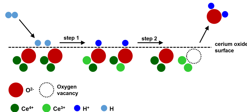
Fig. 4.1: An H 2 molecule adsorbs on the cerium oxide surface, dissociates, forms hydroxyls on the surface and reduces Ce 4+ to Ce 3+ . The surface hydroxyls diffuse on the cerium oxide surface and interact to produce H 2 O, which desorbs and leaves behind an oxygen vacancy. The figure follows the example in [108].
