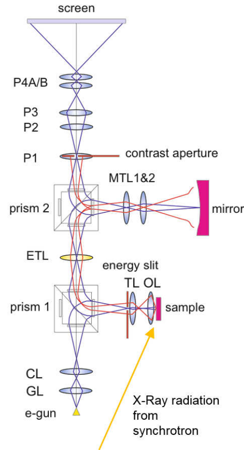
Fig. 2.2: Schematic diagram of the electron path through the LEEM/PEEM instrument with aberration correction (blue lines indicate the field rays and red lines the axial rays), adapted from [56].
