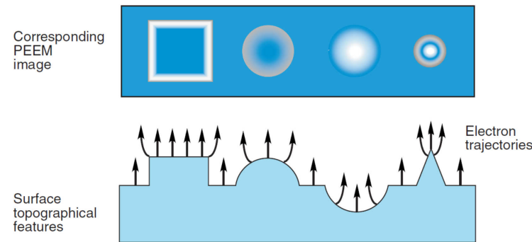
Fig. 2.5: Topological contrast in PEEM imaging, caused by topology induced electrostatic field distortions, from [74].
