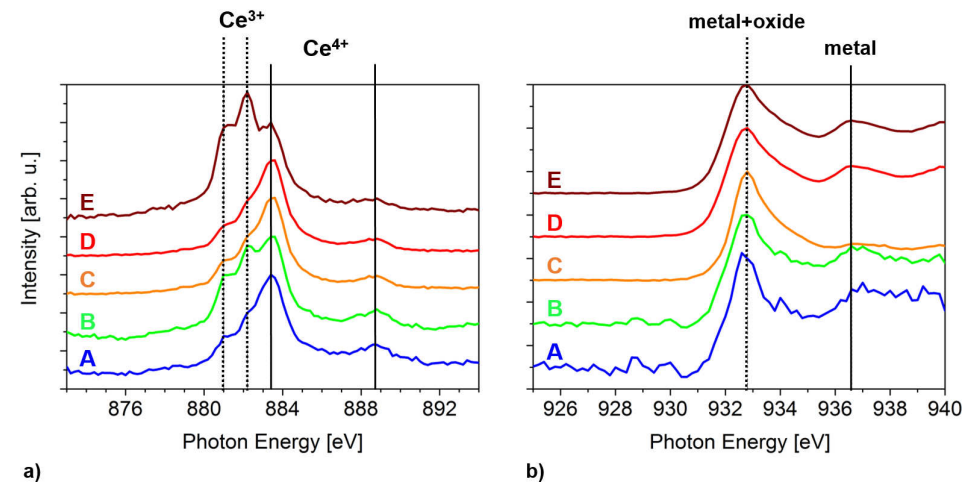
Fig. 7.4: \mu -XAS of the regions indicated in Fig. 7.3: a) Ce M_5 edge, b) Cu L_3 edge.
