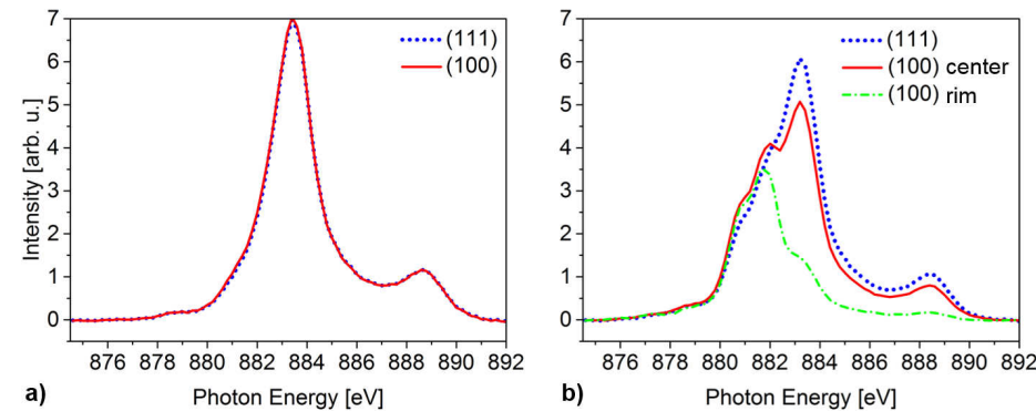
Fig. 5.5: Ce M 5 XAS of (111) and (100) islands market in 5.4 a) after growth, b) After Ce evaporation in vacuum at room temperature, followed by annealing 600 °C.
