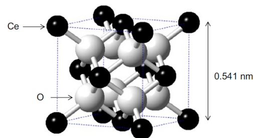
Fig. 1.2: Unit cell of CeO_2 fluorite structure, from [7].
