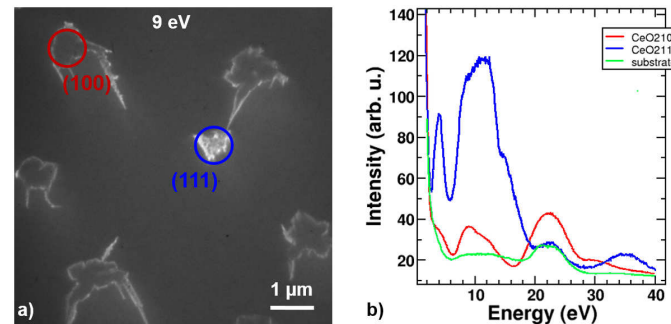
Fig. 3.8: Ceria island reflectivity in LEEM: a) LEEM image of (111) and (100) ceria islands showing a difference in contrast, b) IV-LEEM curves: Intensities of the Cu (111) substrate, the ceria (111) and (100) surfaces over the LEEM start energy, from [87].
