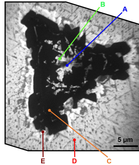
Fig. 7.3: a) UV-PEEM image of ceria triangle structure, indicating the regions for the \mu -XAS spectra in Fig. 7.4.
