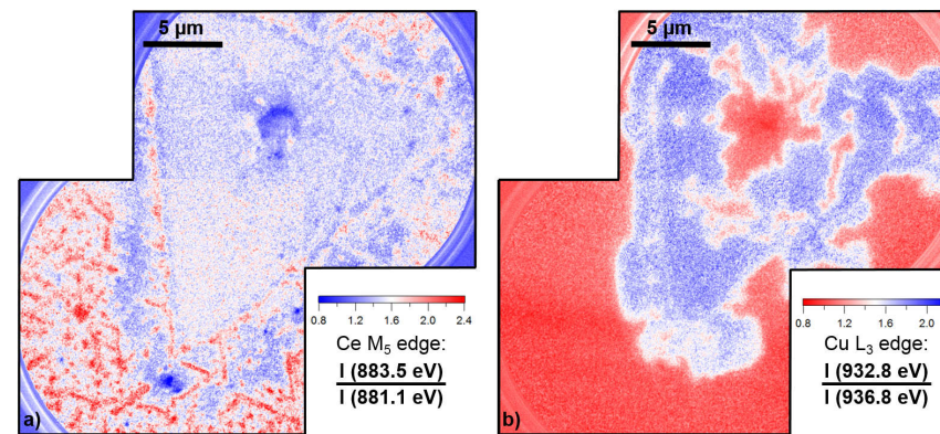
Fig. 7.5: a) Division of X-PEEM images recorded at the Ce M 5 peaks at 883.5 eV and 881.1 eV, b) Division of X-PEEM images recorded at the Cu L 3 peaks at 932.8 eV and 936.8 eV, also in publication [123].
