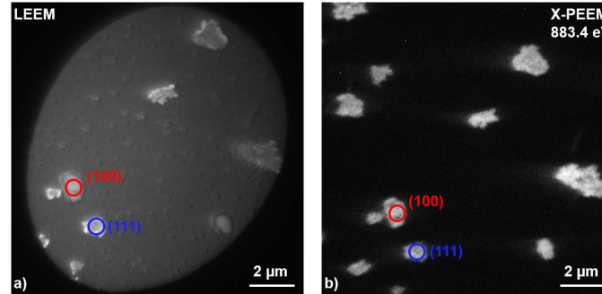
Fig. 4.6: a) LEEM image of ceria (111) and (100) islands after growth, b) X-PEEM image of islands in a) imaged at characteristic energy for Ce 4+ .
