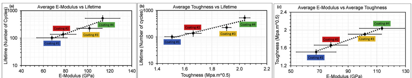
Fig. 11. Dependence of thermal shock lifetime on average E-modulus (a) and average Toughness (b). The relationship between Toughness and E-modulus (c) is also shown.
