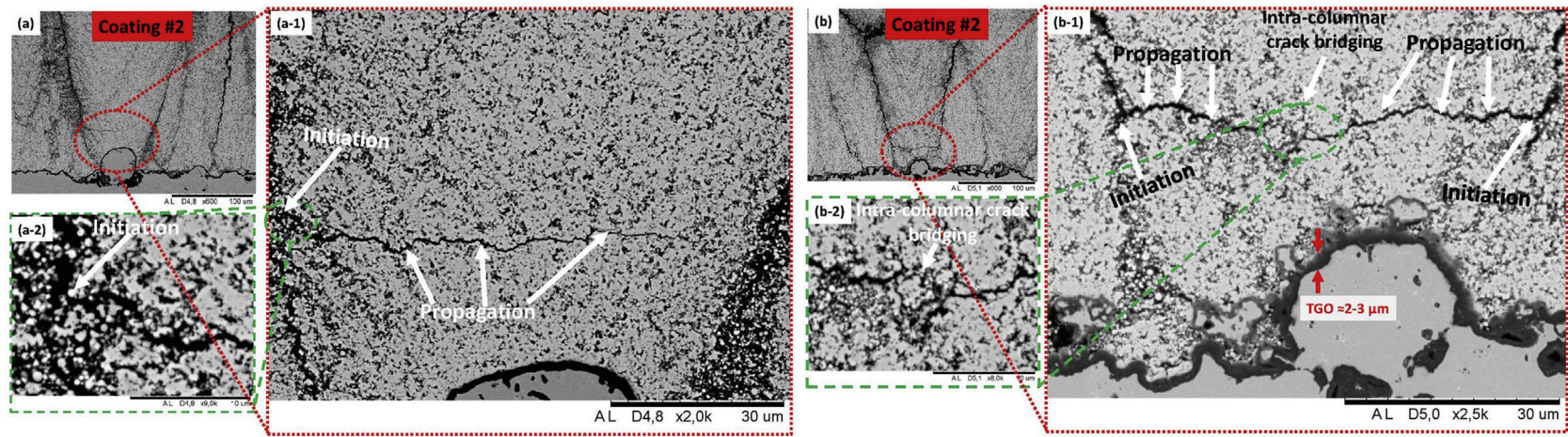
Fig. 13. Crack initiation and propagation in Coating #2, (a, a-1 & a-2) showing a crack initiating at the inter-columnar space and propagating towards the next nearest inter-columnar space; (b, b-1 & b-2) showing the crack initiating at the two neighboring inter-columnar spaces and bridging within the column (intra-columnar crack bridging).
