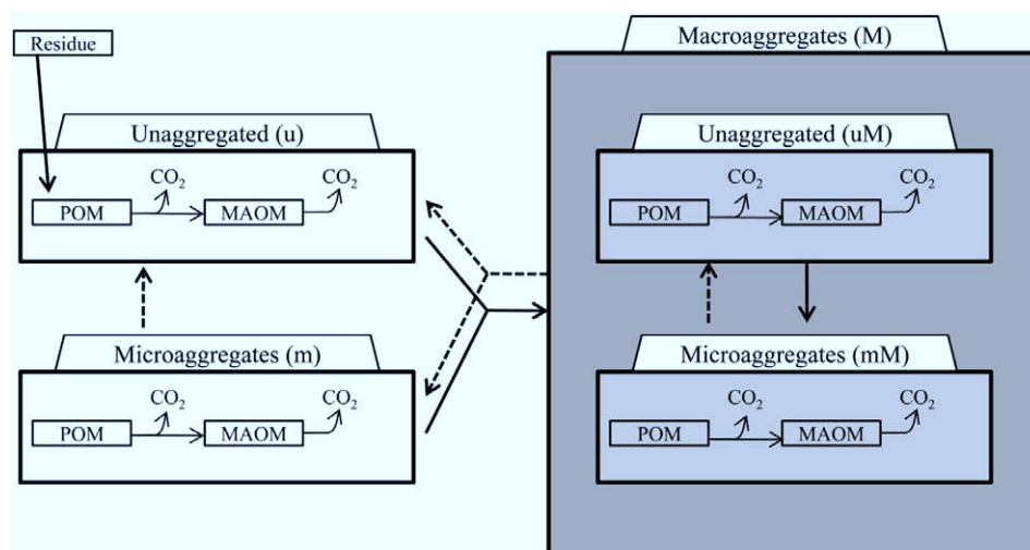
Figure 4: Conceptual multipool model of soil aggregate dynamics coupled with soil organic matter dynamics. POM: particulate organic matter, MAOM: mineral associated organic matter (Reprinted from Ecological Modelling, Vol. 263, M. Segoli, S. De Gryze, F. Dou, J. Lee, W. M. Post, K. Denef, J. Six, AggModel: A soil organic matter model with measurable pools for use in incubation studies, 1–9, Copyright (2013), with permission from Elsevier.).
