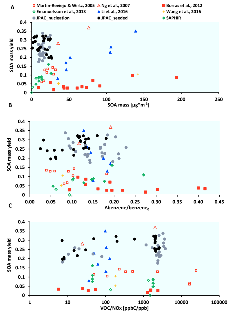
Figure 7.4: SOA mass yield as a function of SOA mass (A), relative benzene consumption (B) and initial VOC/NO x (C) for all studies on SOA formation from photo-oxidation of benzene. For Martin-Reviejo and Wirtz (2005) the overall yield is shown. For Wang et al. (2016) only endpoints of the SOA mass yield are given in the original publication. JPAC data are derived from SOA mass concentrations corrected for wall loss of SOA precursors.
