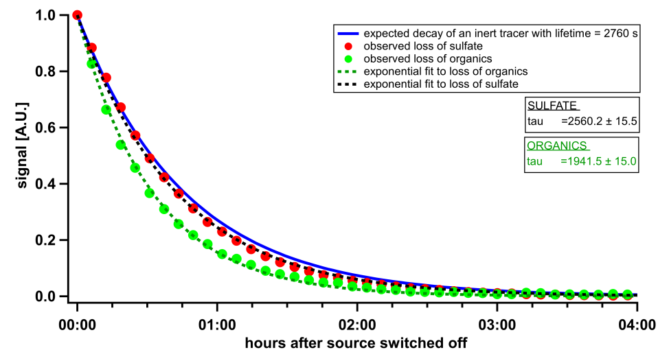
Figure 6.1: The blue line shows the expected exponential decay of an inert tracer with a chamber residence time of 2760 s (=46 min). The red (green) circles depict the sulphate (organics) mass concentration measured by AMS and normalised to 1. The dashed lines are exponential least squares fits to the observations and the resulting lifetime ( \tau ) is given in seconds and the respective uncertainty of the fit within the boxes.
