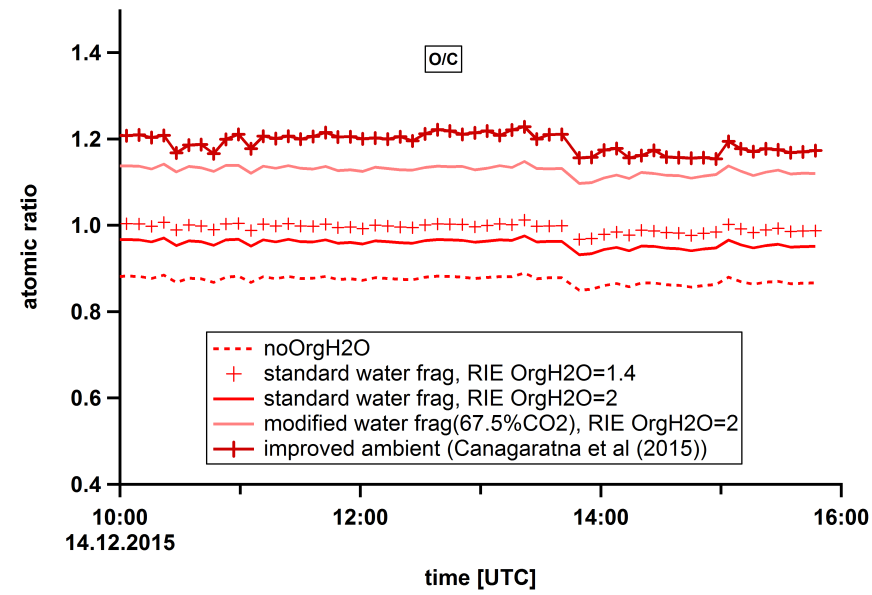
Figure A.11.1: Influence of enhanced water fragmentation on O/C ratio
