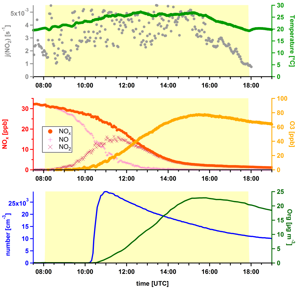
Figure B.16: Overview of ASOA production from benzene-d 6 at high NO x . The yellow shaded area indicates the time when the shutter system of the chamber was open.
