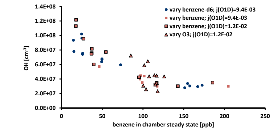
Figure B.8: OH concentration determined from all benzene experiments without \text{NO}_x addition as a function of steady state benzene concentration in the chamber. The amount of benzene (red squares) or benzene-d6 (blue circles) in the chamber is directly controlling the OH concentration as long as the OH production rate is not changed. Since the increase of j(\text{O}^1\text{D}) (red squares with black frame) did not significantly increase the OH production rate, this was only achieved by variation of the ozone concentration (red triangles).
