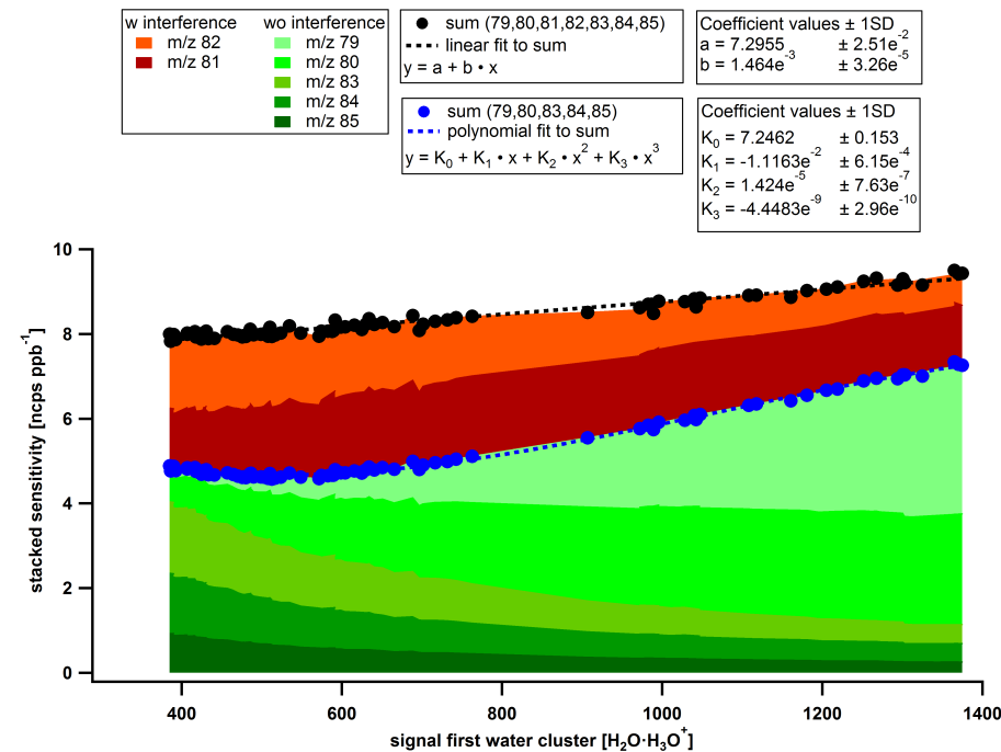
Figure A.3.1: Stacked contributions of the sensitivity of ions to the benzene-d6 total signal. Ions depicted in red colours suffer from interferences with ions originating from monoterpenes and cannot be used for benzene-d6 measurements. A linear function was fitted to the total sensitivity of all contributing ions in order to determine the total dependence on humidity (black data points and black dashed line). A polynomial function including 4 terms was fitted to the sum of sensitivities from ions that are free of interferences (black data points and black dashed line).
