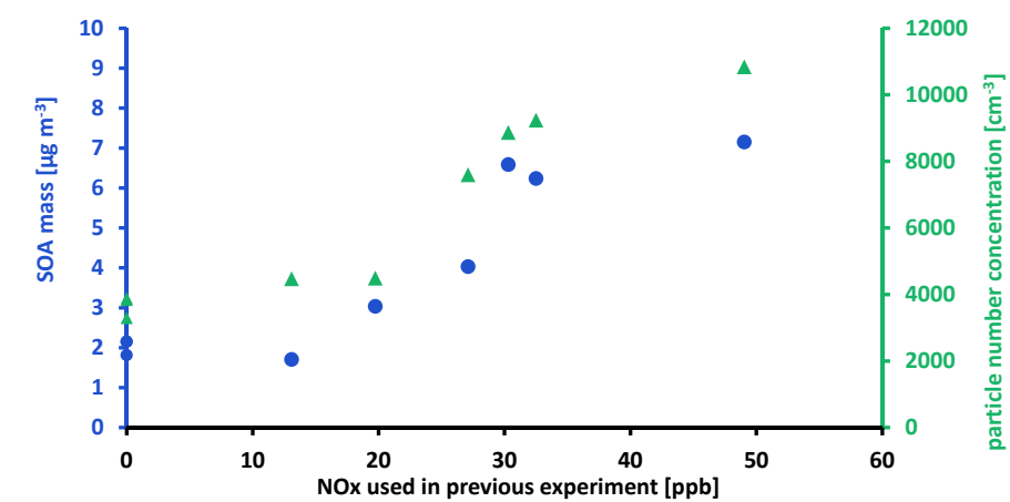
Figure B.11: SOA mass concentration (blue circles) and particle number concentration (green triangles) as function of \text{NO}_x used in preceding experiment.
