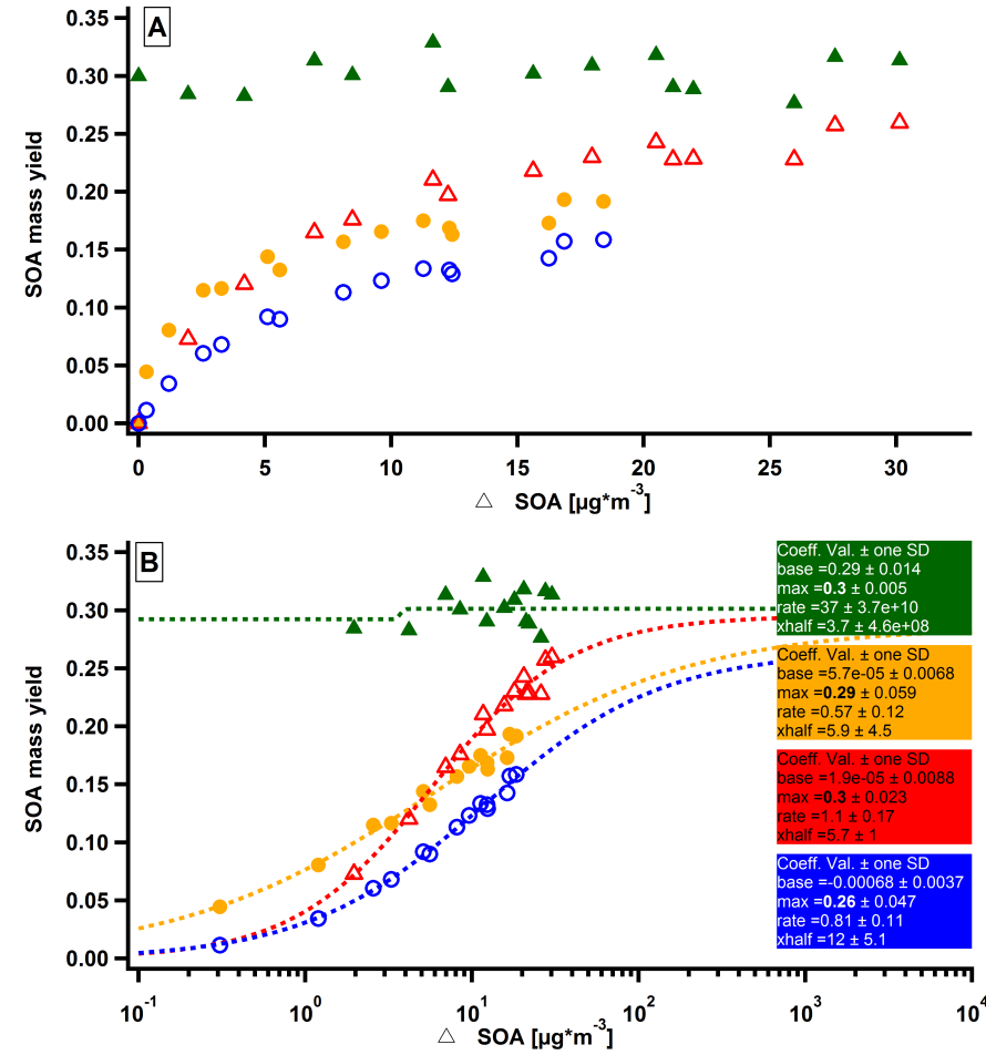
Figure 4.2: Schematic illustration of SOA mass yield concept 2: SOA mass yield as a function of SOA mass (Panel A: linear x-axis; Panel B: logarithmic x-axis). The green filled triangles represent a constant yield independent of the particle mass present in the chamber following the concept of Grosjean and Seinfeld (1989). The orange filled circles show an increasing yield according to Odum et al. (1996). Red hollow triangles and blue hollow circles represent both concepts as mentioned before but shifted by a positive offset on the x-axis. All curves result in the same yield for SOA \rightarrow \infty as can be seen from the Hill Curve least squares fit maximum values (Emanuelsson et al., 2013) in panel B. The proposed behaviour of the SOA mass yield being a function of the SOA mass formed (orange filled circles) can similarly be observed for data that show a linear dependence of SOA formed per amount of VOC reacted but with offset on the x-axis (red hollow triangles) and by a curve with combined effects of mass dependence and offset (blue hollow circles).
