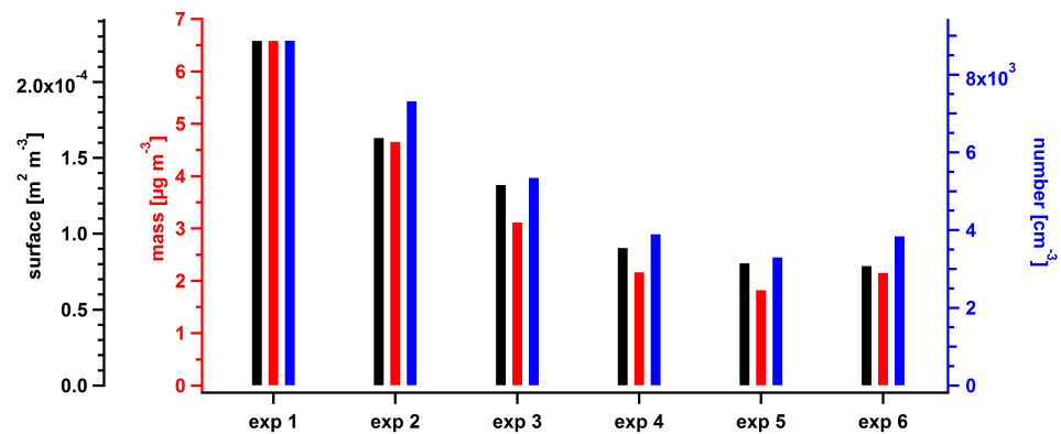
Figure B.12: SOA mass concentration (red bars), particle number concentration (blue bars), and particle surface concentration (black bars) for 6 \text{NO}_x -free experiments following a \text{NO}_x experiment with initial \text{NO}_x of 107 ppb.
