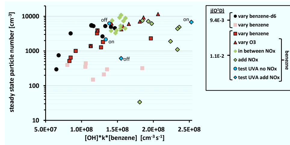
Figure 6.18: Steady state particle number concentration as a function of benzene reaction rate.
