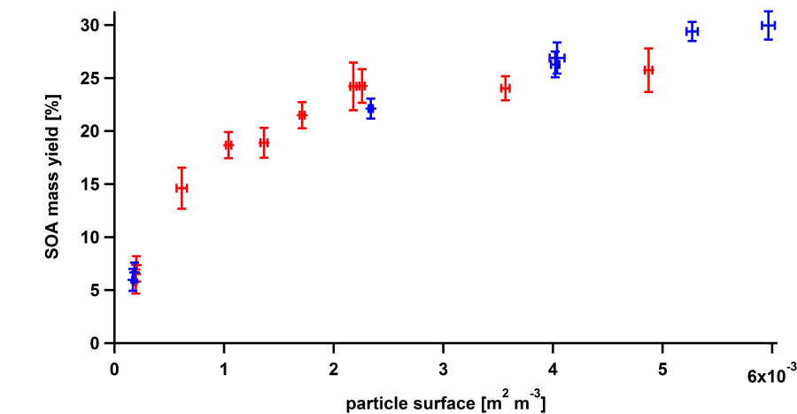
Figure B.7: Uncorrected SOA mass yield of benzene as function of particle surface for chamber 1 (red) and chamber 3 (blue) determined from experiments at constant oxidation conditions and varying seed aerosol surface. Error bars for both data sets give the experimental variation as the standard deviation for each steady state where the data were averaged. Note that the absolute uncertainty of yields is estimated to be 30 %.
