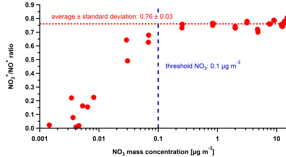
Figure 2.5: \text{NO}_2^+/\text{NO}^+ ratio as a function of total \text{NO}_3 mass. For this calibration, an average R_{calib} of 0.76 was obtained. Below a total nitrate mass concentration of 0.1 \mu\text{g m}^{-3} , the \text{NO}_2^+/\text{NO}^+ ratio drops significantly and this mass concentration is constantly set as the threshold for organic nitrate determination. Data shown in this figure were acquired by Avtandil Turdziladze.
