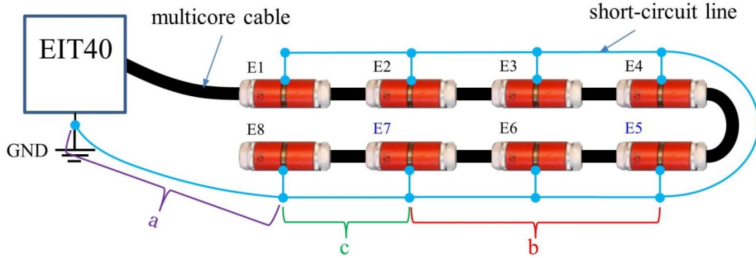
Figure 4.2: Pole-pole calibration measurement for electrode chain with 8 ring electrodes and 25 m long multi-core cable: one example for the configuration [5 7] with the segments a , b , and c of the short-circuit line related to the additive inductances.
