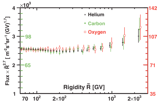
FIG. 4. The rigidity dependence of the helium (left black axis), carbon (left green axis), and oxygen (right red axis) fluxes. For clarity, horizontal positions of the helium and oxygen data points above 400 GV are displaced with respect to the carbon. As seen, above 60 GV the three fluxes have identical rigidity dependence.
