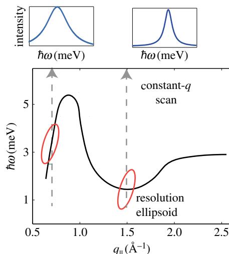
Figure 10. Lipid dispersion and instrumental resolution. The lipid dispersion is drawn schematically. During a constant- q_{||} scan, the resolution ellipsoid is moved across the dispersion to detect the corresponding excitations. The smallest peak width in the spectra is observed when the dispersion is cut perpendicular, in the minimum of the dispersion relation.
