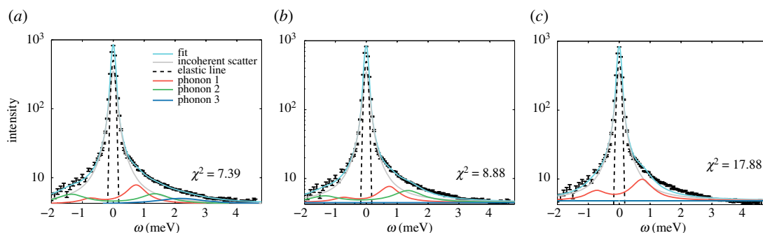
Figure 9. Inelastic scans measured at a q_{||} -value of q_{||} = 1.37 \text{ \AA}^{-1} . The spectra can be fitted using different models: all models contain an elastic line, centred at energy transfer 0 (described by a Gaussian peak profile) and a Lorentzian peak also centred at '0' to account for the incoherent scattering. (a) A fit including three phonon excitations, which shows a good agreement with the measured data. It was also attempted to fit the spectra with two excitations, and one excitation only (c). By comparing the resulting \chi^2 -values, the fit with three phonons provides the best model to the data. This is also supported by the results of an F -test in table 3.
