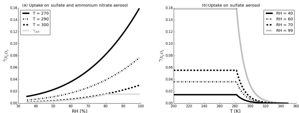
Figure 1. (a) \text{N}_2\text{O}_5 reaction probability dependence on relative humidity for sulfate (black) and nitrate (grey) aerosol. For sulfate aerosol, three temperatures are shown. (b) \text{N}_2\text{O}_5 reaction probability temperature dependence on sulfate aerosol for four relative humidities. Parameterizations are from Evans and Jacob (2005) and Davis et al. (2008); see text.
