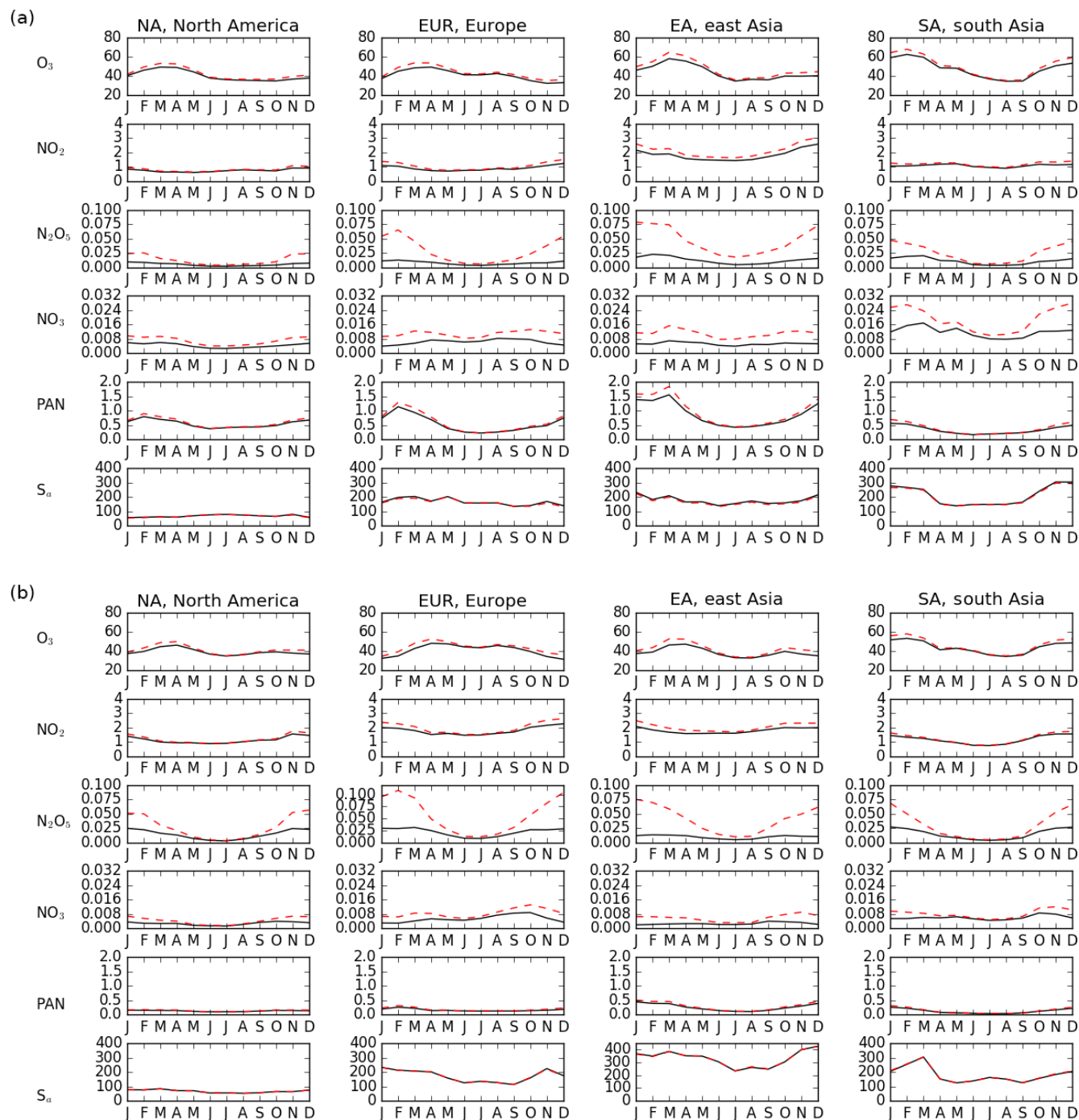
Figure 5. Changes in near-surface O 3 , NO 2 , N 2 O 5 , NO 3 , PAN, and S a for the base case (solid black line) and noN 2 O 5 case (dashed red line) for EMEP (a) and ECHAM-HAMMOZ (b). Plots show monthly gas-phase mixing ratios in ppbv and surface area density in μm 2 cm −3 for different regions as defined above.
