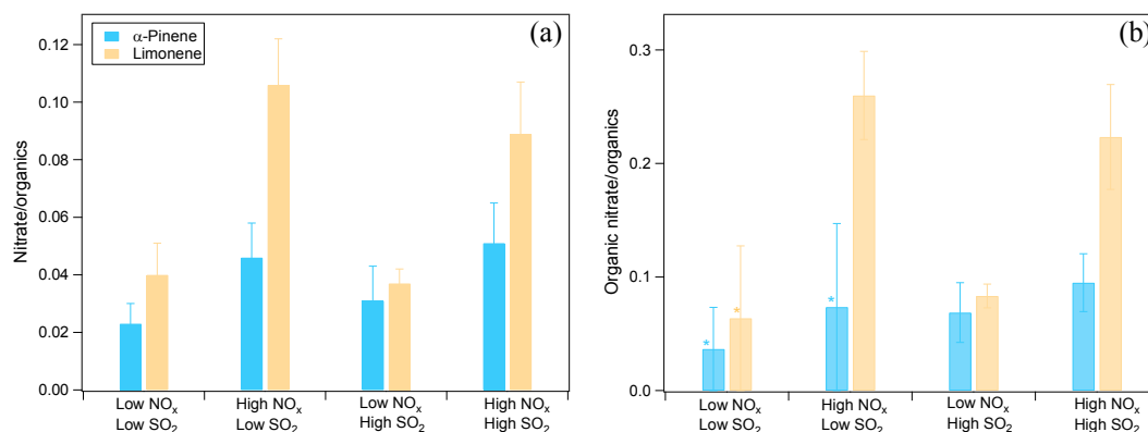
Figure 4. (a) The ratio of nitrate mass concentration to organics mass in different NO x and SO 2 conditions. The average ratios of nitrate to organics during the reaction are shown and error bars indicate the standard deviations. (b) The fraction of organic nitrate to total organics in different NO x and SO 2 conditions calculated using a molecular weight of 200 g mol -1 for organic nitrate. The average fractions during the reaction are shown and error bars indicate the standard deviations. In panel (b), * indicates the experiments where the ratios of NO 2 + to NO + were too noisy to derive a reliable fraction of organic nitrate. For these experiments, 50 % of total nitrate was assumed to be organic nitrate and the error bars show the range when 0 to 100 % of nitrate is assumed to be organic nitrate.
