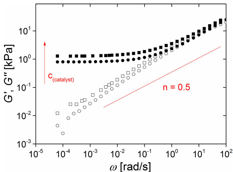
Fig 3. Reducing the catalyst concentration decreases elasticity of elastomers. Frequency dependence of storage ( G' , solid symbols) and loss modules ( G'' , open symbols) of neat silicone networks (system 1) prepared at r = 0.71 and measured at 1% strain. Squares: 0.5 ppm catalyst; circles: 0.37 ppm catalyst. Red line: power law expected for a critical gel (see discussion ). Raw data can be found in S3 Dataset .
