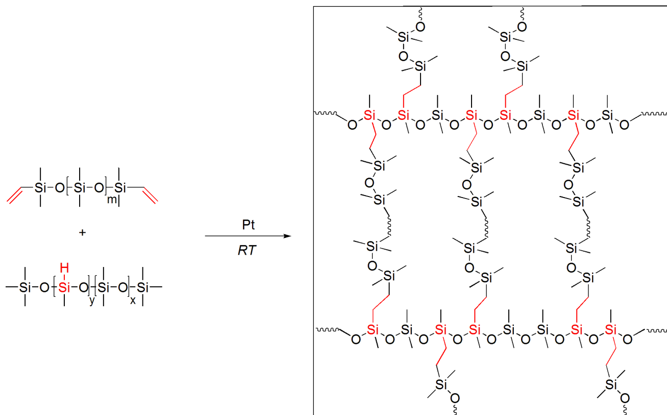
Fig 1. Schematic diagram of the PDMS system for preparation of ultrasoft PDMS elastomers; m \approx 2090 ; x \approx 700 , y \approx 51 , calculated from 5–7 mol% of hydrosilane group. Right hand side shows a detail of the PDMS network.
