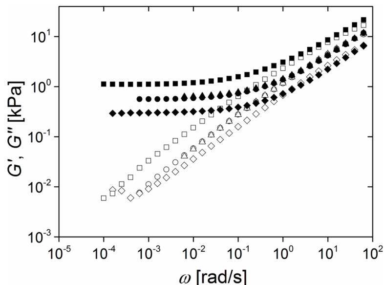
Fig 6. Change of rheological properties due to addition of inert filler polymers. Frequency dependence of the storage ( G' , solid symbols) and loss modules ( G'' , open symbols) at a strain of 1%. All samples: r = 0.71 and 0.5 ppm catalyst; Squares: neat system; Circles: 25% (v/v) of 139 kg/mol inert PDMS added; Triangles: 25% (v/v) of 68 kg/mol inert PDMS added; Diamonds: 25% (v/v) of 28 kg/mol inert PDMS added. Raw data can be found in S7 Dataset .
