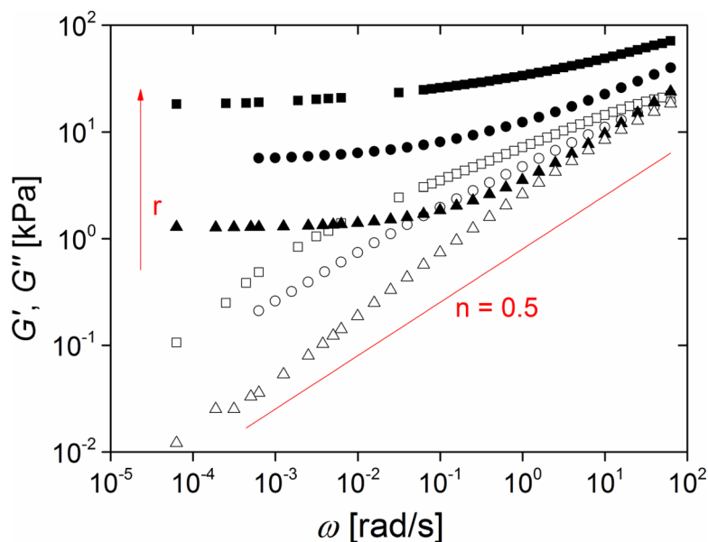
Fig 4. The stoichiometric ratio controls viscoelastic response. Frequency dependence of storage ( G' , solid symbols) and loss modules ( G'' , open symbols); squares stoichiometric ratio r = 1.28 ; circles: r = 1.00 ; triangles: r = 0.71 . Red line: power law expected for a critical gel (see discussion ). Raw data can be found in S4 Dataset .
