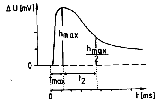
Fig. 23a: Schematic drawing of the ERG (electroretinogram) and the parameters which were measured: h_{max} , t_{max} , t_2
