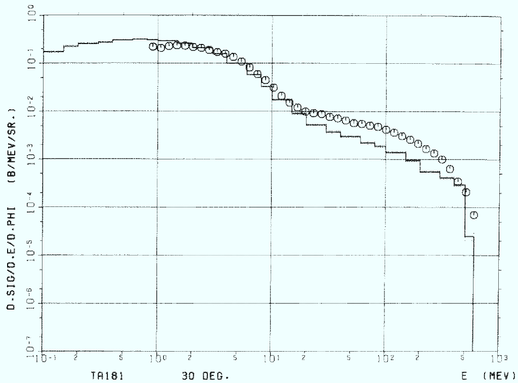
Figure 3a Tantalum (Ta-181) 30^\circ
