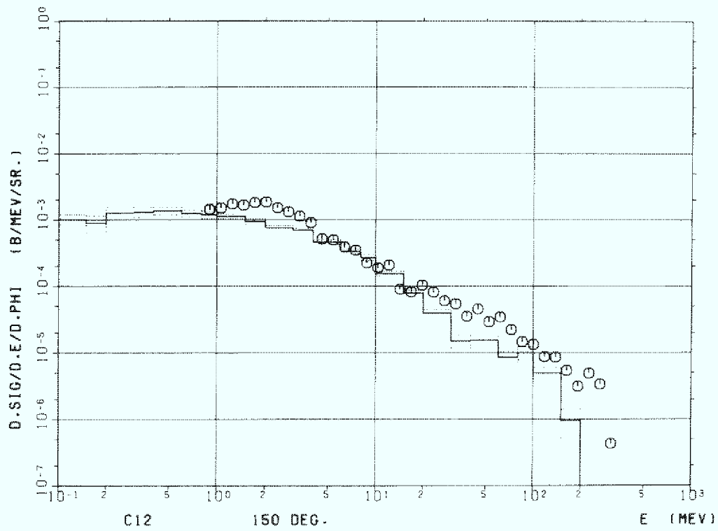
Figure 8c Carbon (C-12) 150°
