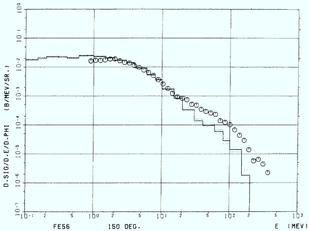
Figure 6c Iron (Fe-56) 150°
