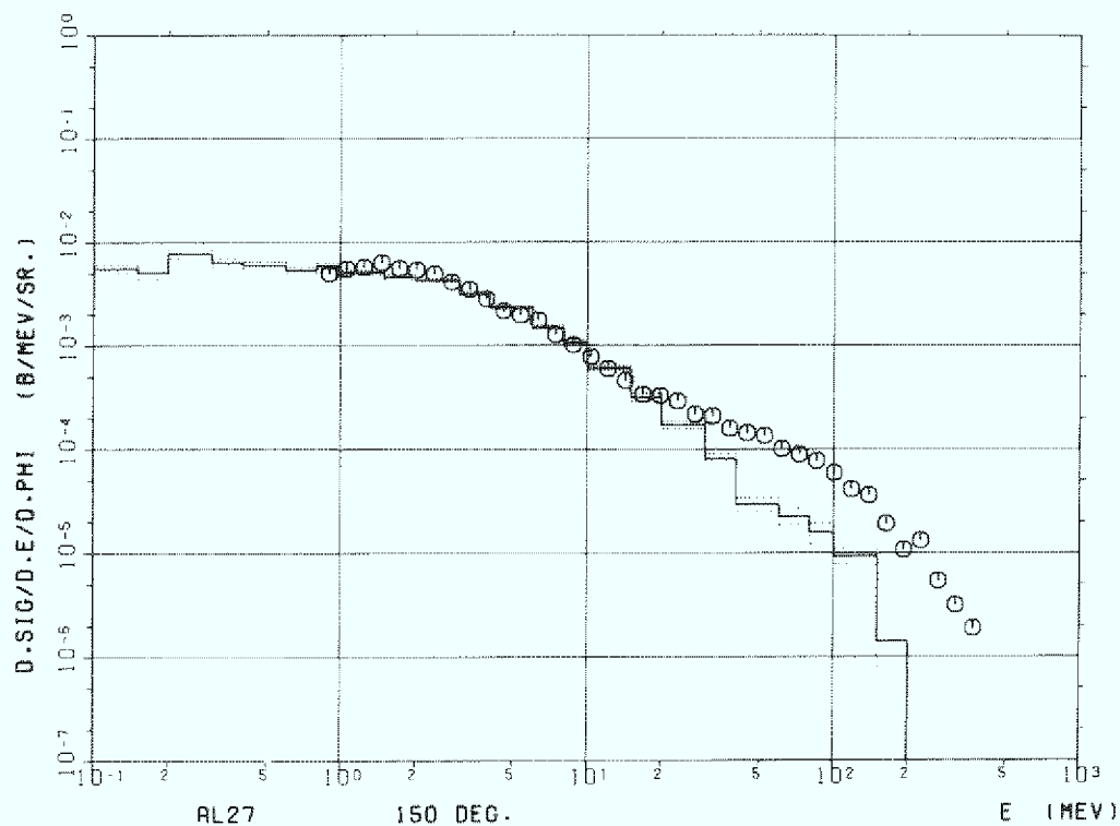
Figure 7c Aluminum (Al-27) 150°
