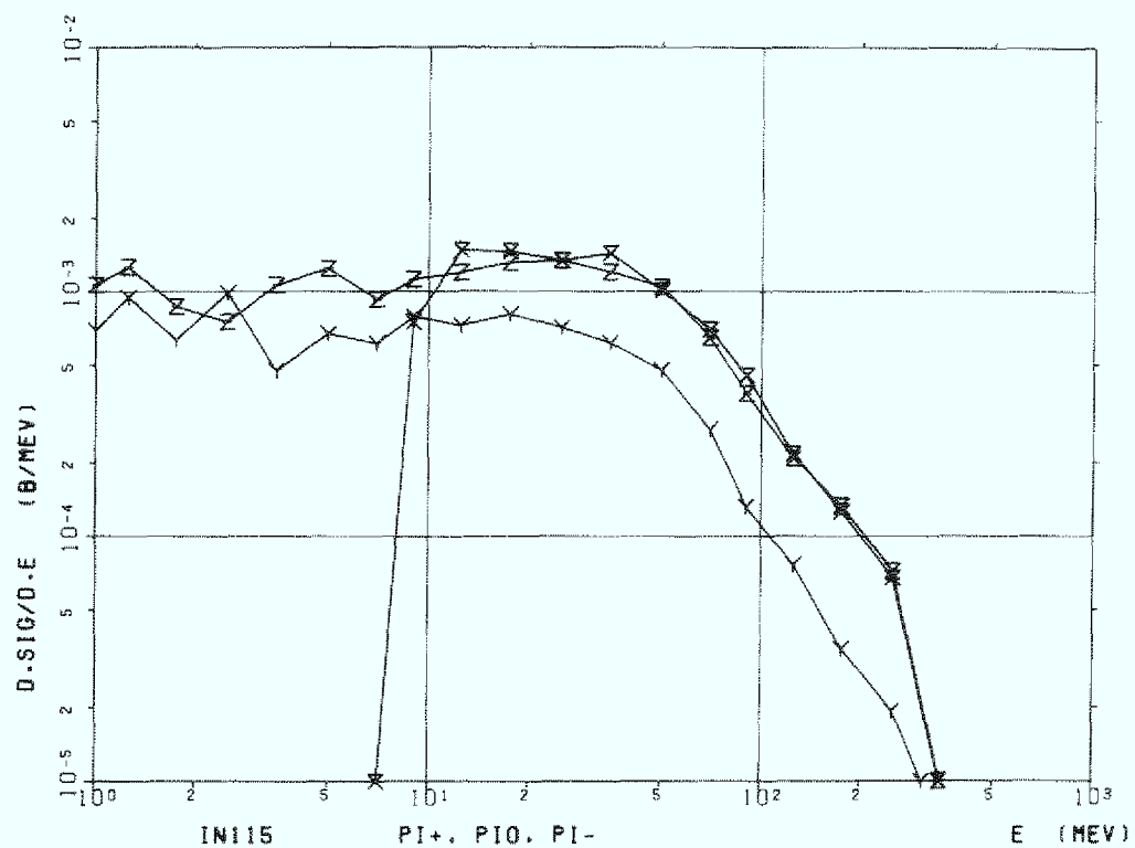
Figure C.4c Indium (In-115), \pi^+ , \pi^- and \pi^0
