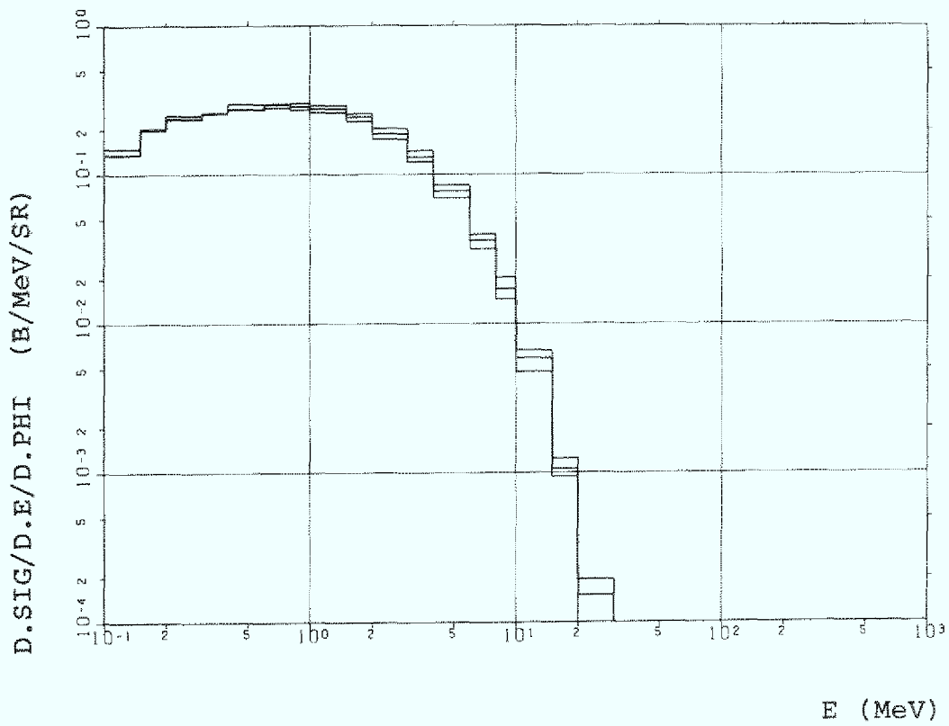
Figure A.2 Lead (Pb-207)
