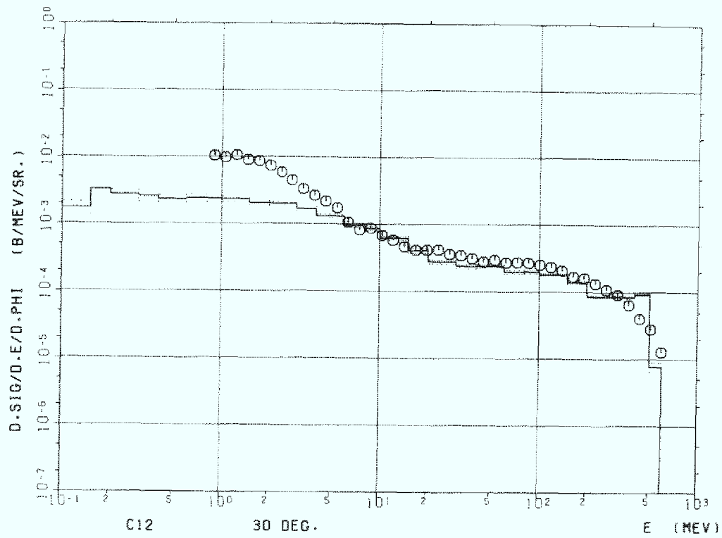
Figure 8a Carbon (C-12) 30°
