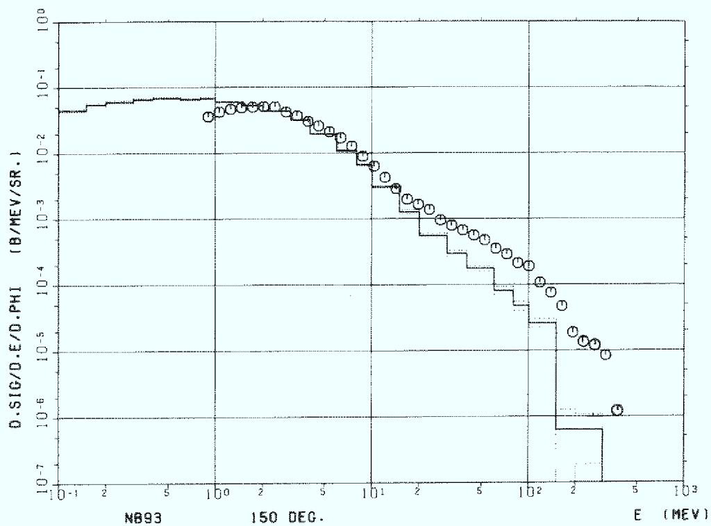
Figure 5c Niobium (Nb-93) 150°
