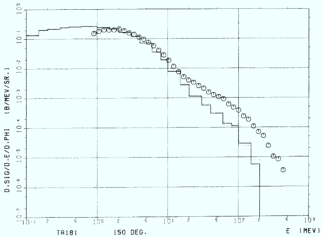
Figure 3c Tantalum (Ta-181) 150°
