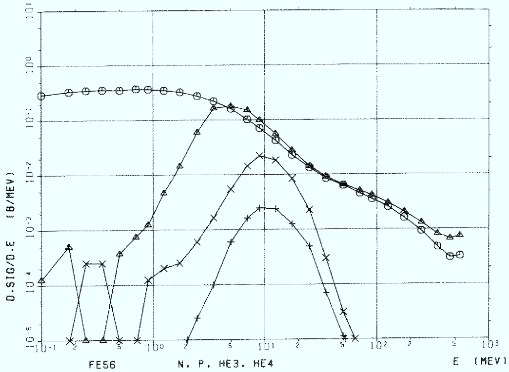
Figure C.6a Iron (Fe-56), n,p,He-3 and He-4
