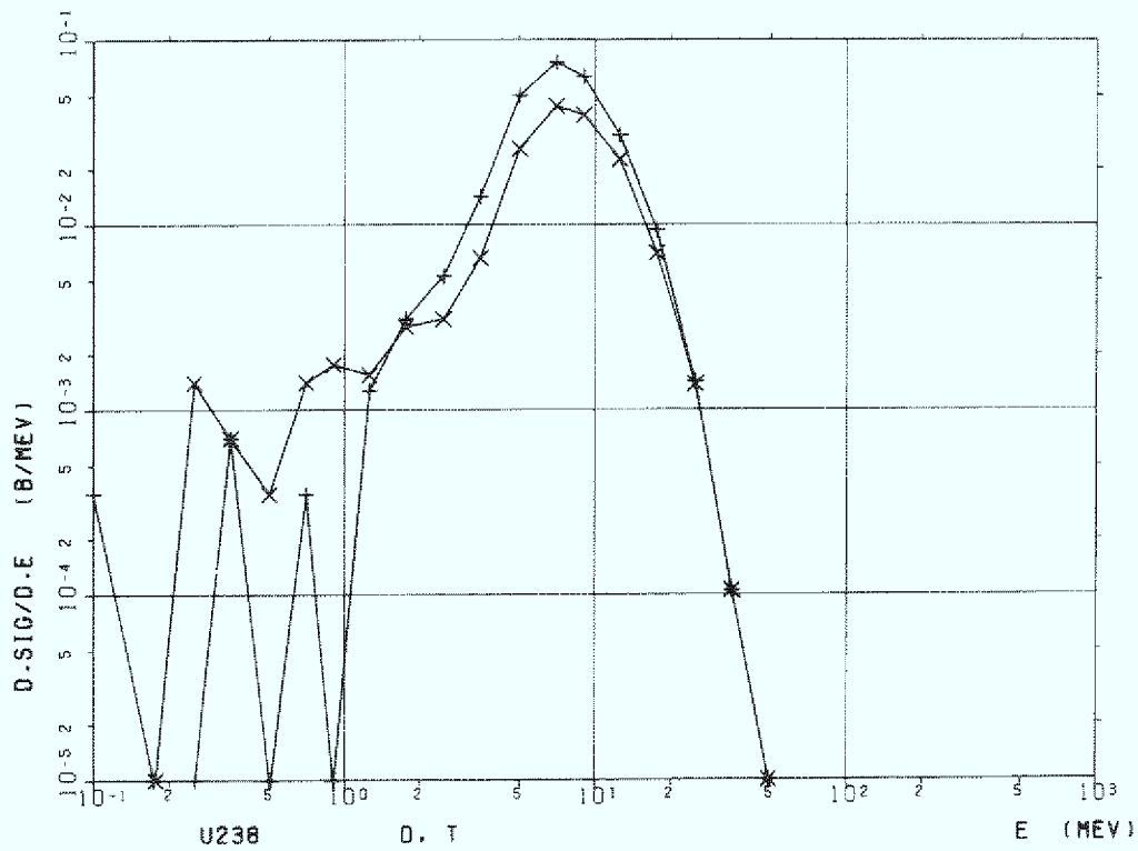
Figure C.1b Uranium (U-238), d and t
