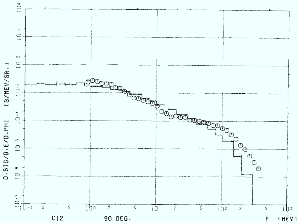
Figure 8b Carbon (C-12) 90°
