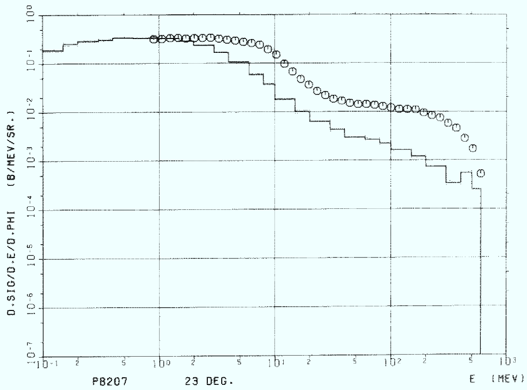
Figure B.1 Lead (Pb-207), 23^\circ
