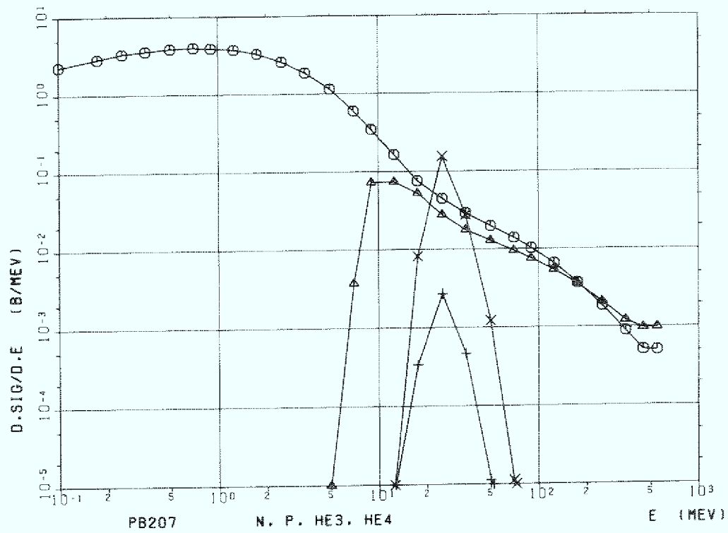
Figure C.2a Lead (Pb-207), n,p,He-3 and He-4
