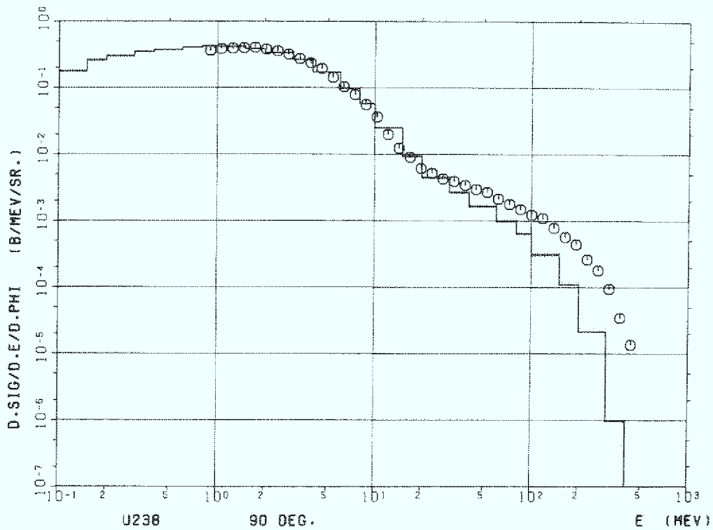
Figure 1b Uranium (U-238) 90°
