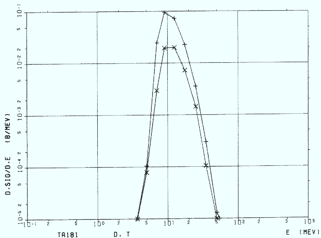
Figure C.3b Tantalum (Ta-181), d and t
