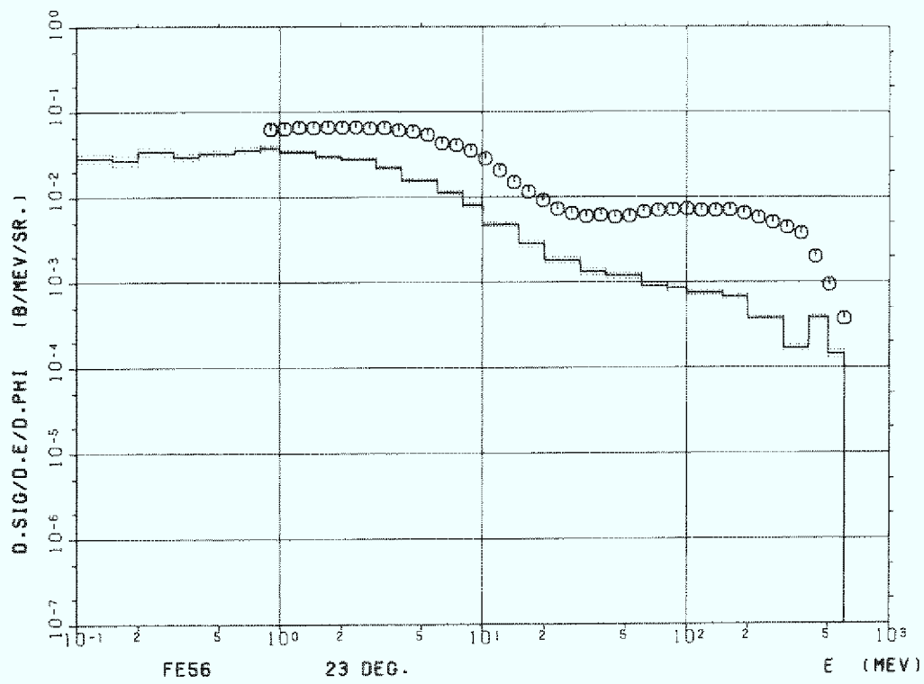
Figure B.5 Iron (Fe-56), 23^\circ
