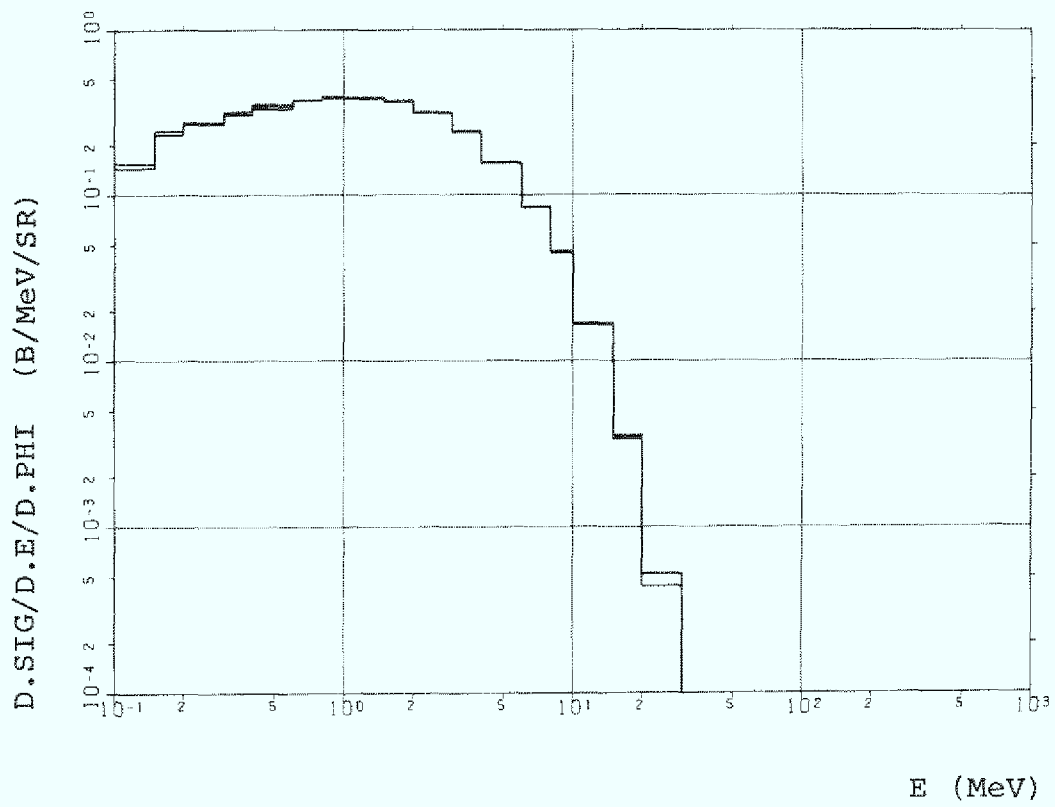
Figure A.1 Uranium (U-238)
