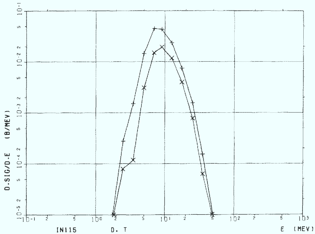
Figure C.4b Indium (In-115), d and t
