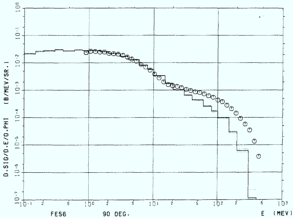
Figure 6b Iron (Fe-56) 90°
