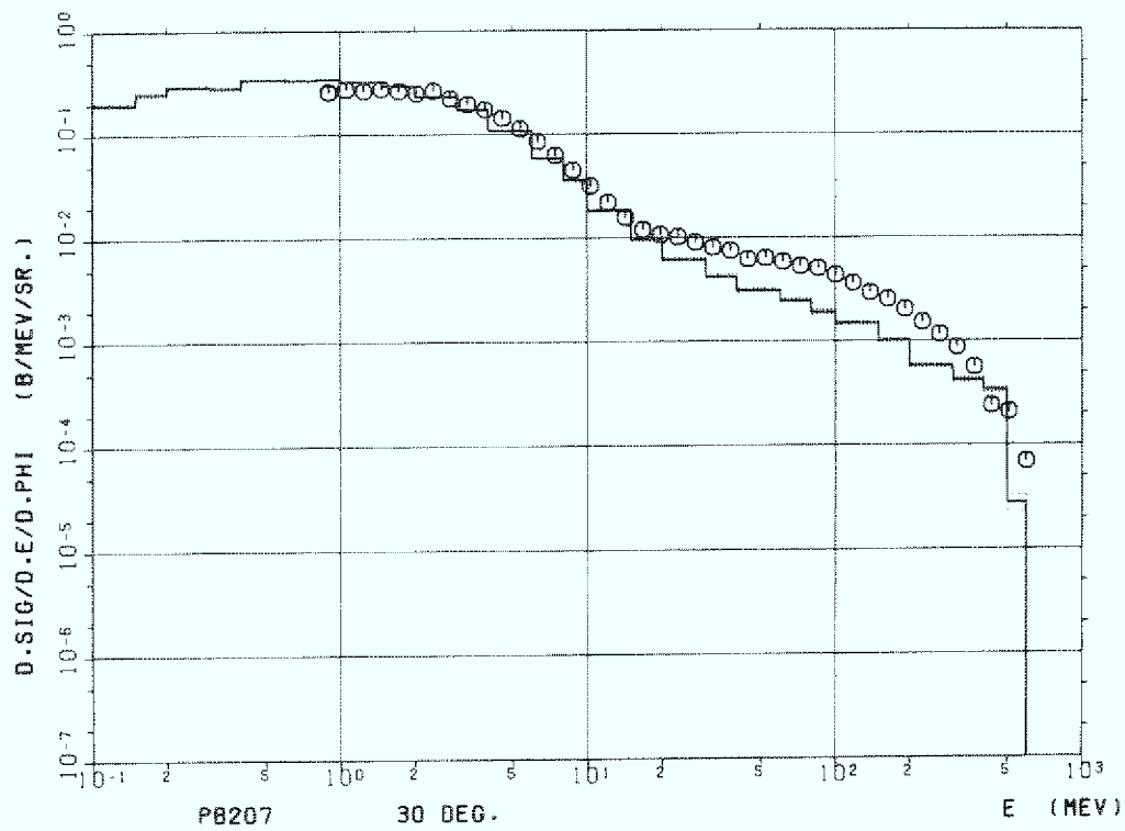
Figure 2a Lead (Pb-207) 30°
