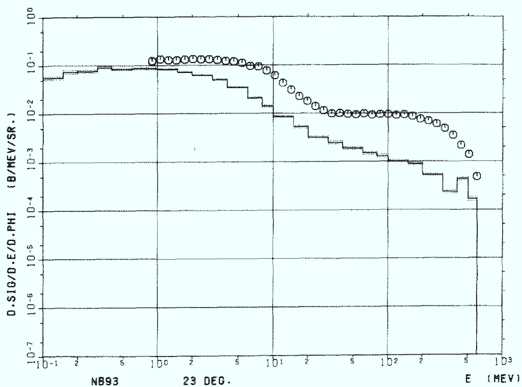
Figure B.4 Niobium (Nb-93), 23^\circ
