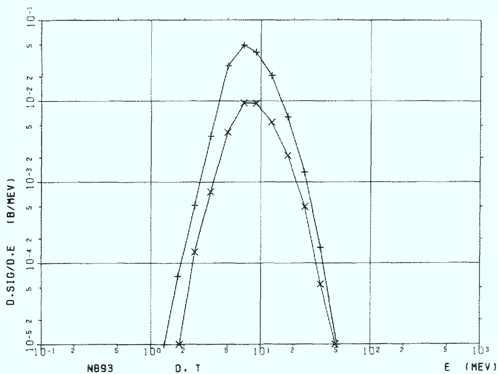
Figure C.5b Niobium (Nb-93), d and t
