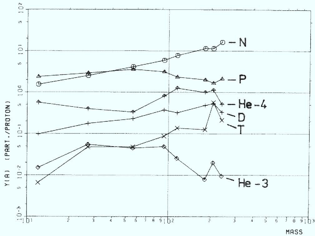
Figure 11 Total yields of n,p,d,t,He-3 and He-4 vs. mass number
