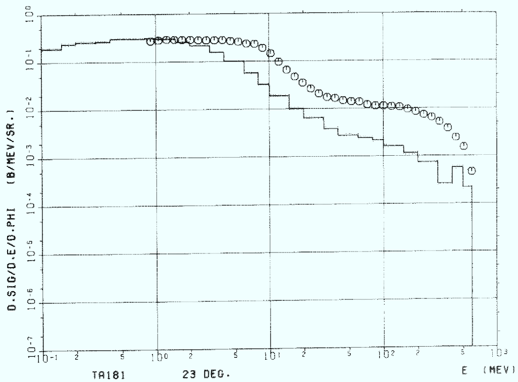
Figure B.2 Tantalum (Ta-181), 23^\circ
