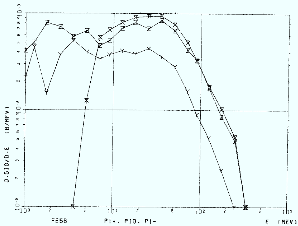
Figure C.6c Iron (Fe-56), \pi^+ , \pi^- and \pi^0
