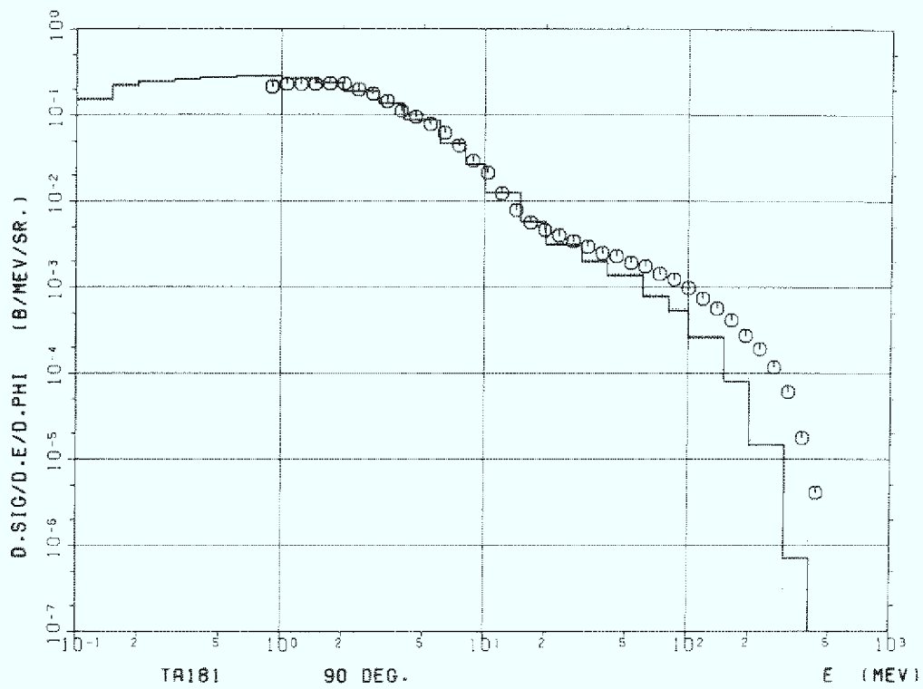
Figure 3b Tantalum (Ta-181) 90^\circ
