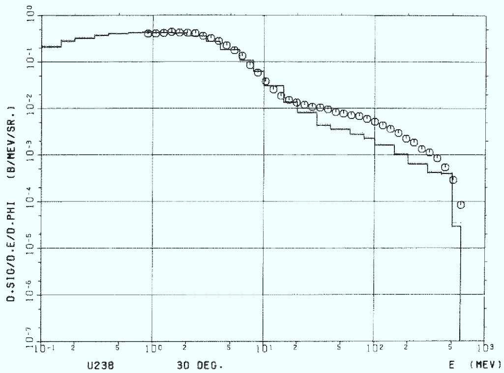
Figure 1a Uranium (U-238) 30°
