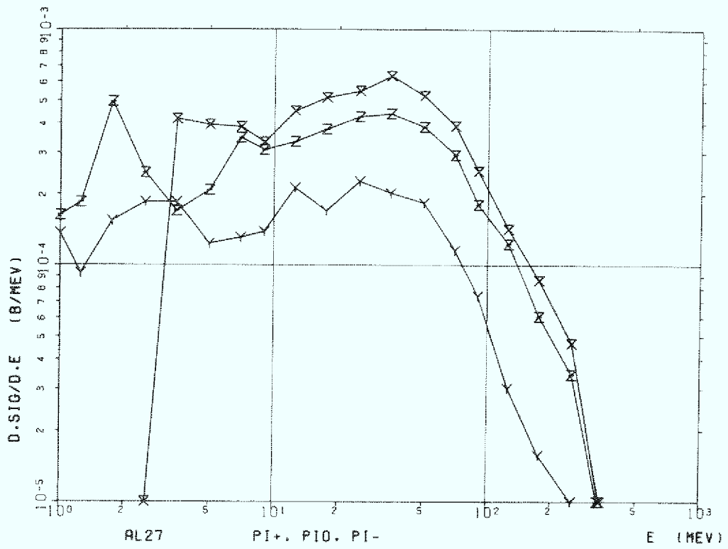
Figure C.7c Aluminum (Al-27), \pi^+ , \pi^- and \pi^0
