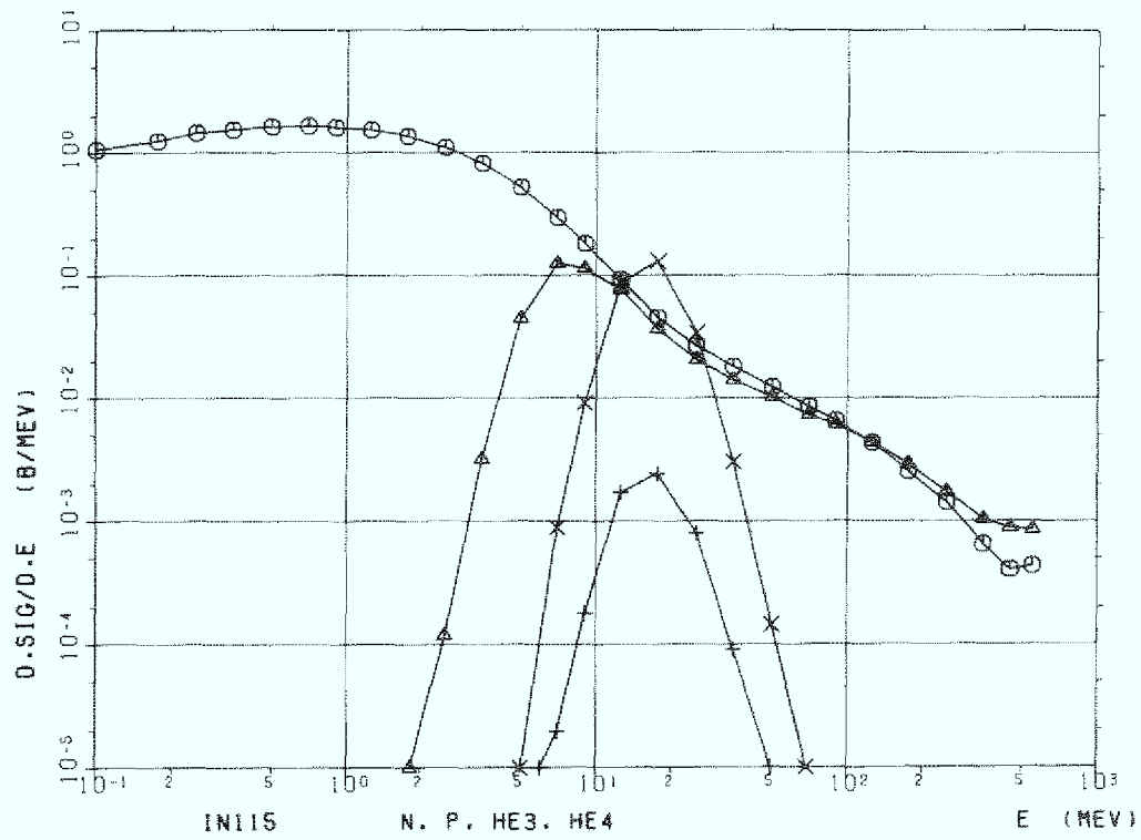
Figure C.4a Indium (In-115), n,p,He-3 and He-4
