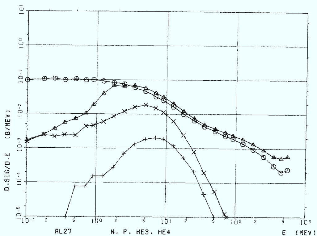
Figure C.7a Aluminum (Al-27), n,p,He-3 and He-4
