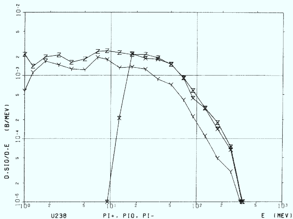
Figure C.1c Uranium (U-238), \pi^+ , \pi^- and \pi^0
