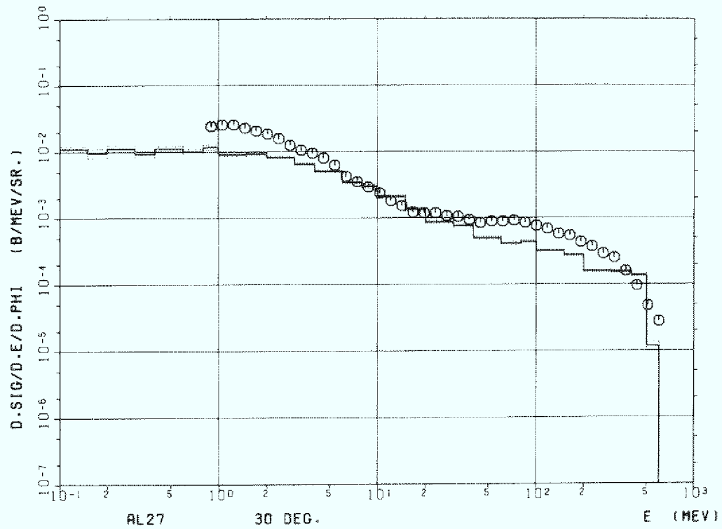
Figure 7a Aluminum (Al-27) 30°
