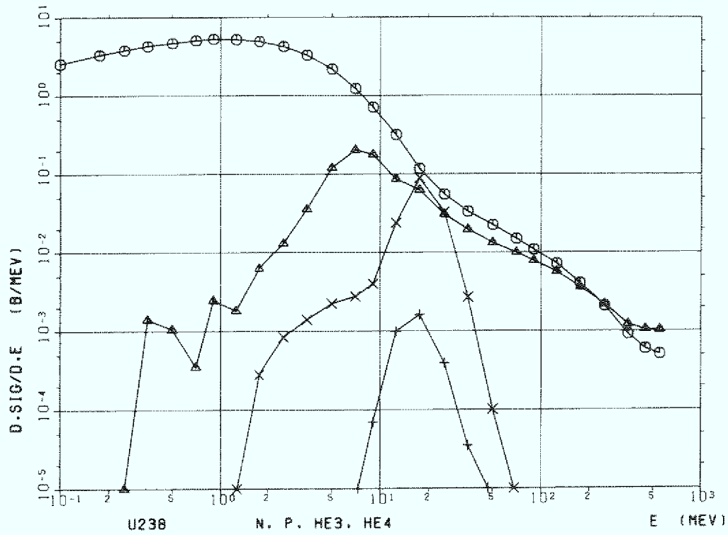
Figure C.1a Uranium (U-238), n,p,He-3 and He-4
