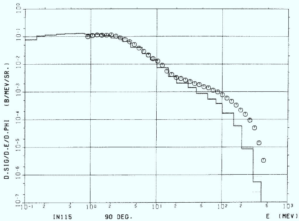
Figure 4b Indium ( In-115 ) 90^\circ
