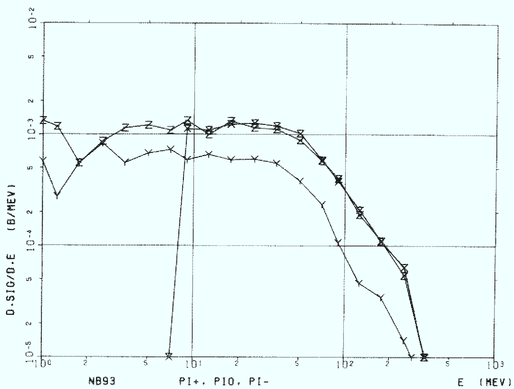
Figure C.5c Niobium (Nb-93), \pi^+ , \pi^- and \pi^0
