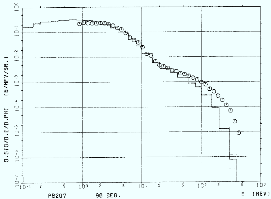
Figure 2b Lead (Pb-207) 90°
