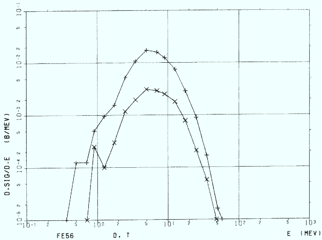
Figure C.6b Iron (Fe-56), d and t
