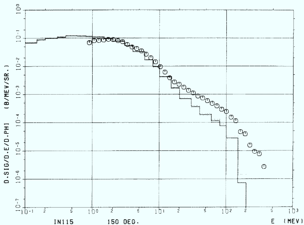
Figure 4c Indium (In-115) 150°
