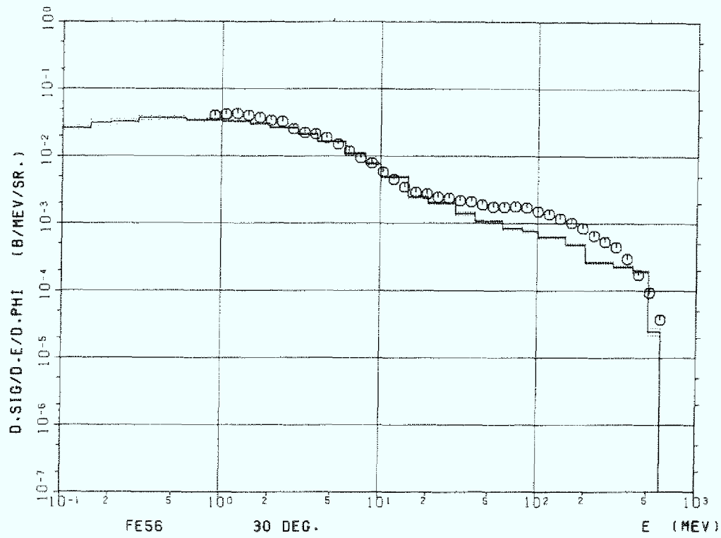
Figure 6a Iron (Fe-56) 30°
