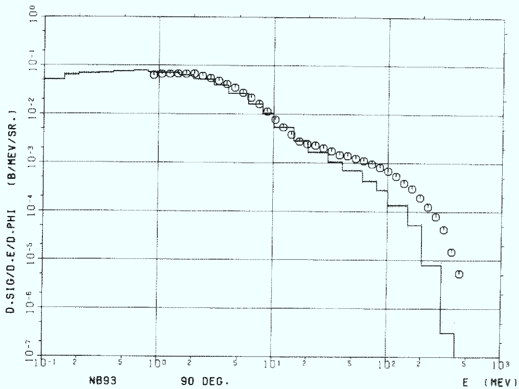
Figure 5b Niobium (Nb-93) 90^\circ
