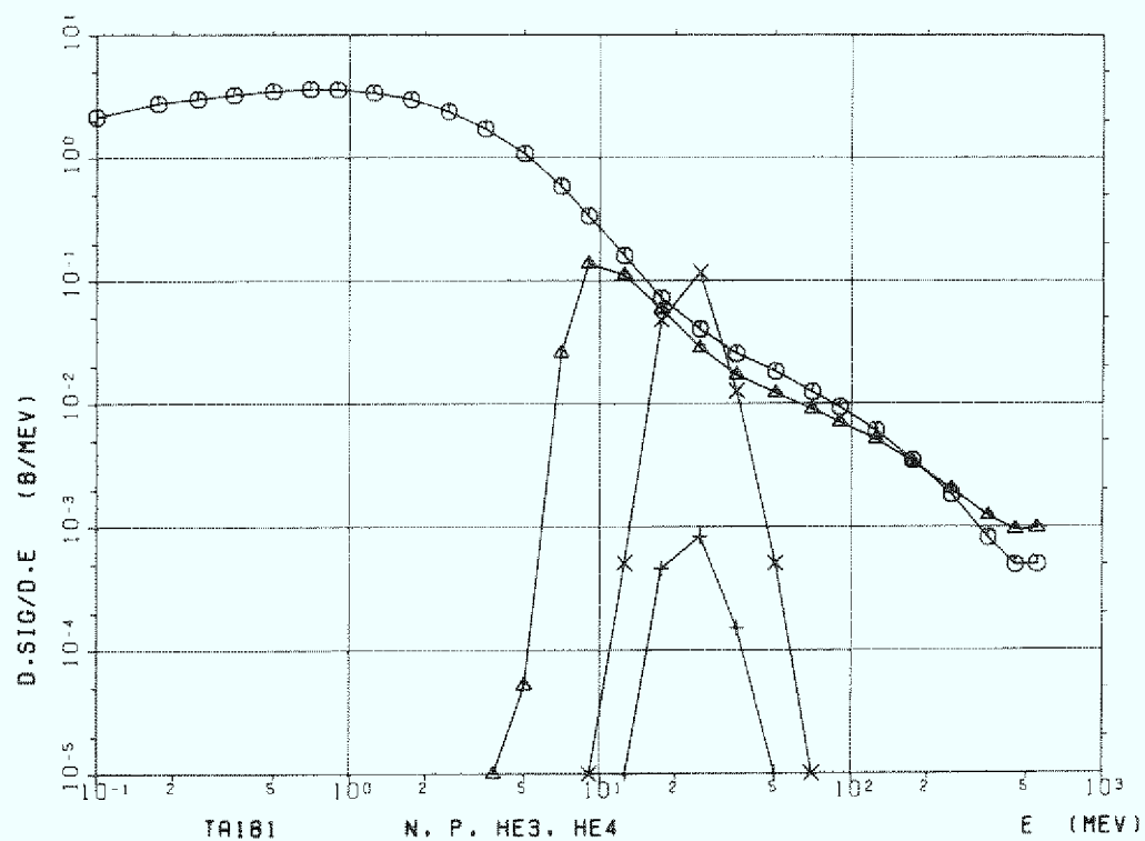
Figure C.3a Tantalum (Ta-181), n,p,He-3 and He-4
