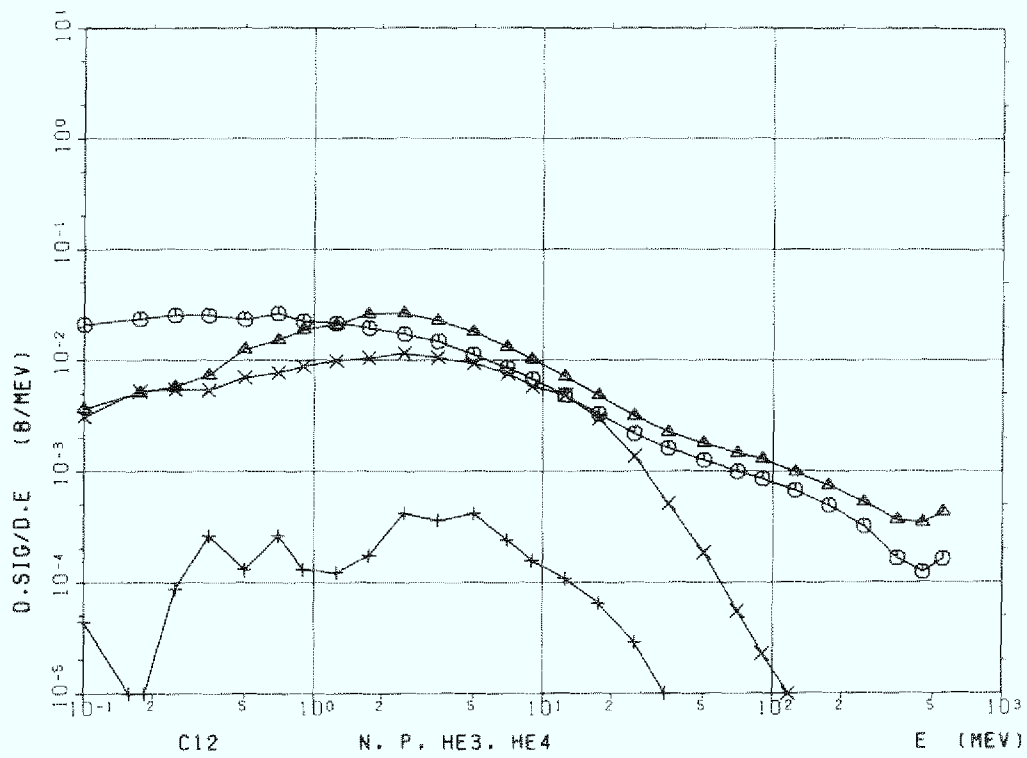
Figure C.8a Carbon (C-12), n,p,He-3 and He-4
