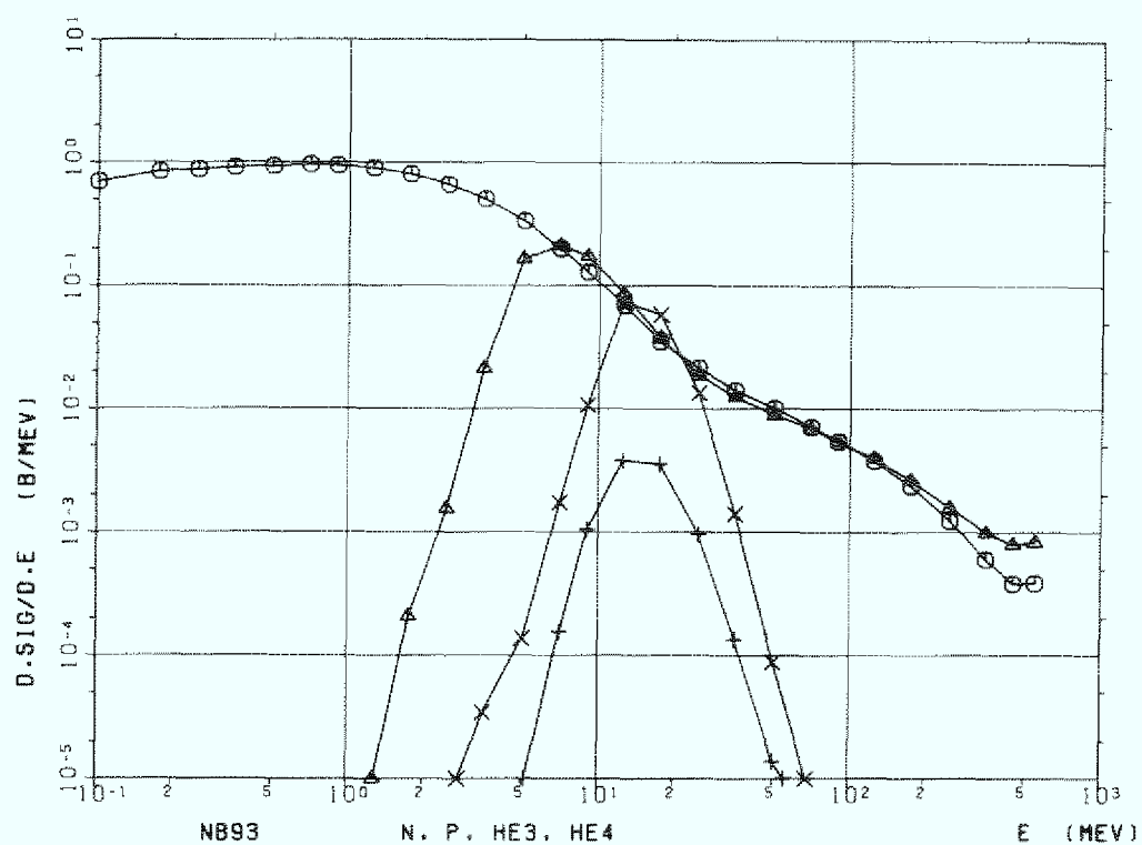
Figure C.5a Niobium (Nb-93), n,p,He-3 and He-4
