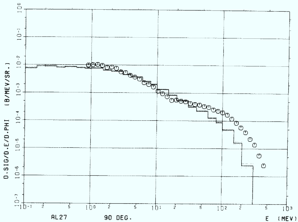
Figure 7b Aluminum (Al-27) 90°
