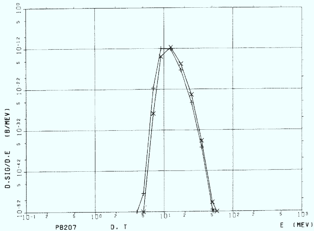
Figure C.2b Lead (Pb-207), d and t
