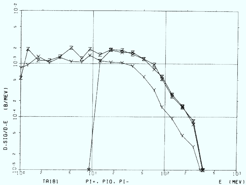
Figure C.3c Tantalum (Ta-181), \pi^+ , \pi^- and \pi^0
