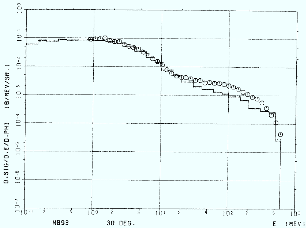
Figure 5a Niobium (Nb-93) 30^\circ
