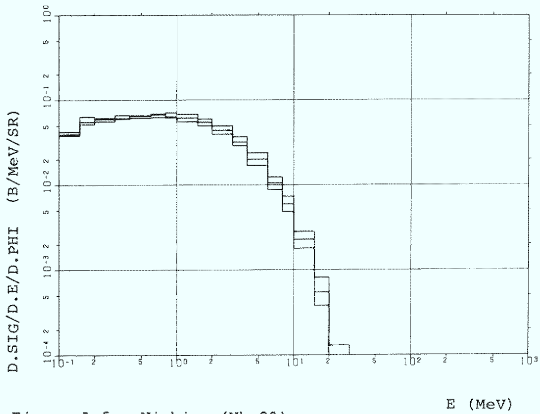
Figure A.5 Niobium (Nb-93)
