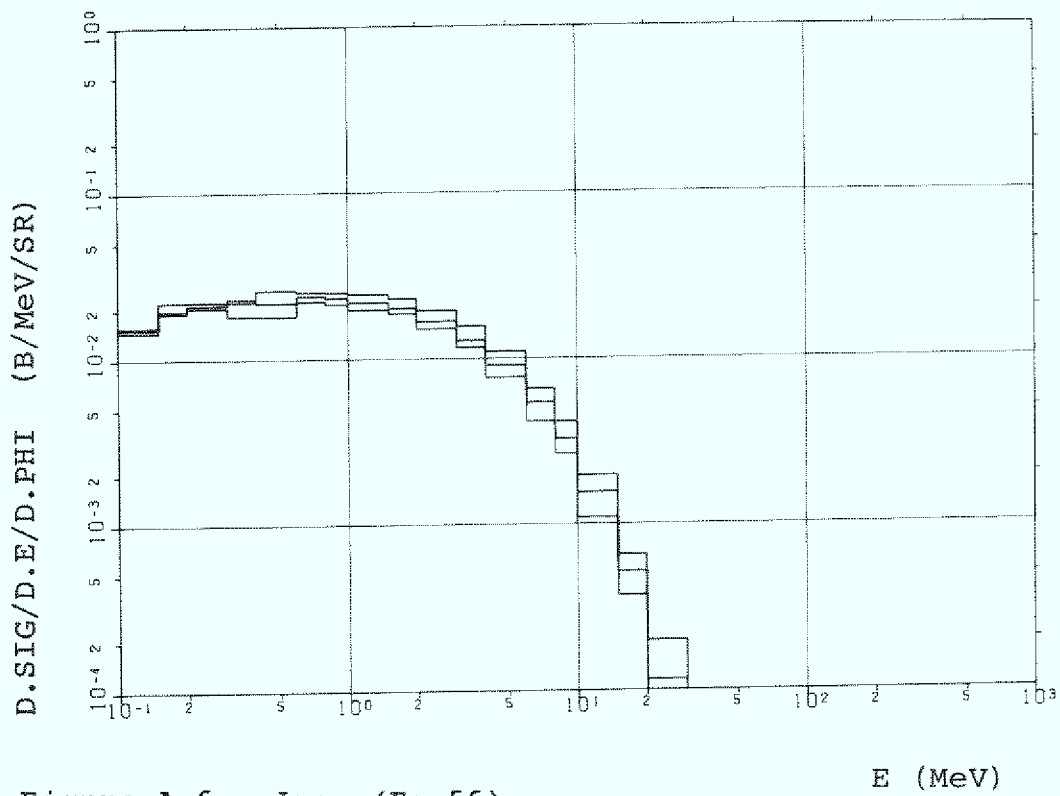
Figure A.6 Iron (Fe-56)
