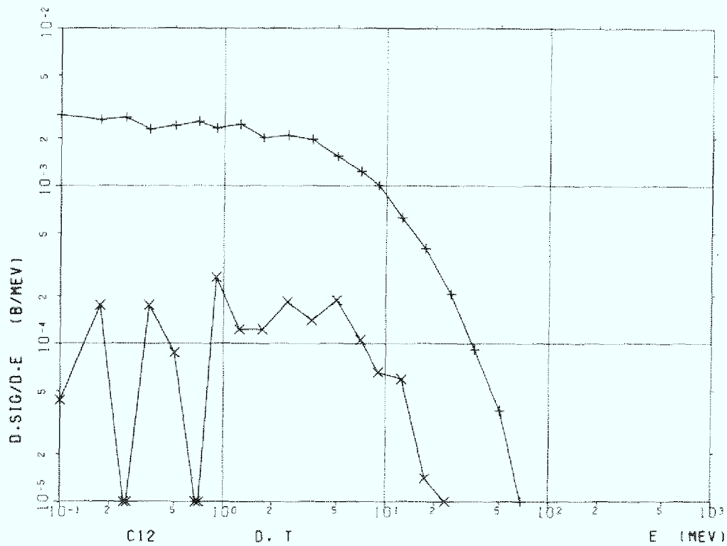
Figure C.8b Carbon (C-12), d and t
