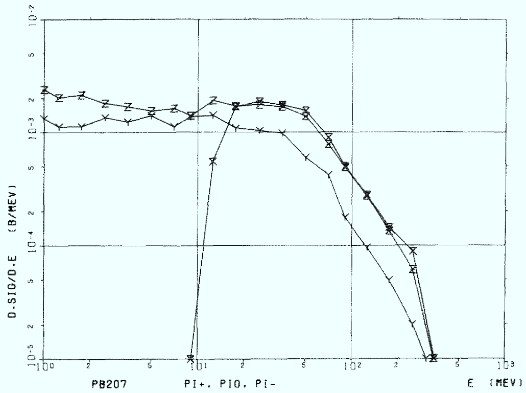
Figure C.2c Lead ( Pb-207 ), \pi^+ , \pi^- and \pi^0
