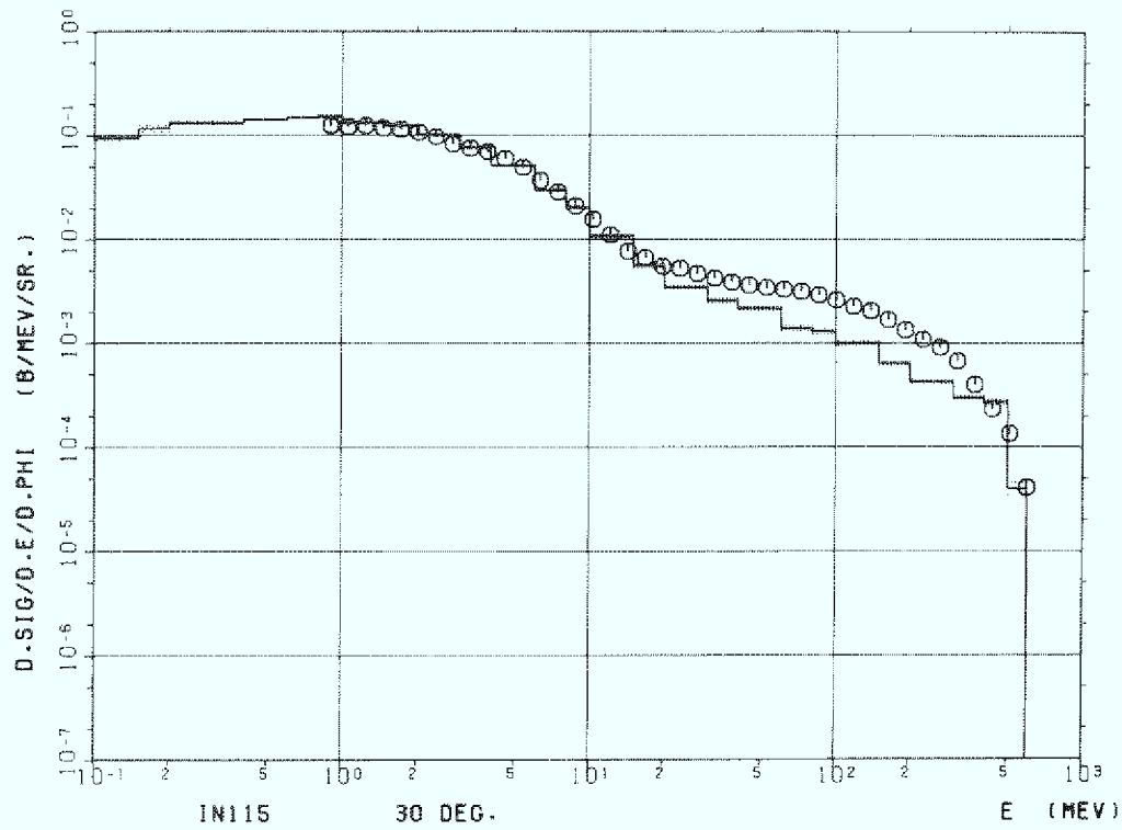
Figure 4a Indium ( In-115 ) 30^\circ
