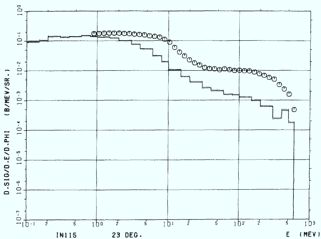
Figure B.3 Indium (In-115), 23^\circ
