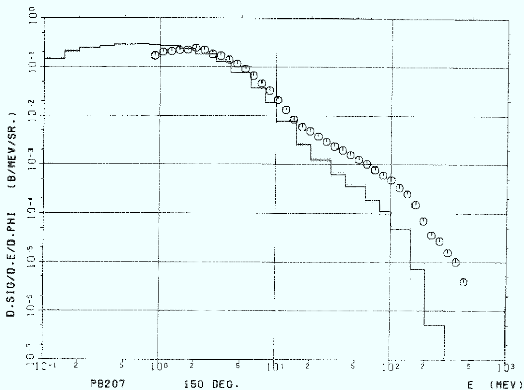
Figure 2c Lead (Pb-207) 150°
