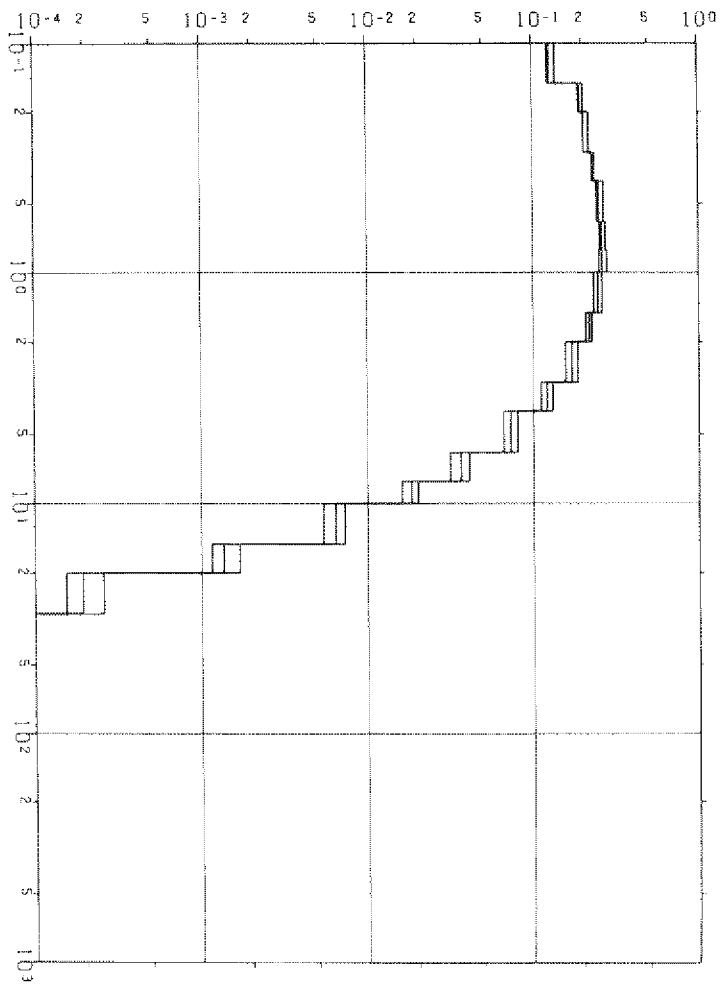
Figure A.3 Tantalum ( Ta-181 )
