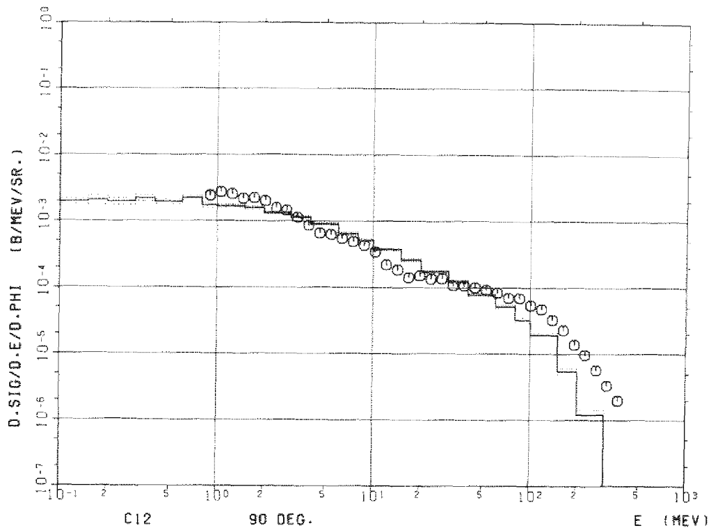
Figure 8b Carbon (C-12) 90^\circ
