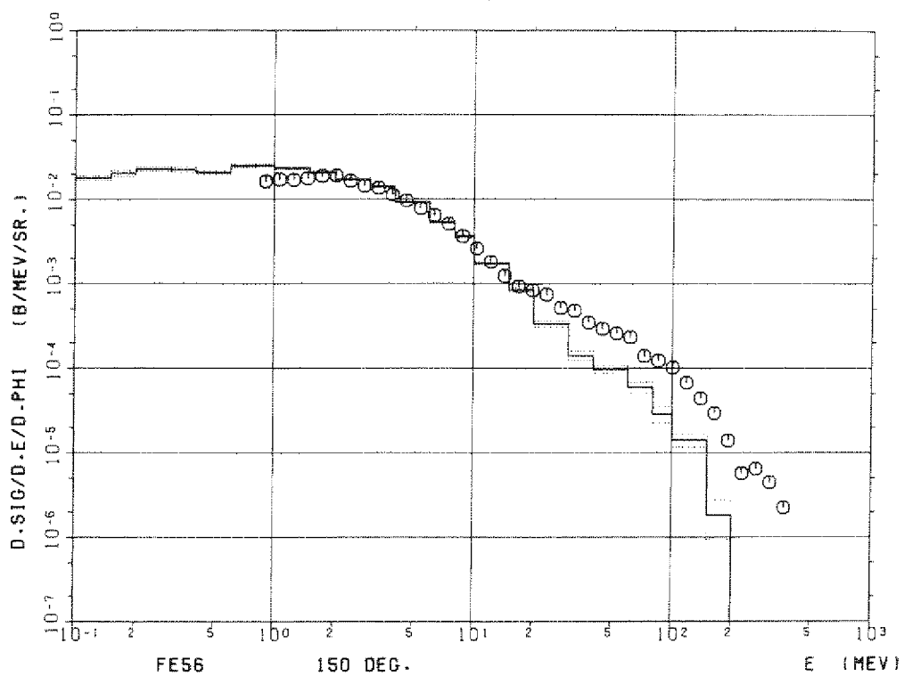
Figure 6c Iron (Fe-56) 150°
