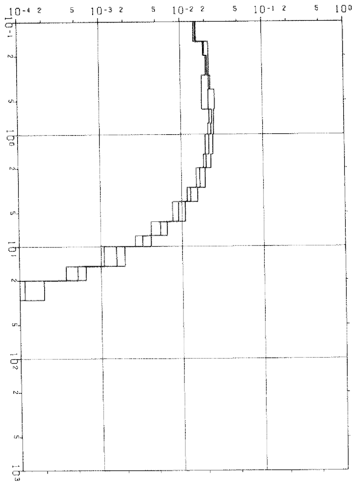
Figure A.6 Iron ( Fe-56 )
