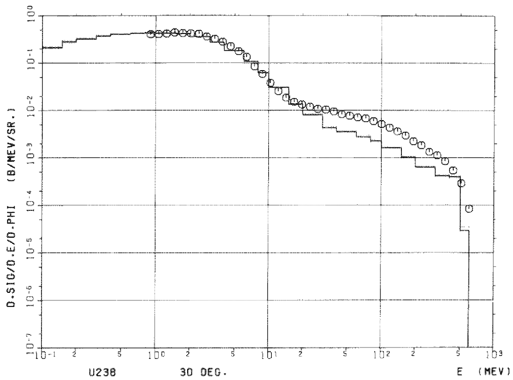
Figure 1a Uranium (U-238) 30^\circ
