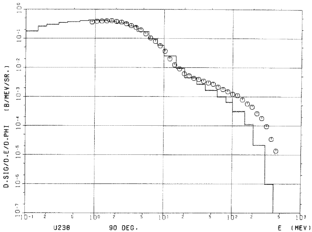
Figure 1b Uranium (U-238) 90^\circ
