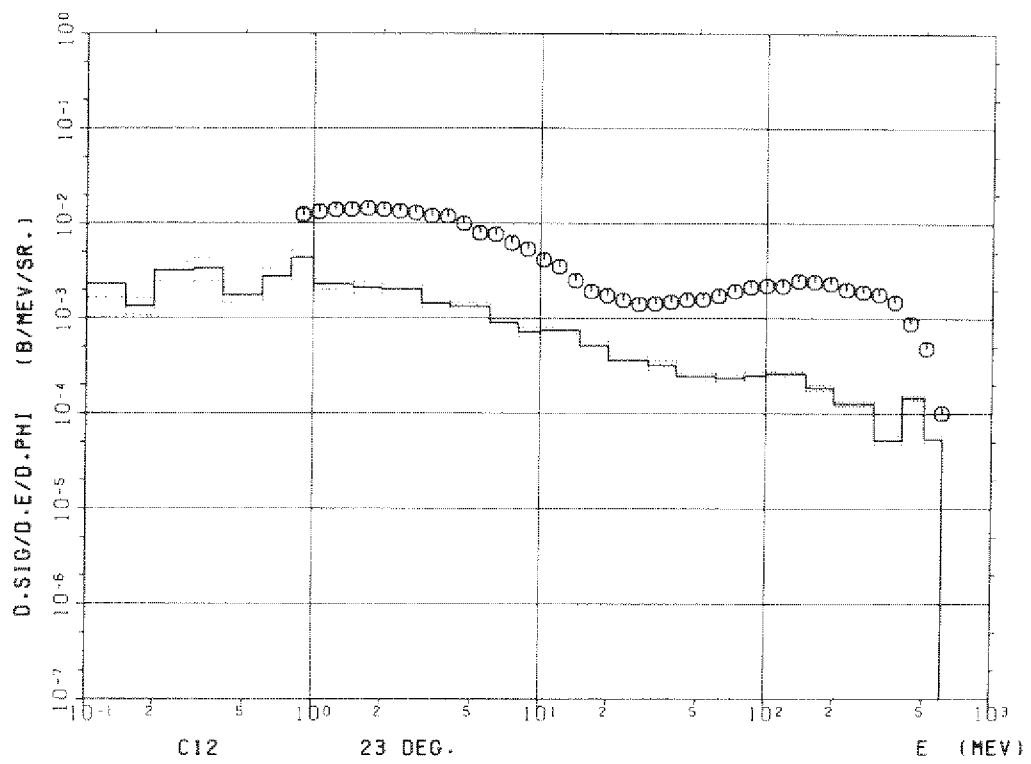
Figure B.7 Carbon (C-12), 23°
