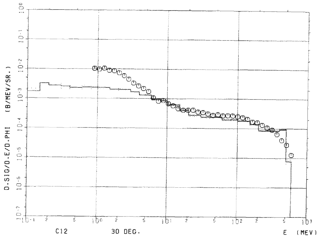
Figure 8a Carbon (C-12) 30^\circ
