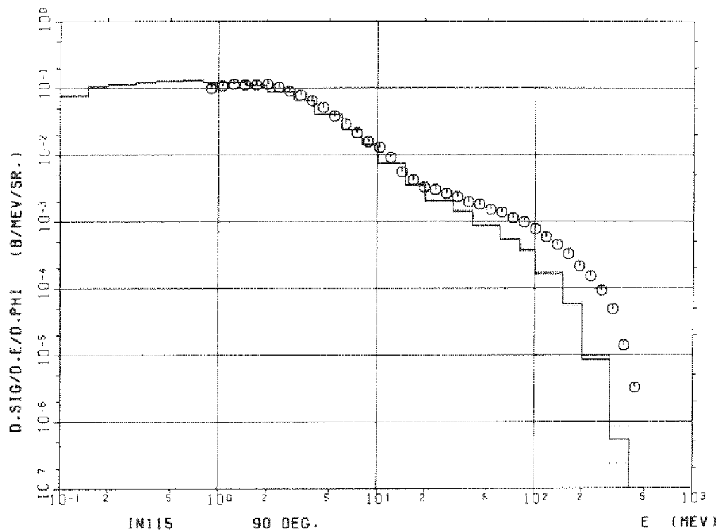
Figure 4b Indium ( In-115 ) 90^\circ
