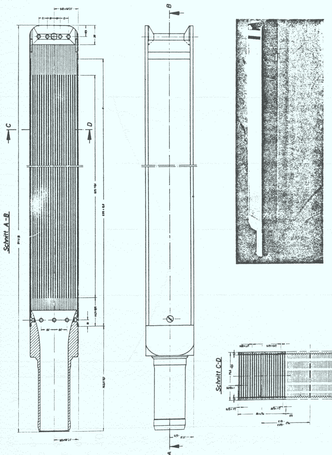
Abb. 1.3 Standard-Brennelement
