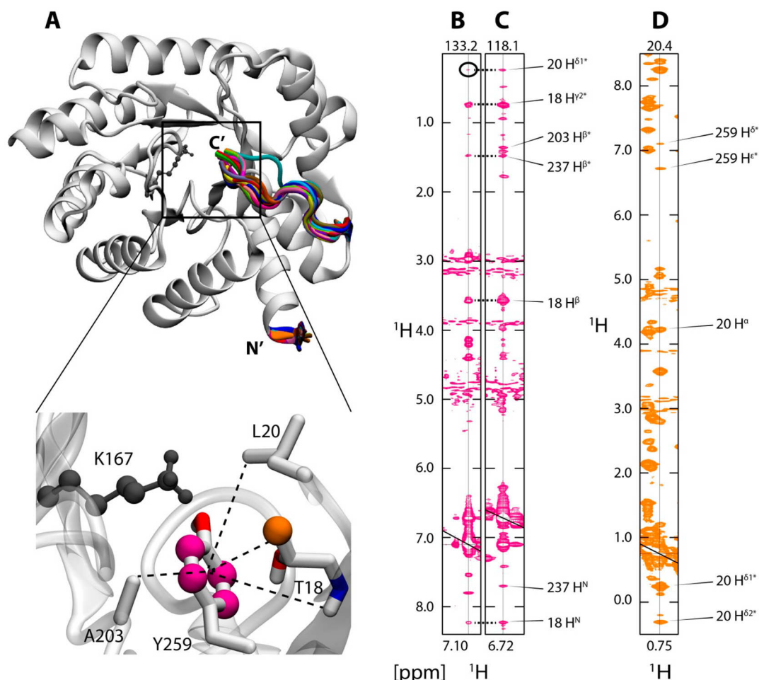
Figure 4. NOE distance restraint derived structural ensemble of DERAm C-terminal tail closed state. (A) A set of 48 NOEs satisfies the closed state ensemble. The inset shows that the presence of Y259 inside the active site is supported by NOEs (dashed lines) to nearby residues. Strips from ^{13}\text{C} -edited NOESY spectra showing inter-residue NOE interactions for 259 \text{H}^{\delta*} (B), 259 \text{H}^{\epsilon*} (C), and 18 \text{H}^{\gamma 2*} (D) protons. Weak NOE between 259 \text{H}^{\delta*} and 20 \text{H}^{\delta 1*} is highlighted by a black circle in (B). ^{13}\text{C} chemical shifts for 259 \text{C}^{\delta*} , 259 \text{C}^{\epsilon*} , and 18 \text{C}^{\gamma 2*} are displayed at the top of the NOESY strips in (B)–(D), respectively.
