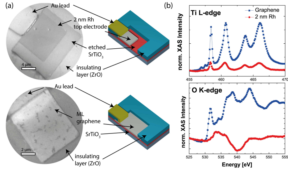
Figure 6.13. – (a) Vertical MIM \text{SrTiO}_3 devices: XAS images of 2 nm Rh (top) and 1 ML graphene (bottom) electrodes. (b) Ti L_{2,3} -edge absorption spectra and O K-edge absorption spectra collected from underneath 1 ML graphene (blue) and 2 nm Rh (red). In contrast to the Rh overlayer, the graphene top electrode exhibits less absorption and shows more details of the Ti L_{2,3} and especially of the O K-edge line shape. The average transmissivity of the graphene electrodes was calculated to be 7 – 10 times larger as compared to the Rh electrodes.
