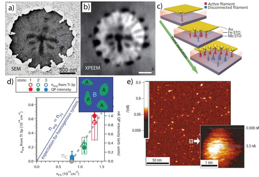
Figure 5.11. – (a) SEM image of a micron sized filamentary area in Fe : SrTiO 3 , (b) high resolution XPEEM XAS image of the same device imaged at a photon energy E_{\text{ph}} = 459.9 eV characteristic for tetravalent titanium (Ti 4+ ) (c) Multi filament model to explain large filamentary areas. A detailed explanation is given in [64]. (d) Mismatch between the expected charge carrier density (blue line) for a homogenous surface reduction of SrTiO 3 single crystals and the charge carrier densities measured from Fermi surfaces (data points). The deviation is explained by the presence of Ti 3+ rich islands (inset) [66]. (e) LC-AFM study on a SrTiO 3 single crystal surface: Observation of nanoscale conductive filaments with diameters of a few nm [24].
