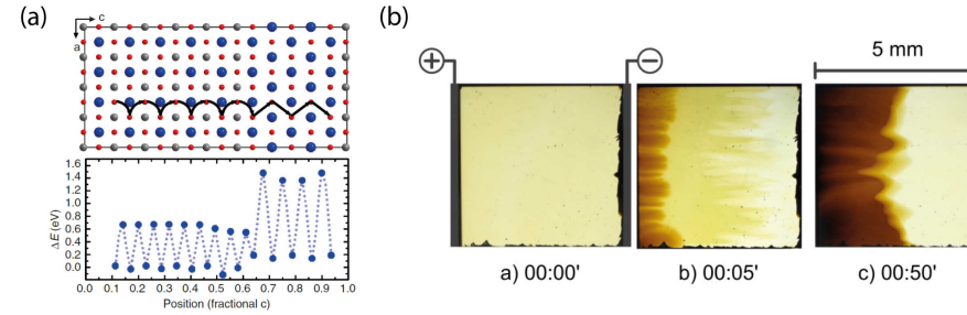
Figure 2.6. – (a) Migration of an oxygen atom across a \text{SrTiO}_3/\text{SrO} interface layer via lattice site hopping (black line, top). The activation energy per hop is show on the bottom. Taken from Ref. [27] (b) Electro coloration in 0.05% Fe doped \text{SrTiO}_3 single crystal under the application of 200V with a current compliance of 1 mA. Adapted from Ref. [28]
