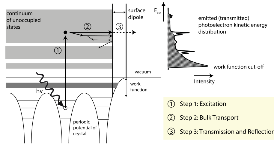
Figure 4.1. – Three-step model of the photoemission process: (1) A photon with energy E = h\nu is absorbed by a bound electron in the solid, which in turn is excited into the continuum of unoccupied states. (2) During its travel through the crystal the electron undergoes elastic and inelastic scattering events. (3) When the electron reaches the surface it has to overcome a surface potential barrier before being transmitted into vacuum. The kinetic energy distribution of the emitted electrons is a replica of the electronic states in the crystal. Image inspired by [50]
