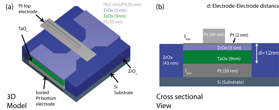
Figure 6.3. – (a) Three-dimensional representation and (b) cross sectional representation of TaO x /ZrO x crossbar devices with Pt/ZrO x /TaO x /Pt layer stacking.
