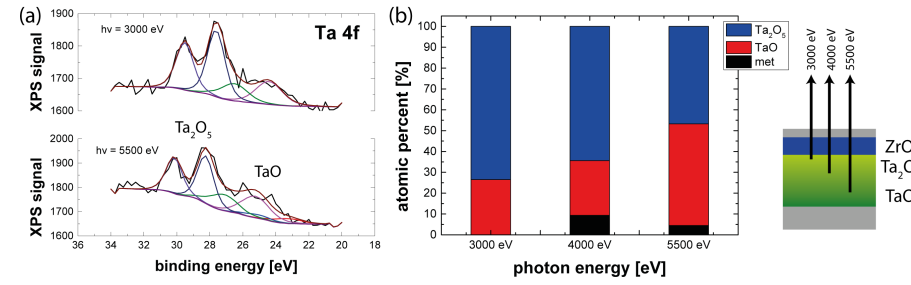
Figure 6.6. – (a) Ta 4f XPS spectra of the junction area (black) for h\nu = 3000 eV and h\nu = 5500 eV. (b) Fitted relative contributions of Ta, TaO and \text{Ta}_2\text{O}_5 for different photon energies. For higher photon energies an increasing contribution of the TaO component is observed.
