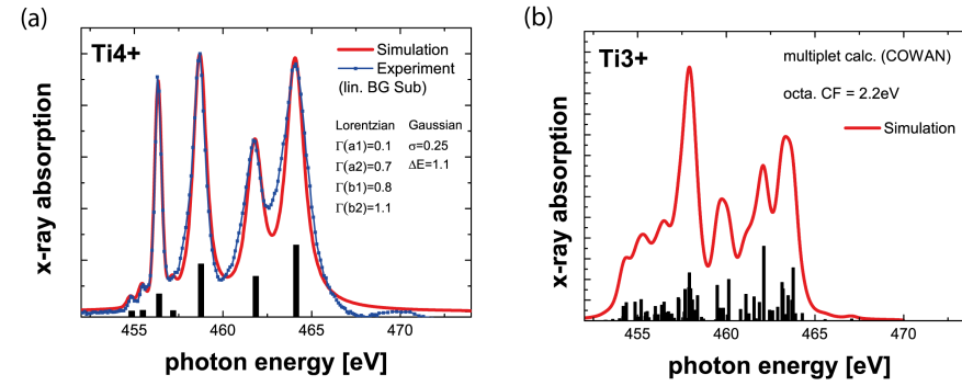
Figure 3.4. – (a) Atomic multiplet calculations for tetravalent Ti in octahedral symmetry (black bars) using CTM4XAS. The crystal field splitting is set to \Delta_0 = 2.2 eV. The simulated transition probabilities are artificially broadened (red) to match experimental X-ray absorption spectra of stoichiometric \text{SrTiO}_3 (blue) (b) the same simulations performed for trivalent Ti.
