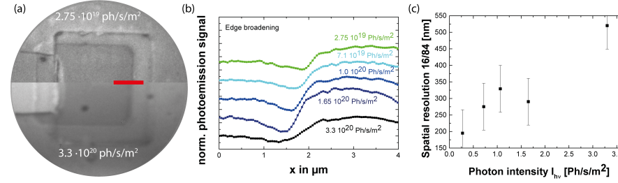
Figure 6.7. – (a) XPEEM images at the secondary cut-off acquired for two different photon intensities. The bottom part of the image is blurred and shows intensity modifications related to space charge effects. (b) corresponding line profiles of the edge marked by the red line for different photon intensities. (c) The spatial resolution derived from the line shapes according to the 16/84 criterion.
