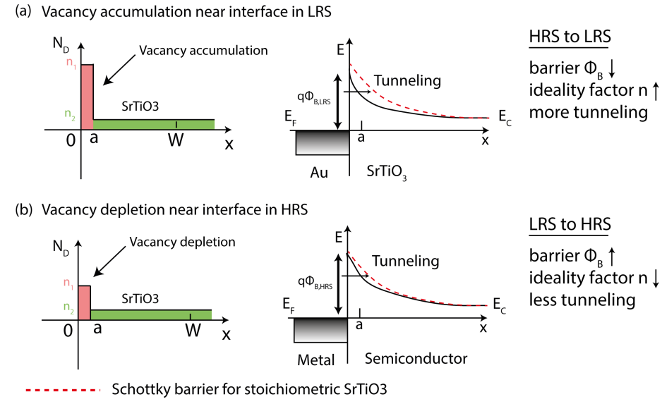
Figure 8.17. – Influence of defect density modulations at the metal/oxide interface. (a) High donor densities N_D in the electrode vicinity lower the barrier and enable tunneling. (b) A decrease of the donor density increases the barrier height and enlarges the tunneling distance. Adapted from Sze, Wiley. [30]
