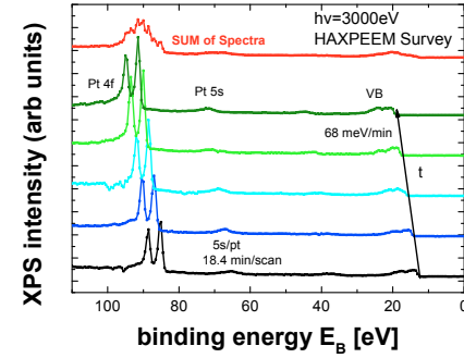
Figure 6.8 – Sample charging effects observed during HAXPEEM ( h\nu = 3000 eV) survey scans of Pt/TaOx/Pt devices. Each scan took 18.4 min and a linear shift between subsequent scans can be observed. This indicates a constant charging of the sample surface with 68 meV/min. The red line is representative for a long exposure spectrum.
