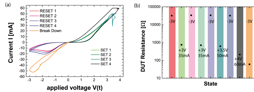
Figure 8.11. – (a) I-V characteristics of an Au/G/STO/Nb:STO device mounted in the microscope in 'moving potential configuration' and measured by the external Keithley 2611A source meter (b) READ measurements of the device resistance after each cycle (corresponding to the color scheme in a). The resistance values were extracted at +0.2 V read out voltage.
