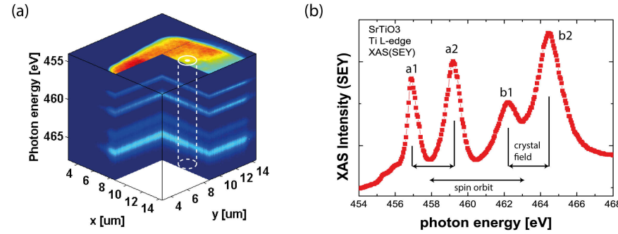
Figure 5.5. – (a) Ti L-edge XAS-PEEM scan of a single, delaminated device in the HRS plotted in three dimensions. The x - and y -axis define the spatial coordinates. The z -axis encodes the photon energy. The area indicated by the white line was chosen for a cut along the photon energy ( z -axis), plotted on the right. (b) The Ti L-edge XAS line shape of the chosen region is characteristic for tetravalent titanium in an octahedral configuration.
