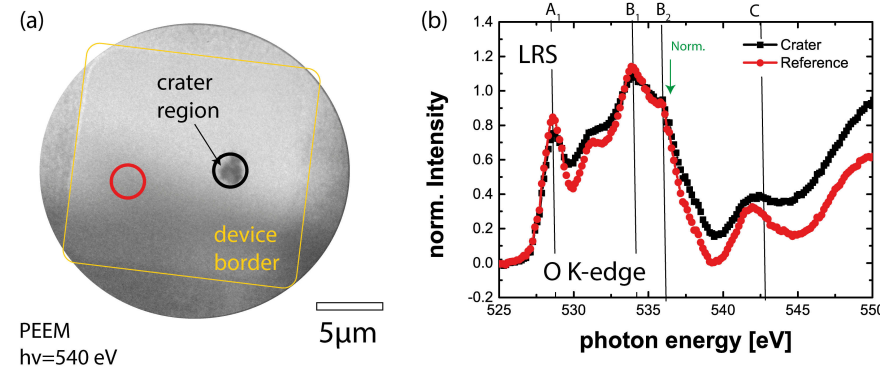
Figure 5.7. – (a) XAS-PEEM image showing a modified region of approximately 1\ \mu\text{m} in diameter in an else homogenous matrix. (b) XAS spectrum of the O K-edge extracted from the crater region (black) compared to a reference spectrum extracted from the unaltered surrounding (red). The spectra are normalized to peak B_2 .
