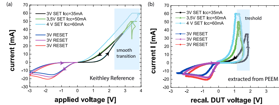
Figure 8.16. – (a) I-V curve of device operation measured by external Keithley (b) I-V curve of the DUT without parasitic influences deducted from XPEEM measurements.
