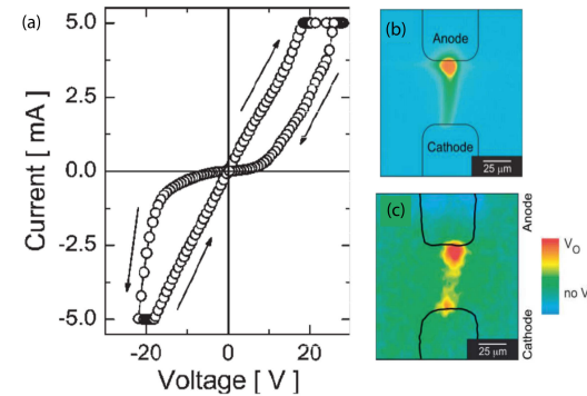
Figure 6.9 – Lateral Cr-doped SrTiO 3 resistive switching device. Images are adapted from ref. [82]. (a) I-V curve for switching cycle (b) thermal distribution during operation derived from infrared emission (c) oxygen vacancy concentration recalculated from Cr x-ray fluorescence. For details see ref. [82]
