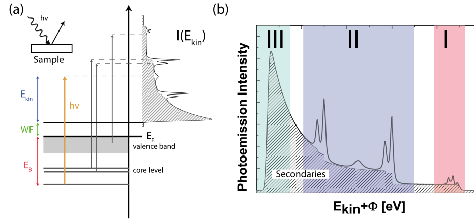
Figure 4.4. – (a) Scheme of a photoemission process. The photon energy (yellow) is transferred to an electron bound in the solid. Some of the energy is consumed to overcome the binding energy E_B (red) and the surface potential \Phi (green). The remaining energy is left in form of kinetic energy E_{kin} (blue). (b) Schematic photoemission spectrum: The measured electron kinetic energy E_{kin} is plotted versus the intensity I of the photoemission signal. Three characteristic regions can be distinguished, which are explained in the text.
