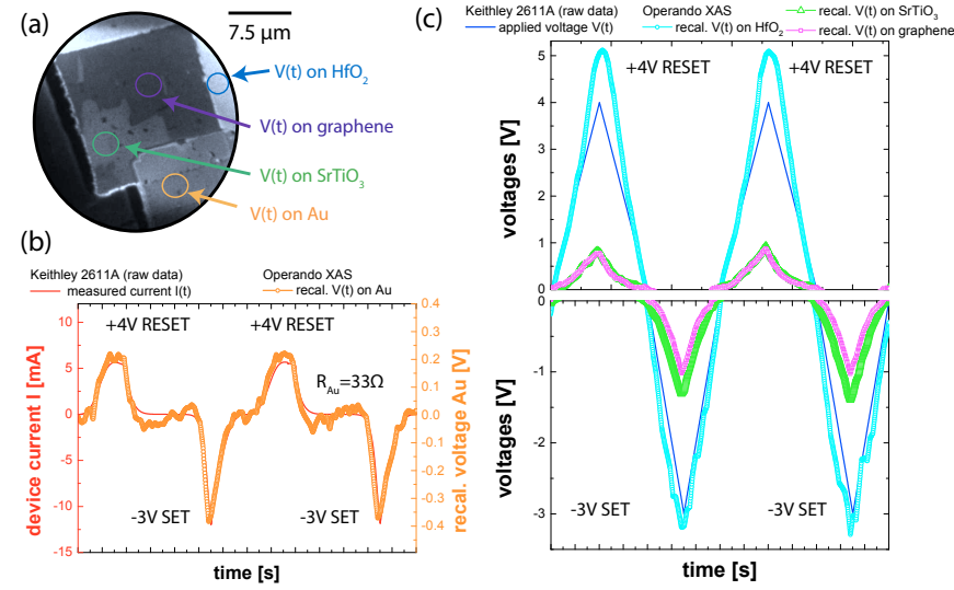
Figure 8.20. – (a) XPEEM image of device in 'fixed potential' mode. Voltage trace extraction points are indicated by color. (b) Local potential V_{Au}(t) at Au lead plotted vs. device current I(t) measured by the Keithley. (c) Potential traces of marked regions plotted vs. externally applied voltage V(t) .
