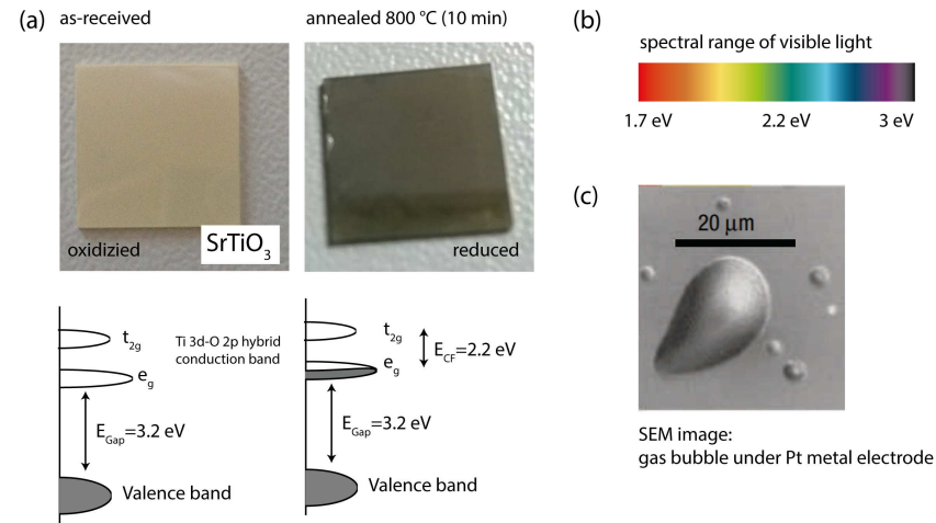
Figure 2.5. – Creation of oxygen vacancies: (a) \text{SrTiO}_3 single crystal as received (left) and after annealing to 800°C under UHV conditions for 10 min (right). The change in color from pearl white to brown indicates the formation of oxygen vacancies at the surface. The partial filling of the CB opens new absorption channels within the visible spectrum. (b) spectral range of visible light (c) SEM image: bubble formation underneath metal electrodes induced by vacancy formation and corresponding oxygen exorporation. See Ref. [24].
