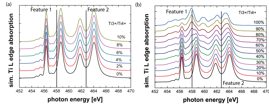
Figure 3.5. – Superpositions of Ti L-edge spectra for \text{Ti}^{4+} and \text{Ti}^{3+} in octahedral configuration ( \Delta_0 = 2.2 eV) for a varying \text{Ti}^{3+} fraction (a) 0 – 10 % \text{Ti}^{3+} in 2 % steps and (b) 0 – 100 % \text{Ti}^{3+} in 10 % steps
