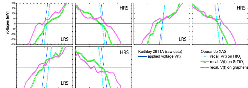
Figure 8.21. – Zoom of zero-voltage crossing points for different resistance states. Neither the potential traces of the graphene nor the potential traces of the SrTiO 3 region show reversible offset modifications.
