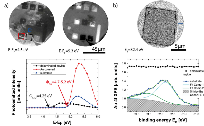
Figure 1.1. – Verification of the delamination process by PEEM & XPEEM (a) PEEM images at two different kinetic energies showing a set of nine devices. Devices with potentially removed Au electrode show a lower work function (black) than devices with remaining Au on top (red). (b) Au 4f 7/2 XPS of a delaminated device: The central pad region is gold free.
