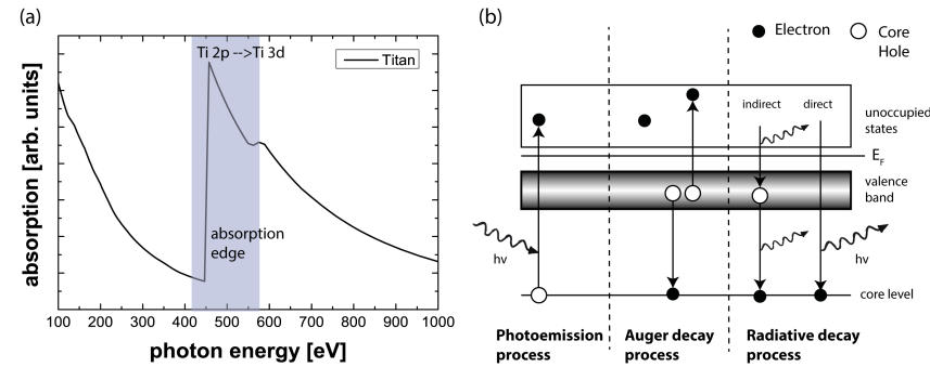
Figure 4.5. – (a) Calculated photon absorption coefficient \sigma(h\nu) for elemental Ti plotted (source: Center for X-Ray Optics). The absorption edge around 458 eV corresponds to the transition from a Ti 2p core level into an unoccupied Ti 3d state. (b) Photoexcitation and core hole relaxation processes: (left) If the photon energy h\nu matches the binding energy E_B , the photon is absorbed and the core level electron is emitted in the unoccupied states. (center) Auger processes: Electrons from lower binding energy can relax into the hole and transfer the excess energy to adjacent electrons. (right) Radiative decays: Electrons can relax into the core hole under the emission of photons.
