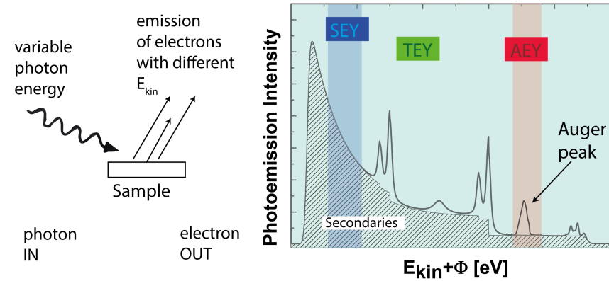
Figure 4.6. – XAS modes defined by the photoelectrons being detected. Total electron yield (green, TEY): the full spectrum of electron kinetic energies is taken into account. Secondary electron yield (blue, SEY): Only electrons near the work function cut-off are considered for analysis. Auger electron yield (AEY): only specific auger electrons are analyzed.
