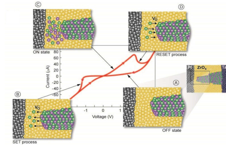
Figure 2.9. – Compact model for VCM in resistive switching in oxides. A complete OFF/ON/OFF cycle for a Pt/ZrO x /Ta MIM device is plotted on the left (A to D). Black balls represent atoms of the electrode; yellow balls are insulating regions in the oxide. Green balls depict oxygen vacancies and purple balls describe valence changed metal atoms. The center graph shows a simulated I-V curve based on the VCM model. Adopted from [31]
