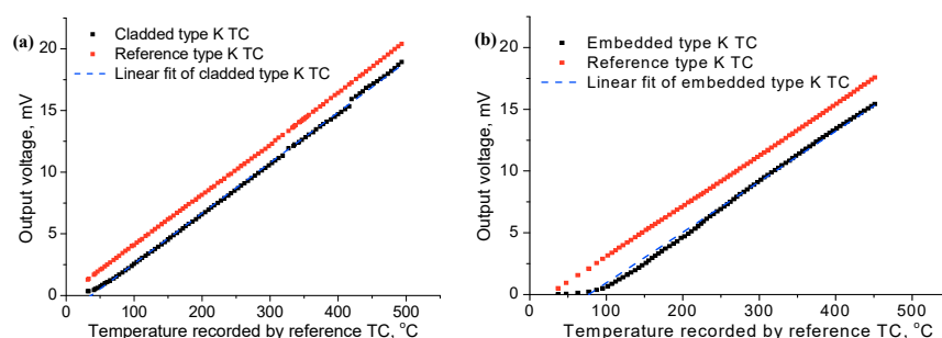
Figure 9. Voltage response of cladded K-type thermocouple from ambient temperature to 450 °C (a) before and (b) after embedding.
