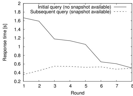
Figure 3. Querying measurements storage: In each round aggregated entity for decreasing timestamp is requested twice.
