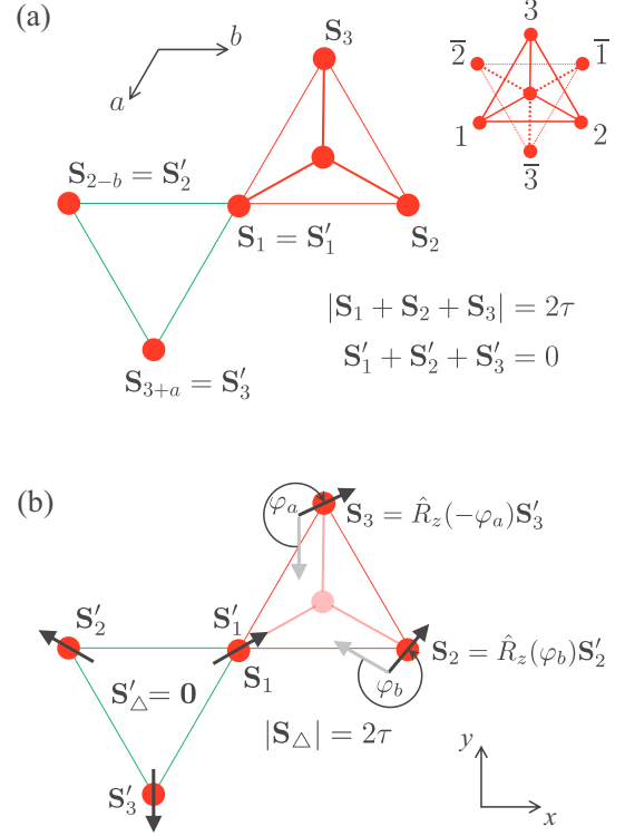
FIG. 9. (a) The spins \mathbf{S}_1 , \mathbf{S}_2 , and \mathbf{S}_3 in the bipyramid triangle ( |\mathbf{S}_1 + \mathbf{S}_2 + \mathbf{S}_3| = 2\tau ) and the spins in the bipyramidal triangles, \mathbf{S}'_1 = \mathbf{S}_1 , \mathbf{S}'_2 = \mathbf{S}_{2-b} , and \mathbf{S}'_3 = \mathbf{S}_{3+a} , forming the 120^\circ state ( \mathbf{S}'_1 + \mathbf{S}'_2 + \mathbf{S}'_3 = 0 ). (b) In the spiral ground states spins \mathbf{S}_2 and \mathbf{S}_3 are obtained by rotating the spins \mathbf{S}'_2 and \mathbf{S}'_3 through the angles \varphi_b and -\varphi_a , respectively.
