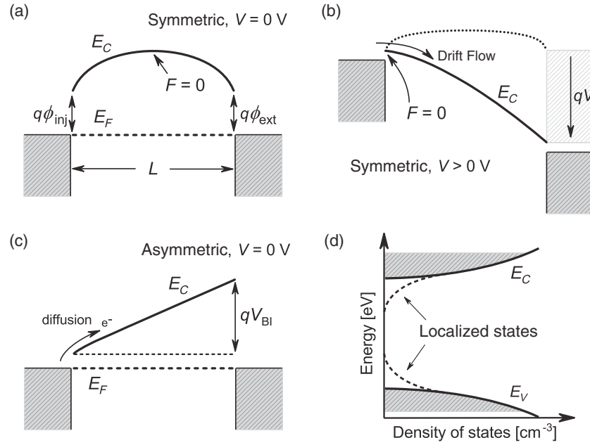
FIG. 1. Schematic of the energy-level diagrams of (a) symmetric electron-only device at thermodynamic equilibrium, where q\phi_{\text{inj}} and q\phi_{\text{ext}} represent the injection and extraction barrier heights, respectively, E_C and E_V are the conduction- and valence-band edge, respectively, E_F is the Fermi level of the semiconductor at thermal equilibrium, and F is the electric field. (b) Symmetric electron-only device with enough applied voltage to assume drift-dominant transport (Mott-Gurney regime). (c) Asymmetric electron-only device at equilibrium showing the energy barrier arising from a built-in voltage qV_{\text{bi}} = q\phi_{\text{ext}} - q\phi_{\text{inj}} . (d) Sketch of the total DOS including exponential tail states (the depth of the tails are given by their respective characteristic energies). Electron transport is shown for simplicity (hole transport is completely analogous). In (b) and (c), forward injection of electrons from the left-hand side is assumed.
