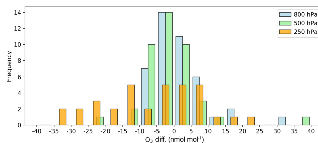
Figure 6. Frequency distributions of the ozone bias (in \text{nmol nmol}^{-1} ) at the 42 stations from Tilmes et al. (2012). Note: high northern latitude stations with biases larger than \pm 40 \text{ nmol nmol}^{-1} at 250 hPa are not shown.
