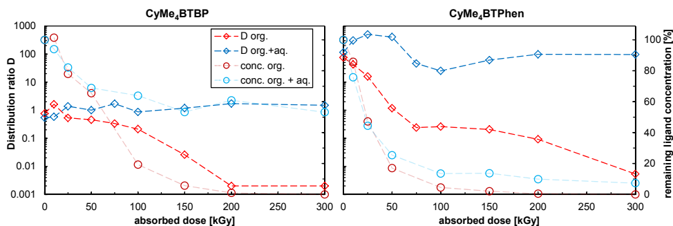
Fig. 45: Americium distribution ratios (left y-axis) for the extraction with irradiated solvents of \text{CyMe}_4\text{BTBP} (left diagram) and \text{CyMe}_4\text{BTPhen} (right diagram) and remaining ligand concentration (right y-axis) as a function of the absorbed dose.
