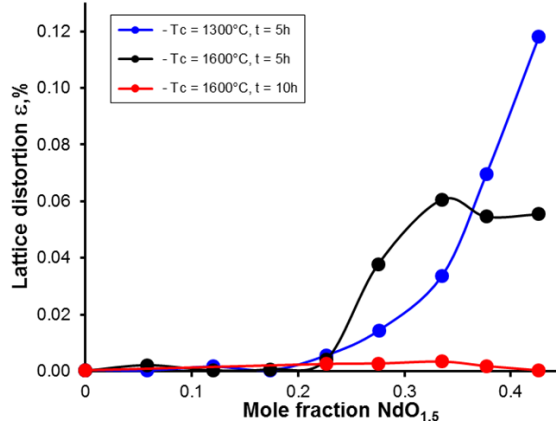
Fig. 47: Lattice distortion ( \delta ) as function of the Nd mole fraction in \text{UO}_2 matrix.
