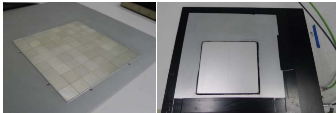
Fig. 79: Assembling of the single bundles on the aluminium frame (left) and mounting on the \alpha -Si flat panel (right).
