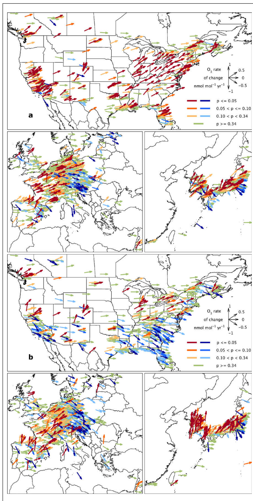
Figure 14: 2000–2014 trends of regional daytime average ozone ( \text{nmol mol}^{-1} \text{yr}^{-1} ). Regional trends (2000–2014) of daytime average ozone ( \text{nmol mol}^{-1} \text{yr}^{-1} ) at all available non-urban sites for December–January–February (DJF, a ), March–April–May (MAM, b ). Vector colors indicate the p-value on the linear trend for each site: blues indicate negative trends, oranges indicate positive trends and green indicates weak or no trend; lower p-values have greater color saturation. DOI: https://doi.org/10.1525/elementa.291.f14
