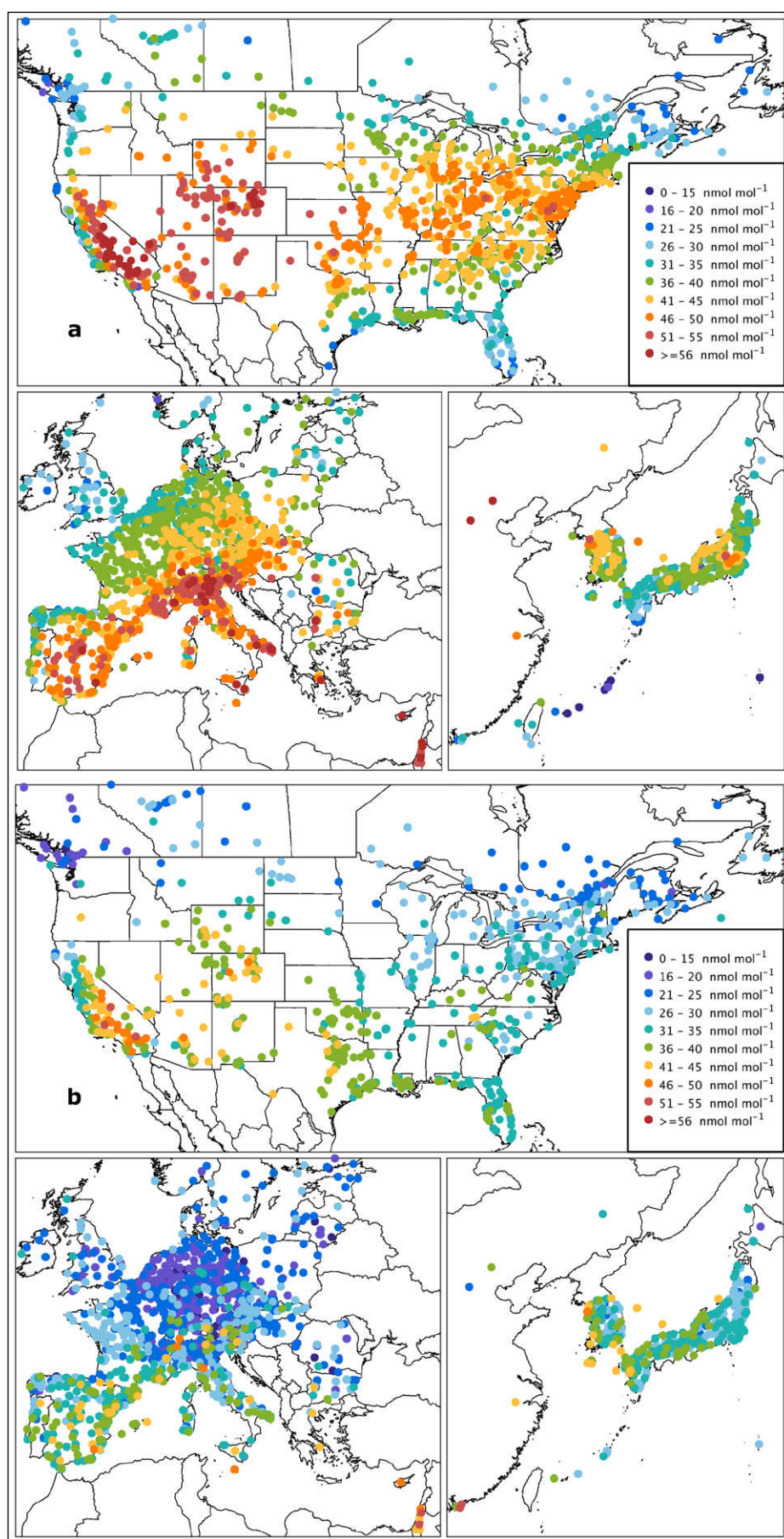
Figure 3: Present-day regional daytime average ozone ( \text{nmol mol}^{-1} ). As Figure 2 but for June–July–August (JJA, a ) and September–October–November (SON, b ). DOI: https://doi.org/10.1525/elementa.291.f3
