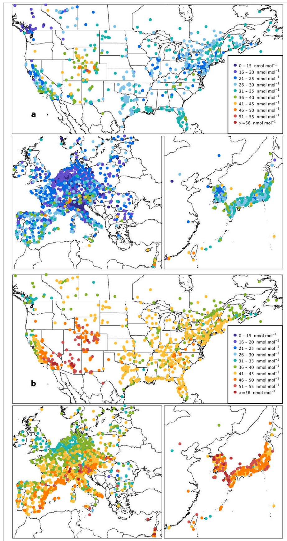
Figure 2: Present-day regional daytime average ozone ( \text{nmol mol}^{-1} ). Regional daytime average ozone ( \text{nmol mol}^{-1} ) at all available non-urban surface sites for December–January–February (DJF, a ), March–April–May (MAM, b ) for the present-day period, 2010–2014. Panel (a) shows the same data as Figure 1 (top), but focuses on the three regions with dense surface networks. DOI: https://doi.org/10.1525/elementa.291.f2
