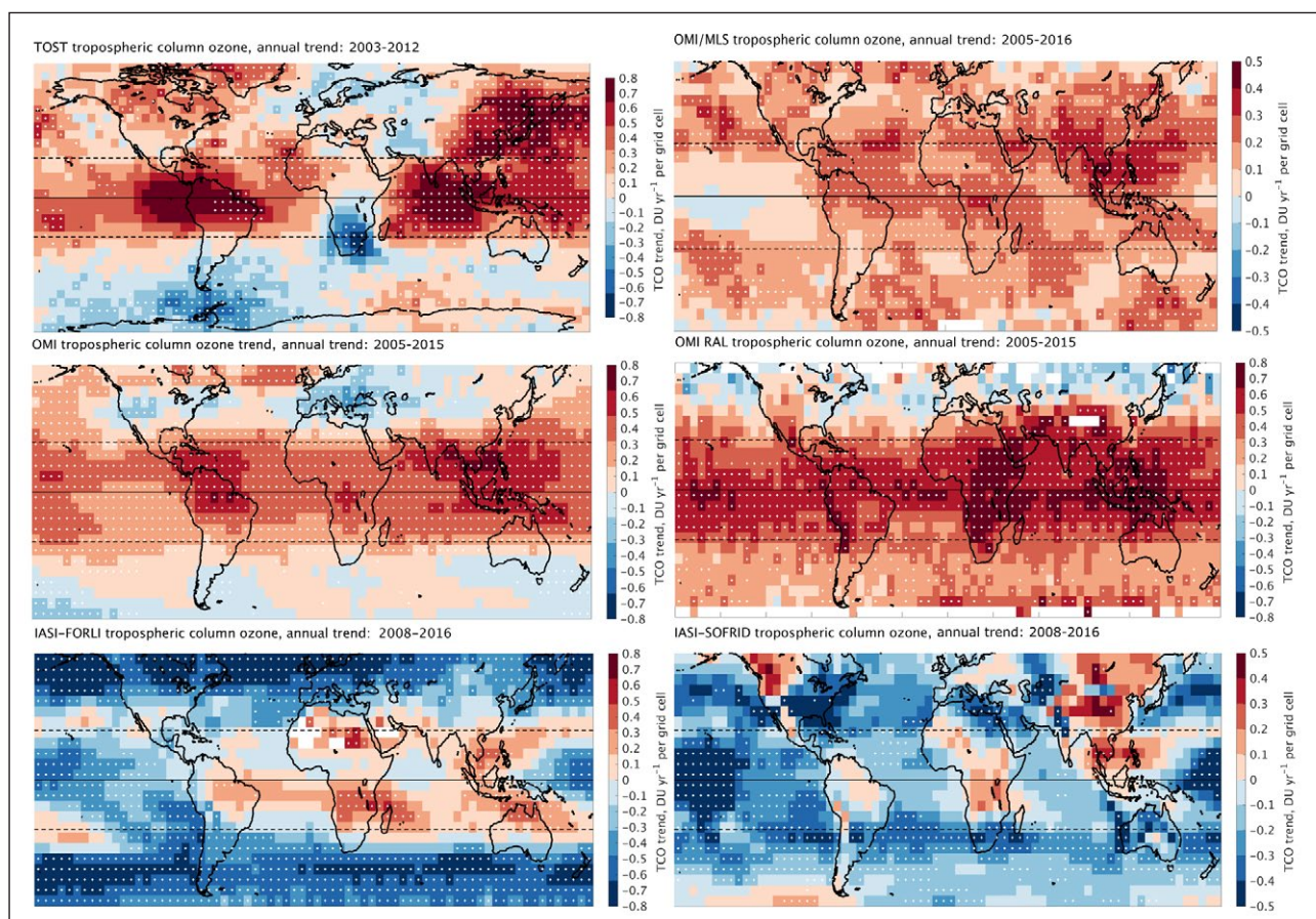
Figure 24: Maps of trends of TCO ( \text{DU yr}^{-1} ) from five satellite products and ozonesondes (TOST). (top left) 2003–2012 TOST ozonesonde annual tropospheric column ozone (TCO) trends in Dobson unit per year ( \text{DU yr}^{-1} ) for each 5° × 5° grid cell between 80°S–80°N. White dots indicate grid cells with statistically significant trends. Also shown are satellite products between 60°S–60°N: (top right) OMI/MLS, 2005–2016, (middle left) OMI-SAO, 2005–2016, (middle right) OMI-RAL, 2005–2015, (bottom left) IASI-FORLI, 2008–2016, and (bottom right) IASI-SOFRID, 2008–2015. Note that OMI/MLS and IASI-SOFRID have different color scales from the rest. Trends in this figure are based on least-squares linear regression and reported with 95% confidence intervals and p-values. DOI: https://doi.org/10.1525/elementa.291.f24
