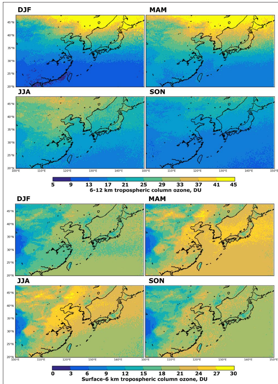
Figure 7: Seasonal mean partial ozone columns (DU) above East Asia from the IASI-LISA product for 2010–2014. Seasonal 6–12 km (top) and surface–6 km (bottom) partial ozone columns (DU) over East Asia, according to the IASI-LISA (TP) product for 2010–2014. The unit is in DU to be comparable with the other satellite products. DOI: https://doi.org/10.1525/elementa.291.f7
