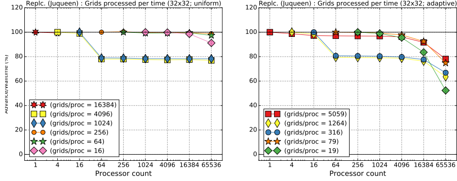
Figure 2. Weak scaling results for the replicated scalar transport problem. Uniformly refined run shown on the left, adaptive run on the right. Each plot shows the efficiency (%) of the particular run, which is computed as the ratio of the number of grids updated per wall time for a simulation run on P processes to the number of grids updated per time on 1 process. The reduction in efficiency going from 16 to 64 processes results from running 1 MPI process per core on 1, 4, and 16 cores to 2 processes per core for 64 and higher process counts, e.g. 32 ranks per node on each JUQUEEN node.
