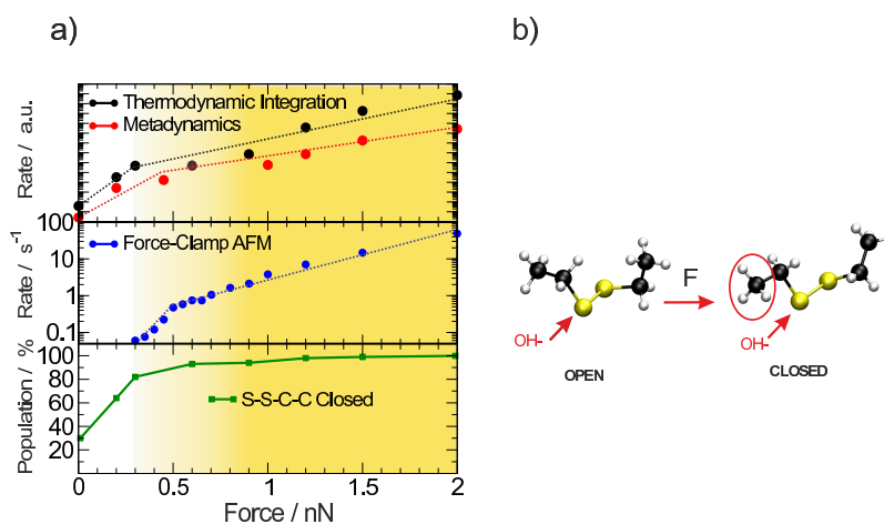
Figure 2. a) Top panel: Force-dependence of the reaction rates obtained from the computed activation free energies ( \Delta A^\ddagger(F) ) via k(F) \sim \exp[-\Delta A^\ddagger(F)/k_B T] , plotted on a logarithmic scale using arbitrary units; Middle panel: reaction rates from force-clamp AFM experiments on a logarithmic scale (data extracted from Figure 2c of Ref. 9; Bottom panel: Relative populations of the closed conformer of the disulphide molecule in the reactant state as a function of force (determined by computing the normalised number of configurations where the S-S-C-C dihedral angles are in the range (180 \pm 50)^\circ ). b) Force-induced transition from the open (left) to the closed (right) diethyl disulphide conformer and the resulting shielding effect with respect to a collinear approach of the nucleophile, OH - , relative to the S-S bond; note that all surrounding water molecules have been omitted for clarity.
