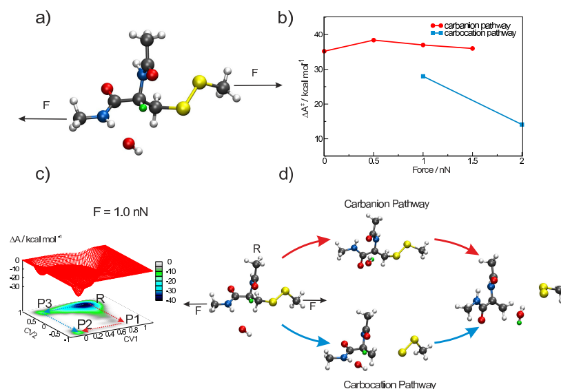
Figure 4. a : Model system to study the \beta -elimination pathway. b : Force-dependence of the activation free energy for \beta -elimination of the disulphide bond corresponding to the rate-determining bimolecular and unimolecular first step of the reaction according to the carbanion (red circles) and carbocation (blue squares) pathways as preferred at low and higher forces, respectively. c : Force-transformed free energy landscape for \beta -elimination at a constant force of F = 1 nN where the carbocation channel is energetically preferred over the still existing carbanion pathway. Red and blue arrows indicate the carbanion and carbocation pathways, respectively, whereas R and Pn, denote reactant and (intermediate) product. d : Representative snapshots sampled from isotensional ab initio metadynamics simulations of the carbocation and carbanion channels at F = 1 nN.
