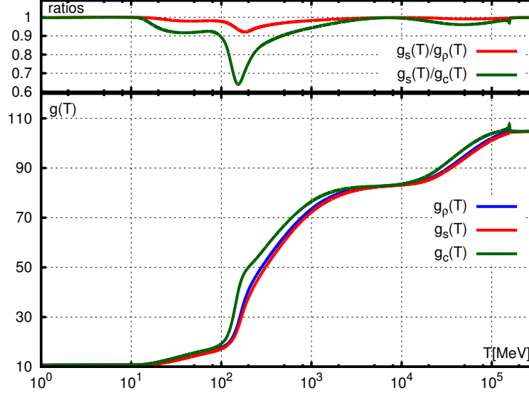
Figure 1. The effective degrees of freedom g_\rho for the energy density ( \rho = g_\rho \frac{\pi^2}{30} T^4 ), g_s for the entropy density ( s = g_s \frac{2\pi^2}{45} T^3 ), and g_c for the heat capacity ( c = g_c \frac{2\pi^2}{15} T^3 ).
