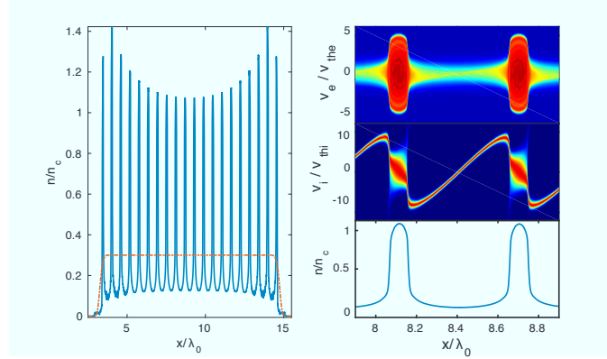
Figure 2. Left: Initial (red line) and final (blue line) plasma density profile of a plasma that has been irradiated by two counterpropagating laser pulses with \lambda_0 = 800 nm and I = 10^{15} W/cm 2 for 300 fs. The final plasma density is periodic with a period of around \lambda_0/2 . Right: Final electron and ion phasespace, showing that the electrons become trapped in the density peaks.
