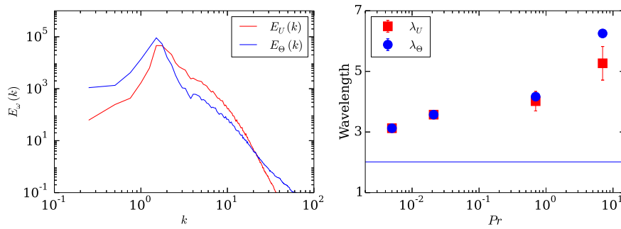
Figure 3. Typical scales of turbulent superstructures obtained by Fourier analysis. Left: time- and azimuthally averaged power spectra E_U(k) and E_\Theta(k) . Data are for Ra = 10^5 and Pr = 0.7 . A corresponding typical wavelength is found from the maximum wavenumber of each of the spectra. Right: Typical wavelengths, \lambda_U and \lambda_\Theta , versus Prandtl number. The Rayleigh number is kept constant at a value of Ra = 10^5 .
