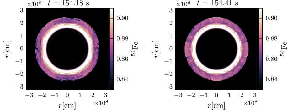
Figure 3. Simulations of the silicon burning phase in a 15 solar mass star in two spatial dimensions with 512^2 cells (left panel) and 3D with 256^3 cells (right panel). The colour coded abundance of ^{54}\text{Fe} is shown in both panels. Regions of fully developed convective burning can be identified in the purple region between 1.9 \times 10^8 cm and 2.6 \times 10^8 cm.
