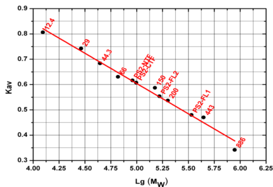
Figure 3.40: M_w determination of PS2 proteins by SEC.
