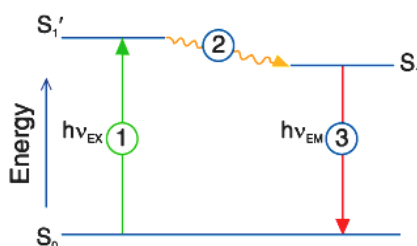
Figure 2.10: Schematic illustration of different electronic transitions.
