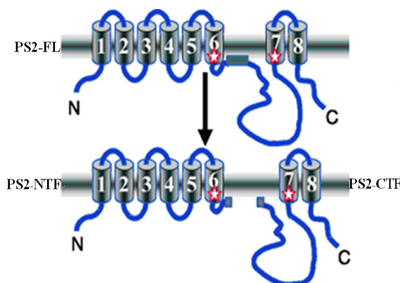
Figure 4.1 Illustration of PS2-FL, PS2-NTF and PS2-CTF.
