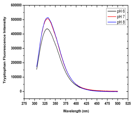
Figure 3.59: Tryptophan fluorescence of His-PS2-NTF-Strep in different pH.
