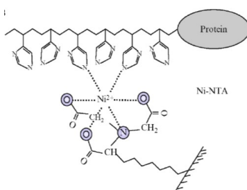
Figure 2.1: A model of interaction between the 6xHis tag and Ni-NTA matrix. Protein in grey with 6xHis tag binding to immobilised Ni-NTA is shown (47).
