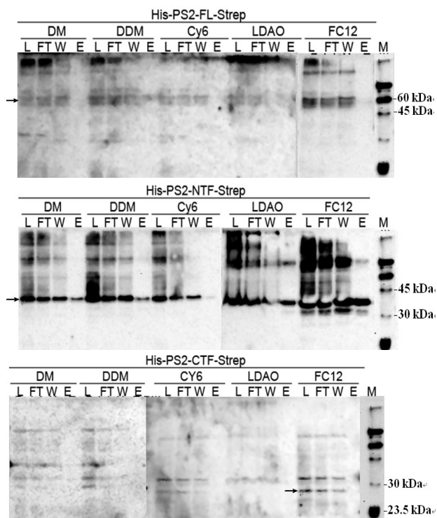
Figure 3.28: Strep-Tactin purification with different detergents.
