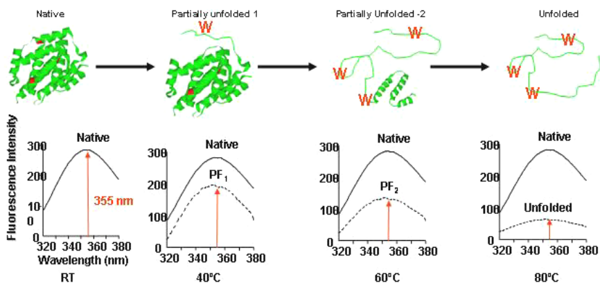
Figure 2.11: Illustration of protein thermal unfolding.
