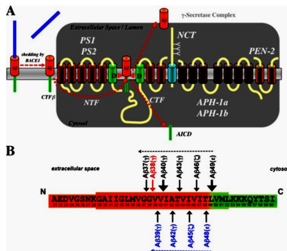
Figure 1.2: Illustration of amyloidogenic pathway of APP processing.
