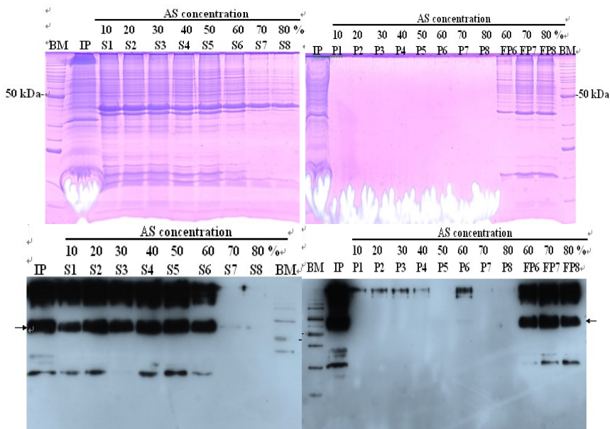
Figure 3.8: Ammonium sulphate precipitation of His-PS2-FL.
