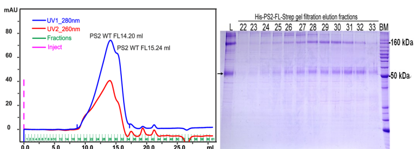
Figure 3.37: SEC analysis of His-PS2-FL-Strep.
