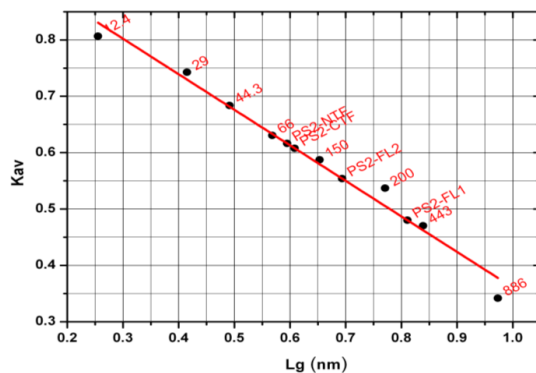
Figure 3.41: R_h determination of PS2 proteins by SEC.
