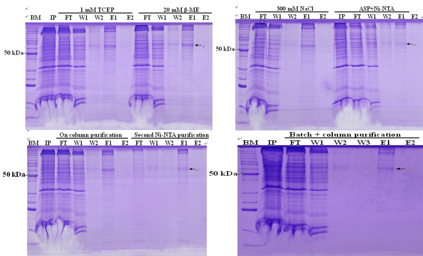
Figure 3.9: Purification Optimization of His-PS2-FL.
