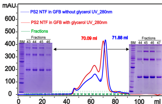
Figure 3.43: Effect of glycerol on SEC of His-PS2-NTF-Strep.
