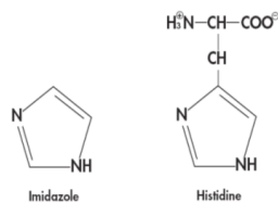
Figure 2.2: Chemical structures of histidine and imidazole.
