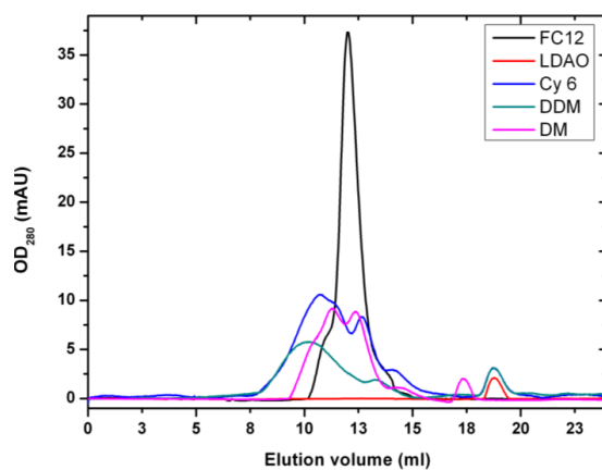
Figure 3.45: SEC profiles of His-PS2-NTF-Strep in different detergents.
