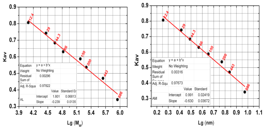
Figure 2.5: Calibration curves of superpose 6 analytical column. Plot of Lg(M_w) versus K_{av} (left) and Lg(nm) versus K_{av} (right).
