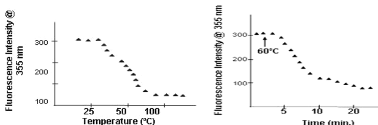
Figure 2.12: Steady and kinetic state protein unfolding.
