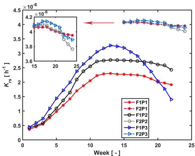
Figure 7. Estimated root hydraulic conductance ( K_{rs} ) in the three plots (P1: sheltered; P2: rainfed; P3: irrigated) of the stony (F1) and silty (F2) soils during the measurement period (F1: from 11 February to 11 July 2014, F2: from 23 May to 24 July 2014).
