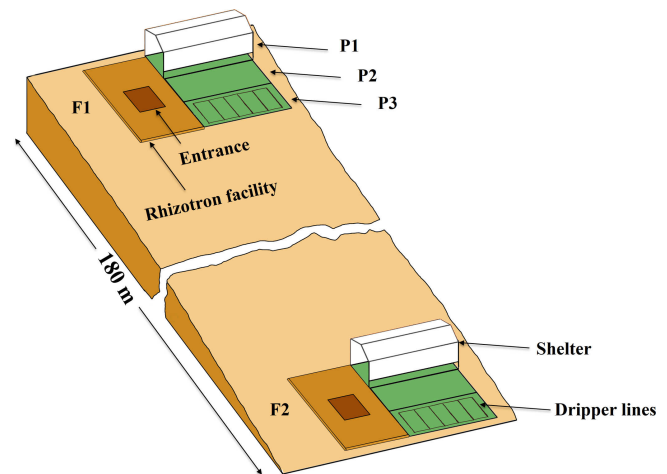
Figure 1. Sketch map of the location and the setup of the upper (F1, stony soil) and lower (F2, silty soil) rhizotron facilities. P1, P2, and P3: the sheltered, rainfed, and irrigated plots.
