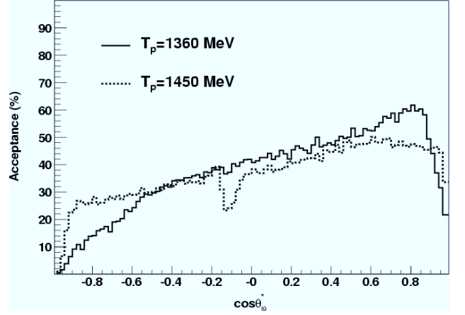
FIG. 3: The acceptance for the pd \rightarrow ^3\text{He}\omega, \omega \rightarrow \pi^+ \pi^- \pi^0 reaction as a function of \cos \theta_{\omega}^* at 1360 MeV (solid line) and 1450 MeV (broken line) after applying the cuts explained in the text. The dip in the 1450 MeV distribution corresponds to the ^3\text{He} that stop between the first and second layer of the FRH.
