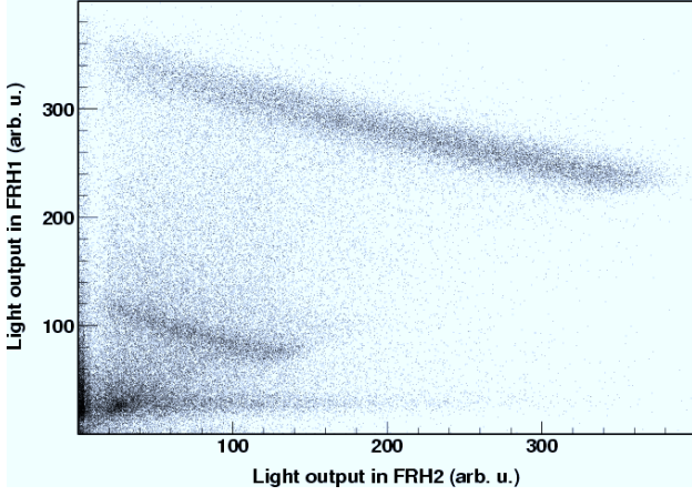
FIG. 2: The scintillation light output in the first layer of the FRH versus the light output in the second layer for particles stopping in the second layer. The uppermost band corresponds to ^3\text{He} ions, below which is a band of stopping protons. The intense spot at the bottom left corresponds to minimum ionizing particles.
