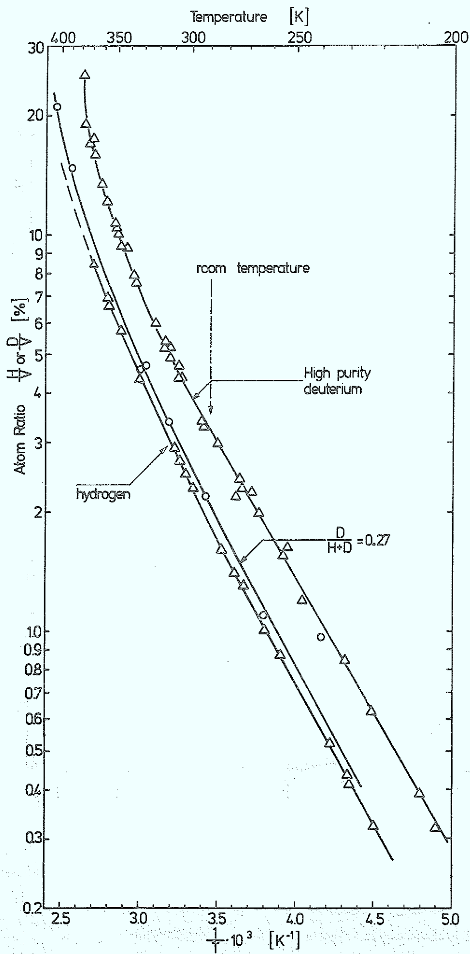
Fig. 39. Solvus for the VH and VD and a mixed system [96]. VH-solvus: \Delta H = 0.1413 \pm 0.005 eV and c_0 = 5.10 \pm 0.50 . VD-solvus: \Delta H = 0.135 \pm 0.004 eV and c_0 = 7.00 \pm 0.70 . These enthalpies are the energies required to transfer one H atom from the ordered to the \alpha phase.
