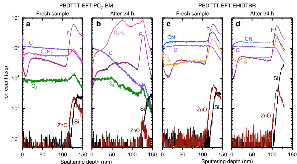
Fig. 5 Depth profiles before and after degradation. Negative SIMS depth profiling of PBDTTT-EFT:PC 71 BM ( a , b ) and PBDTTT-EFT:EHIDTBR ( c , d ) blends prior to light radiation and subjected to light radiation equivalent to 24 h. 0 nm sputtering depth represents the top surface and 150 nm shows the substrate (ZnO)
