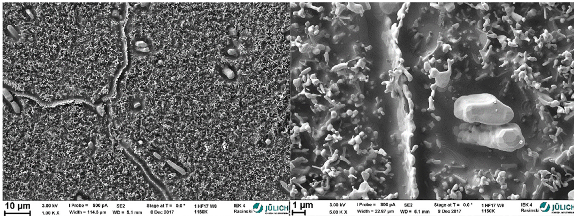
Fig. 6. SEM image of HiperFer-W6 after exposure at 1069 K. As in Fig. 5, Mo–Nb crystallites are visible throughout the surface. W enriched at the grain boundary lines and the fuzzy structures. The fuzzy structures grow coarser at higher temperatures.
