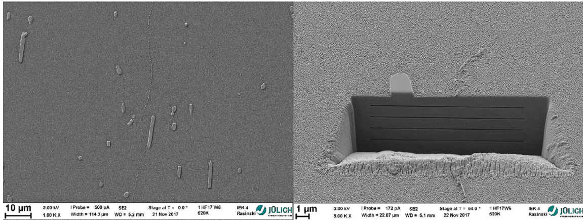
Fig. 5. Electron microscopy images of HiperFer-W6 after PSI-2 exposure at 526 K. The left picture shows the surface with a central grain boundary and several Mo–Nb islands. In total, the islands cover about 0.3% of the surface area. Mo originates from the PSI-2 plasma source. The right image shows a FIB-cut at one of these islands. Furthermore, the surface formed a grass like structure, probably responsible for the reduced sputtering yield. EDX analysis revealed a homogeneous distribution of W over the surface, including the islands.
