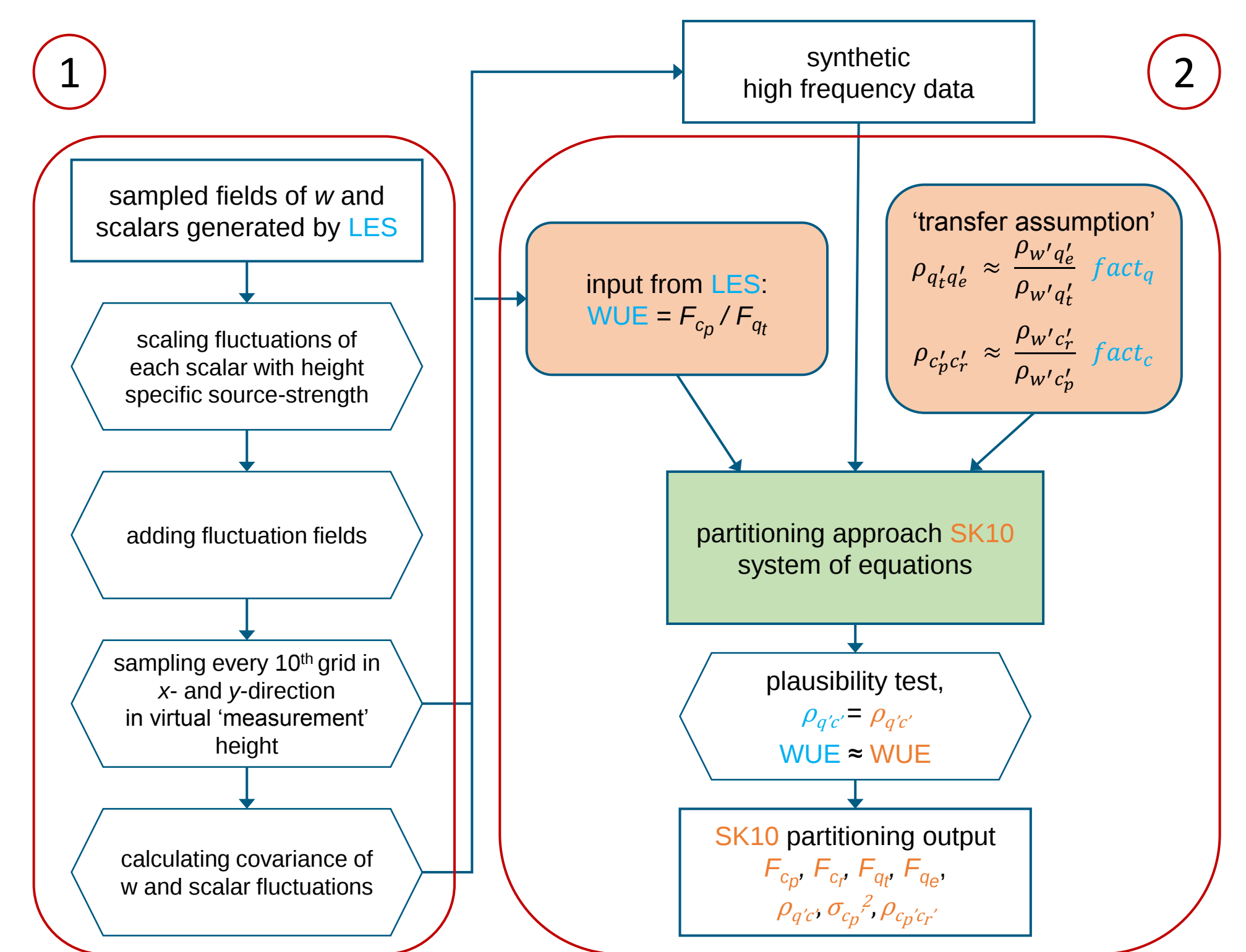
Fig.3: Method: (1) Generation of synthetic high frequency data with LES, (2). application of SK10 to derive the contributions to the fluxes of CO 2 and H 2 O.
