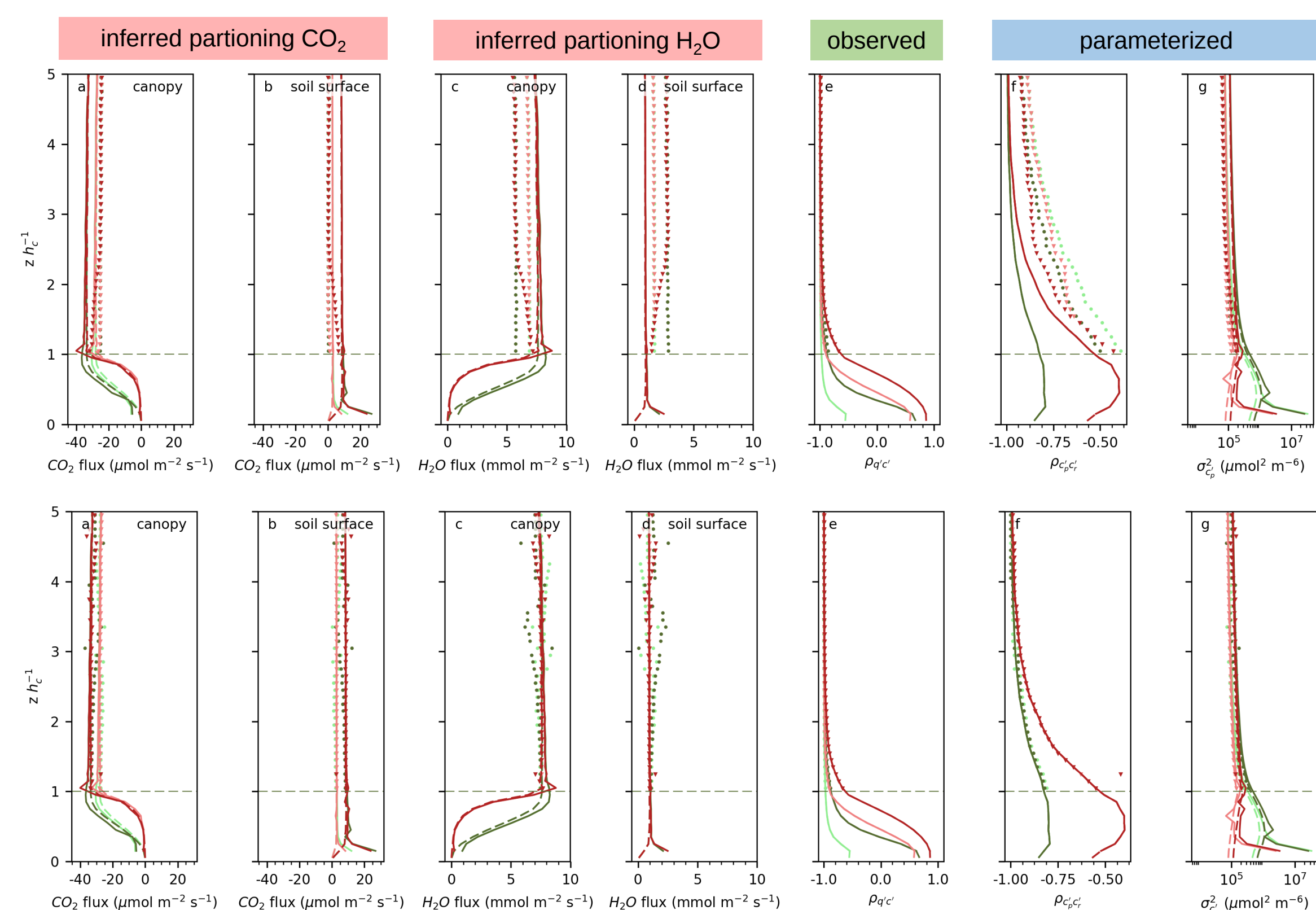
Fig.4: Vertical profiles of inferred H 2 O and CO 2 flux components, observed \rho_{q'c'} and parameterized \rho_{cp'c_r'} and \sigma_{cp}^2 for four sink-source-distributions (ModelV or ModelB, low or high soil source). Top: the partitioning results of SK10 with the original parametrization for \rho_{cp'c_r'} ; bottom: partitioning results with correction to the transfer assumption.
