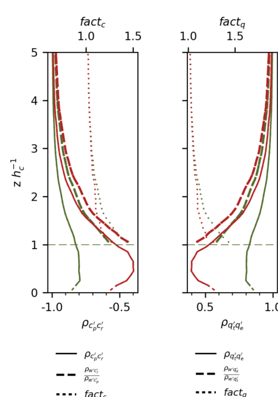
Fig.5: Comparison of real and parameterized correlation coefficients \rho_{cp'c_r'} and \rho_{qt'q_e'} (transfer assumption) and the corresponding correction factors ( fact_q , fact_c ).
