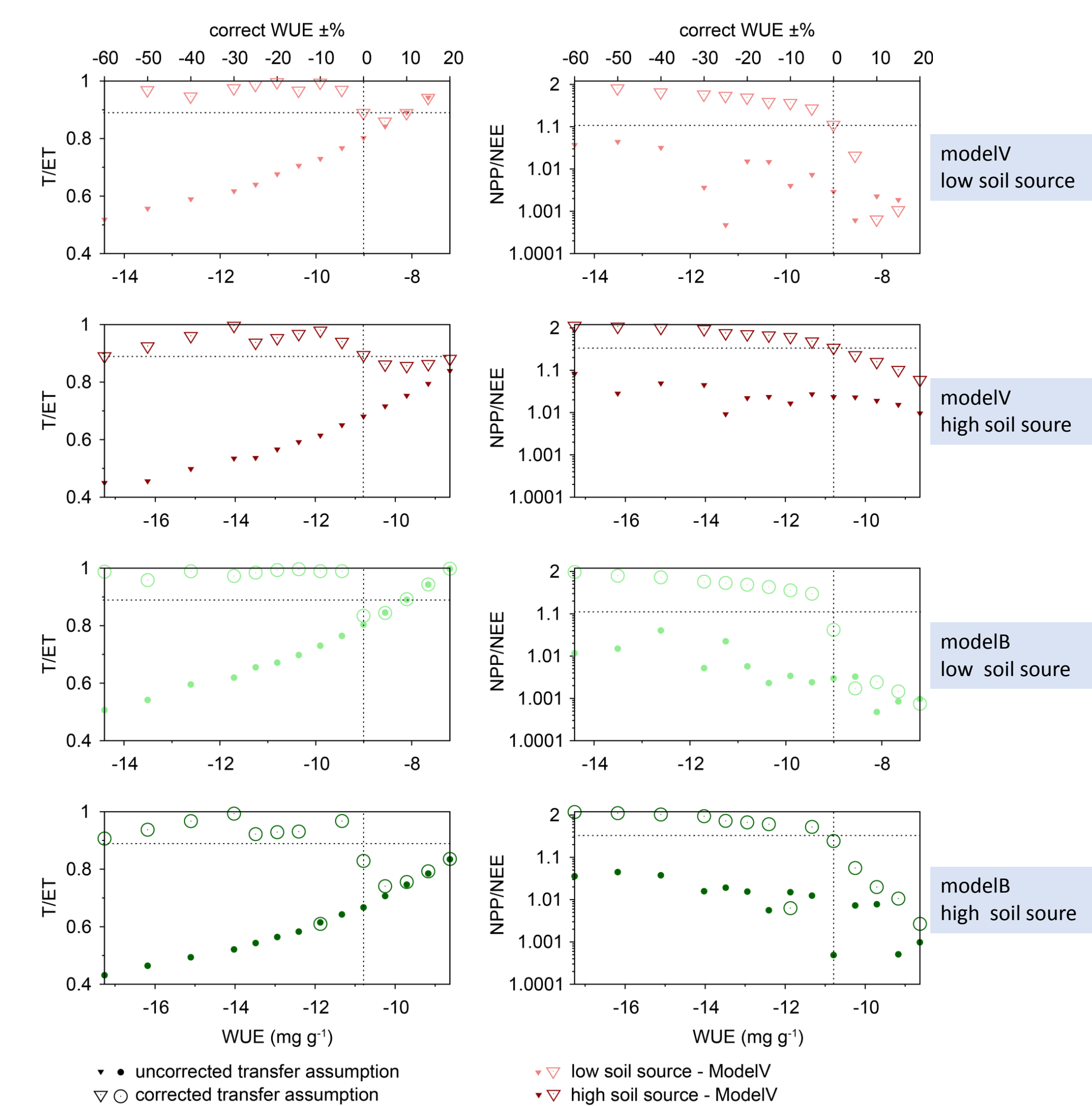
Fig.6: Results of partitioning fractions for H 2 O (T/ET, left ) and CO 2 (NPP/NEE, right ) fluxes in relation to the input WUE at a 'measurement' height of 2.5 h_c with corrected and uncorrected transfer assumption. The true known imposed partitioning factors and WUE input are indicated by the dashed lines (T: transpiration, ET: evapotranspiration, NPP: net primary production, NEE: net ecosystem exchange).
