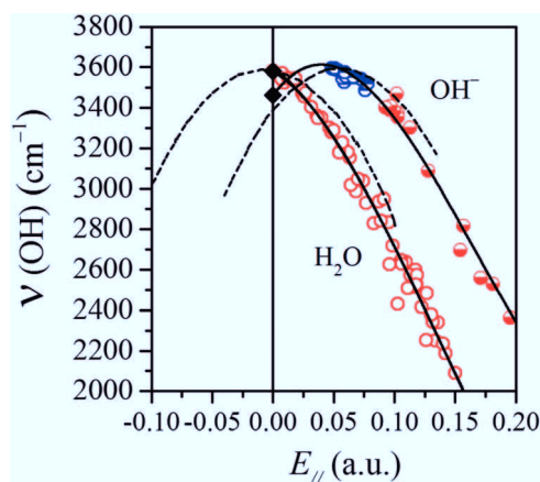
Fig. 3 The same correlations as in Fig. 2(b) and (d) but here the water and hydroxide OH groups are plotted together to highlight that they follow two different ' \nu(\text{OH}) vs. E_\parallel ' correlations. The dashed curves are taken from ref. 10 where the author performed MP2 calculations for a water molecule and a hydroxide ion in uniform electric fields of varying strengths. Here and in the following, the circles for the data points have the same meaning as in Fig. 2.
