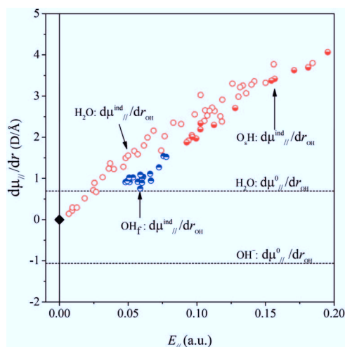
Fig. 6 Calculated permanent and induced dipole moment derivatives with respect to the intramolecular OH distance, calculated for all the \text{OH}_{\text{w}} , \text{O}_2\text{H} and \text{OH}_{\text{f}} groups in our systems, and plotted against E_{\parallel} .
