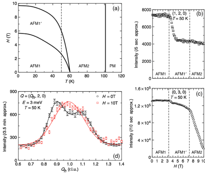
FIG. 4. (a) (T-H) phase diagram of \text{Mn}_5\text{Si}_3 for \vec{H}||c after Ref. [20]. The vertical dashed line indicates the temperature (50 K) where neutron scattering measurements were performed under a magnetic field. (b),(c) Field dependence of magnetic Bragg peaks (1, 2, 0) and (0, 3, 0) at 50 K. For (1, 2, 0) , a 9 mm plexiglass attenuator was in place. (d) Inelastic spectra obtained at 50 K around \mathbf{Q} = (Q_h, 2, 0) under a 0 and 10 T magnetic field for an energy transfer of 3 meV. The red line is a guide for the eyes, and the black line corresponds to fits with Gaussian functions. Data were obtained with an unpolarized neutron beam using IN12.
