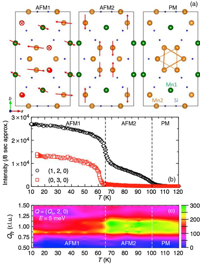
FIG. 1. (a) Projection of the structure of \text{Mn}_5\text{Si}_3 in the (a, b) plane of the orthorhombic cell according to single crystal neutron diffraction data [16,17]. The triangles with continuous and dashed lines are located in different planes separated by c/2 . The red symbols \otimes and \odot in the AFM1 phase indicate magnetic moments pointing in and out of the page, respectively. (b) Temperature dependence of the purely magnetic (1, 2, 0) and (0, 3, 0) Bragg peak intensities. (c) Color-coded intensity plot of the INS data collected at a constant energy transfer of 5 meV as a function of \mathbf{Q} = (Q_h, 2, 0) and temperature. Data were collected with an unpolarized neutron beam using the three-axis spectrometer 2T1. In the inelastic spectra, the background is subtracted and the measured intensity is corrected by the detailed balance factor.
