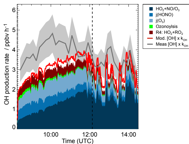
Figure 5. OH budget during the experiment at low NO concentration (23 May 2017) for the period, when MVK photooxidation took place. The vertical dashed line indicates when MVK was reinjected into the chamber. Red and blue coloured areas add contributions to the OH production calculated from the model results (M2 sensitivity run in Fig. 4). The contribution \text{RO}_2 + \text{HO}_2 refers to the OH production from Reaction (R4). In addition to modelled OH production contributions, total OH production calculated from the product of OH concentration and OH reactivity ( k_{\text{OH}} ) is shown. These quantities are either taken from the model results (M2) or from measurements. The coloured grey area gives the uncertainty of the total OH production calculation, if measured OH concentrations and measured OH reactivity are used.
