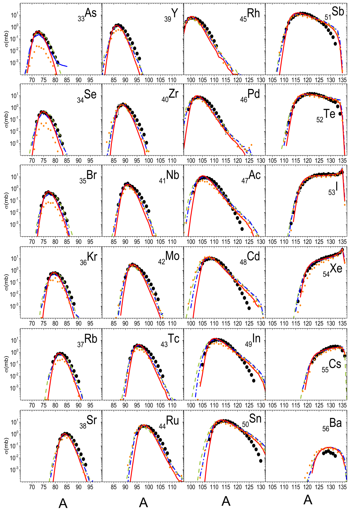
Fig. 3. Same as fig. 1, but for Z = 33\text{--}56 .
