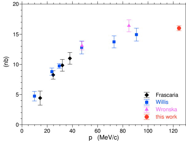
Fig. 10. Excitation function for the total cross section for the dd \rightarrow \alpha \eta reaction. The data are from Frascaria et al. [12], Willis et al. [13], and Wrońska et al. [17]. Only statistical errors are shown.
