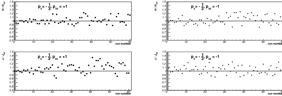
Fig. 8. Comparison of the ratio of the measured parameters H and J to the reference values H_{\text{ref}} and J_{\text{ref}} for both polarisation states as functions of the run number. The H parameter corresponds to the vector polarisation p_z , while J is connected with the tensor beam polarisation p_{zz} . Left: Polarisation state with p_z = -\frac{1}{3} , p_{zz} = +1 . Right: Polarisation state with p_z = -\frac{1}{3} , p_{zz} = -1 .
